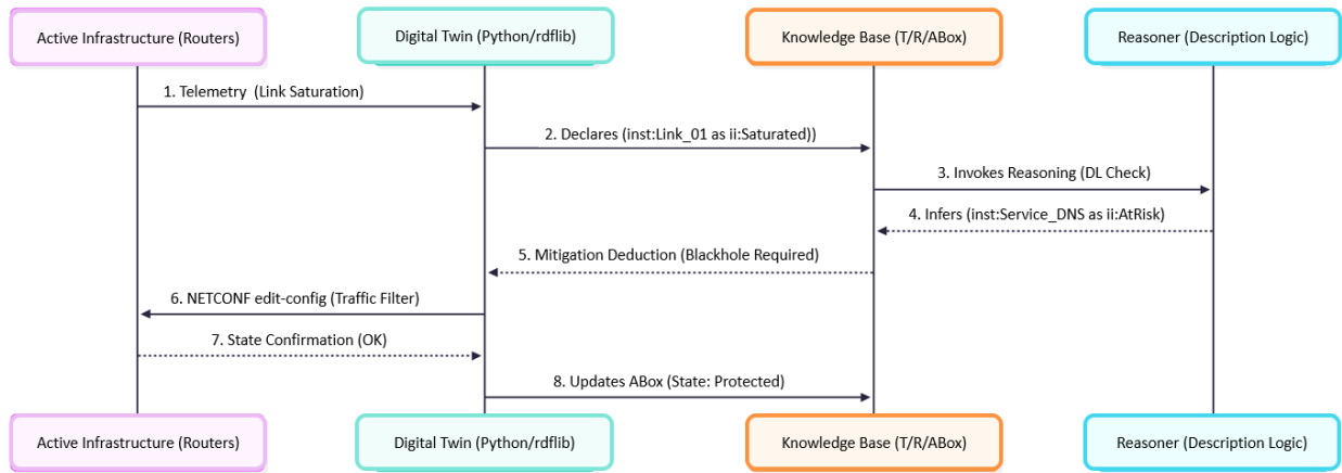
Figure 2: Sequence Diagram of DDoS Mitigation via DT-II
