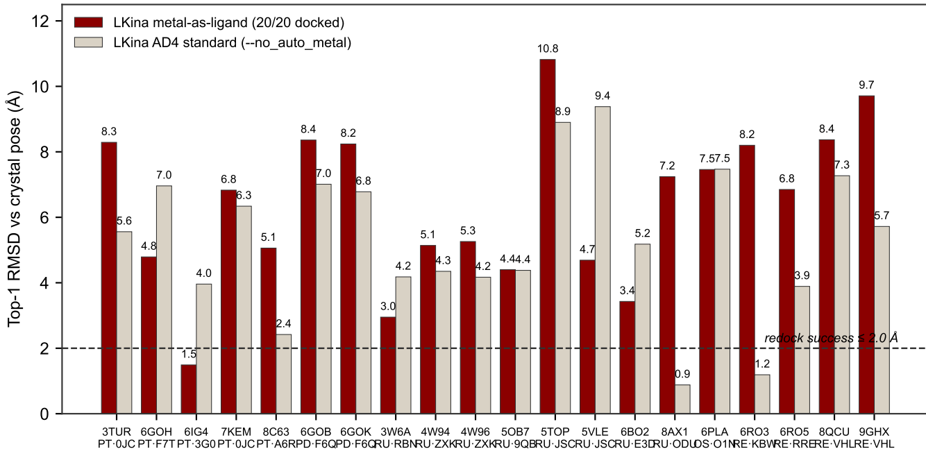
Metal-as-ligand redocking — full Pt/Pd/Ru/Os/Re pool (n=20); Vina 1.2.7 fails 20/20 at parse time
