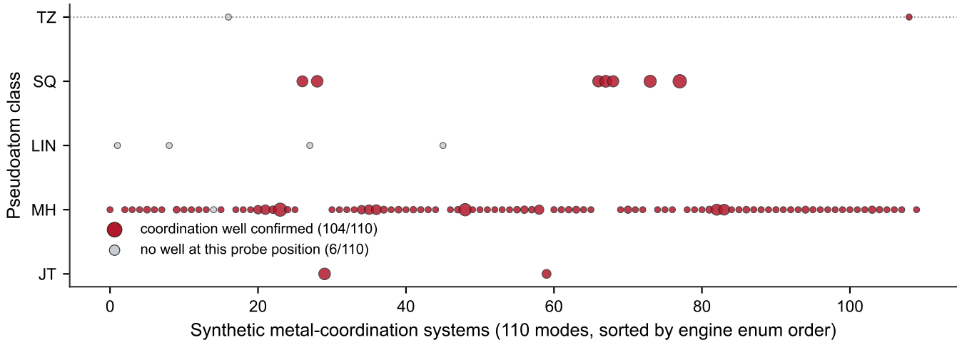
Coordination potential well E_{\text{ideal}} < E_{\text{far}} across the complete mode enum
