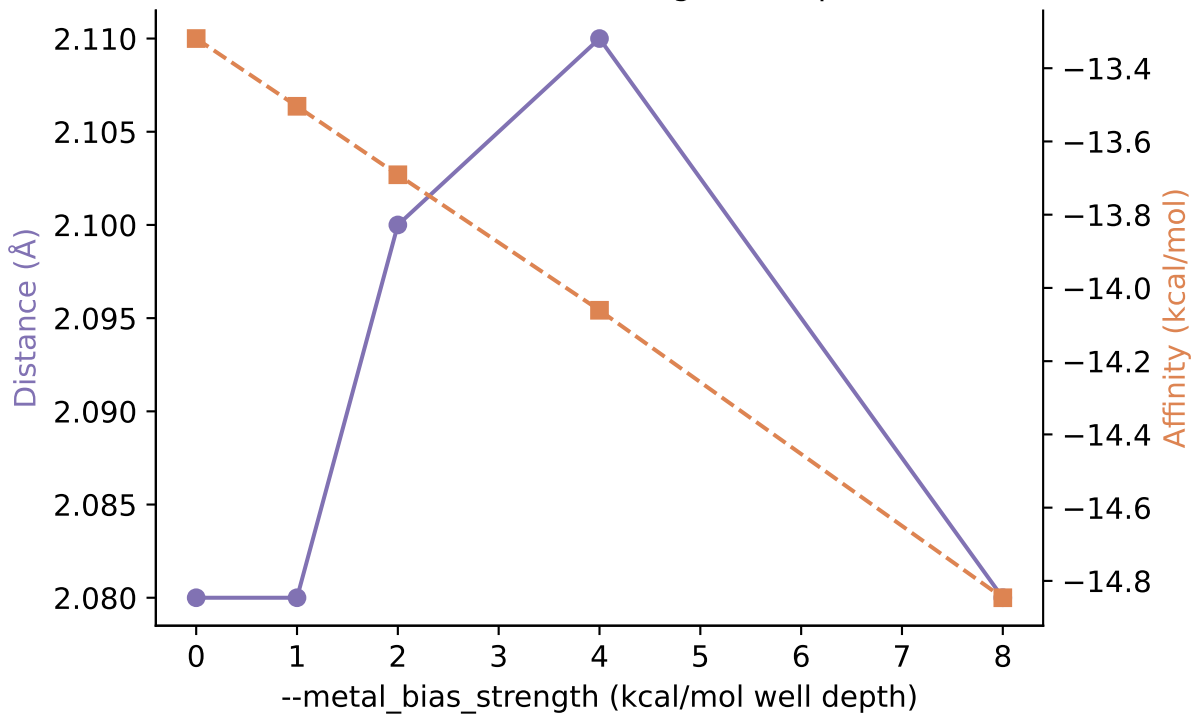
Metal-bias (O5) attractor strength sweep (3HS4, zn)
