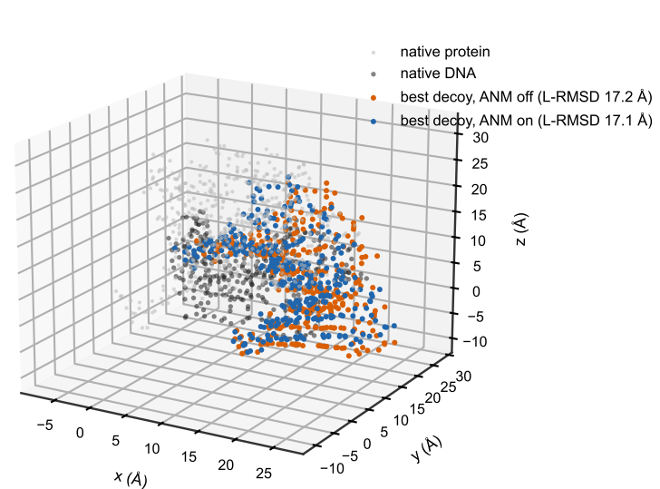
C Best decoy vs bound complex
