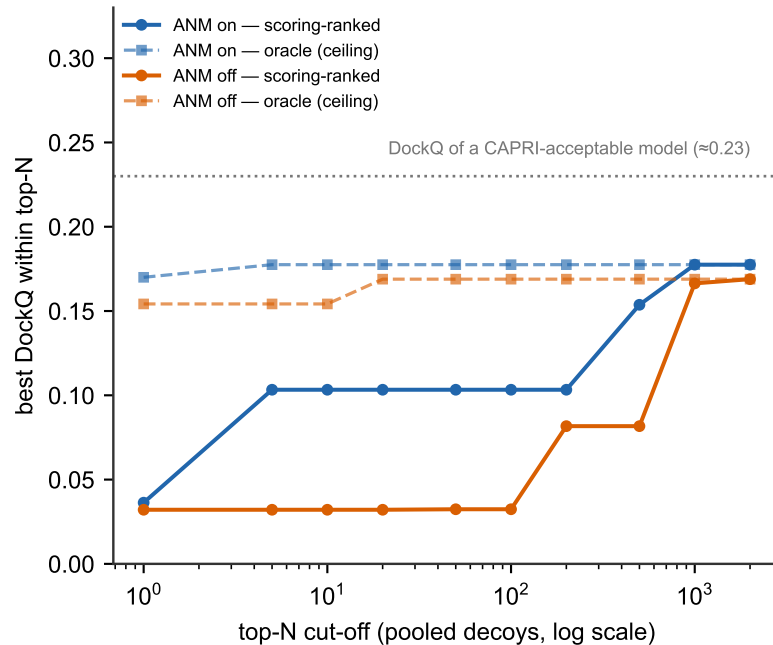
B Ranking vs sampling ceiling
