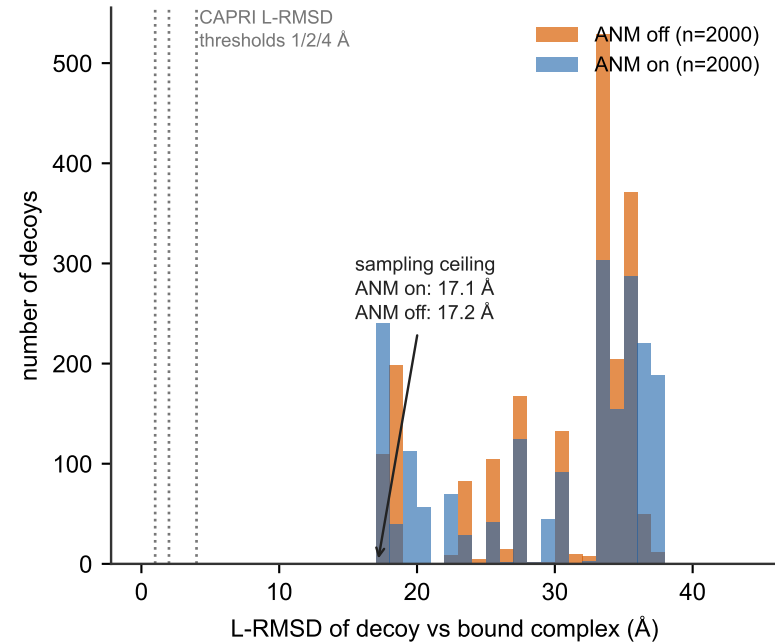
A Protein–DNA decoy quality (1AZP, Sac7d–DNA; 10 swarms \times 200 glowworms \times 200 steps)
