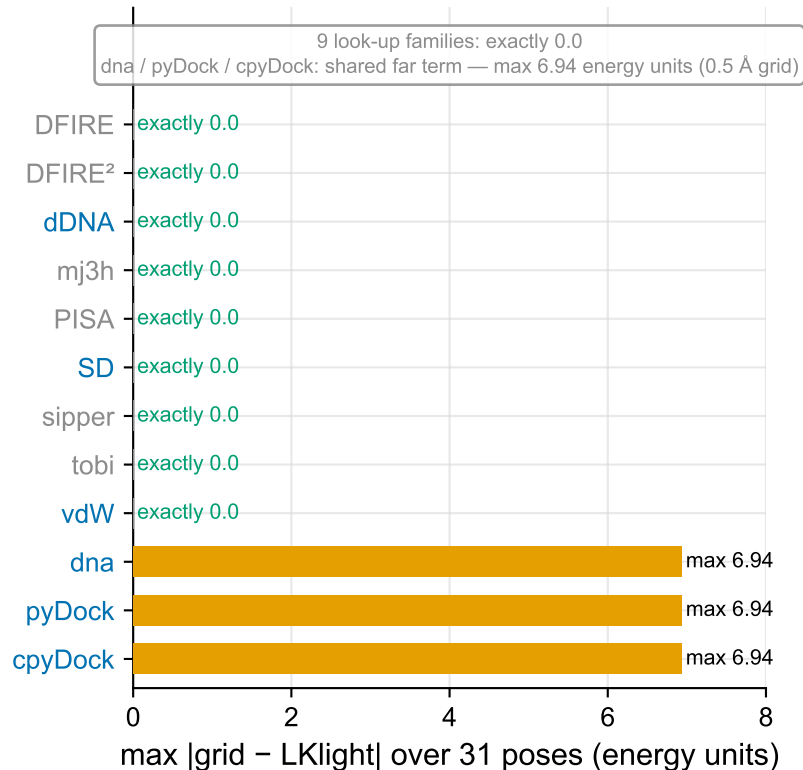
(A) absolute far-field error
