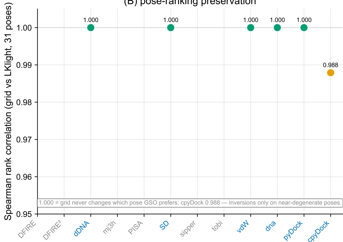
(B) pose-ranking preservation
