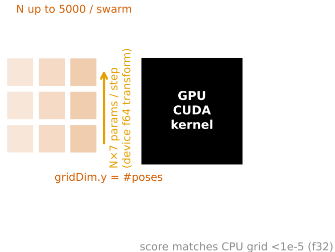
(C) CUDA batch (LKlight-GPU) all poses of one step, one kernel
