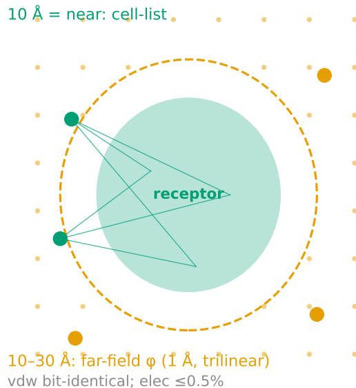
(B) CPU grid (LKlight-grid) cell-list near + far-field lookup
