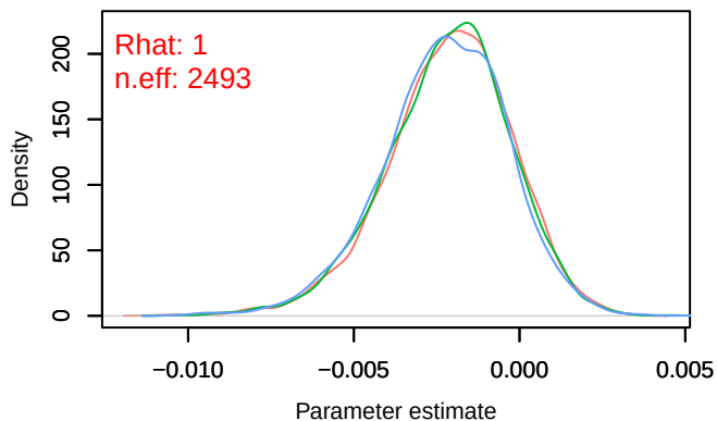
Density – B[altitude (C9), Pica_pica (S3)]
