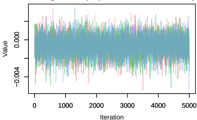
Trace – B[altitude (C9), Carduelis cannabina (S4
