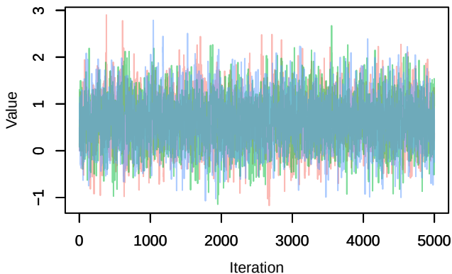
Trace – B[p_milieuE (C7), Carduelis cannabina (S
