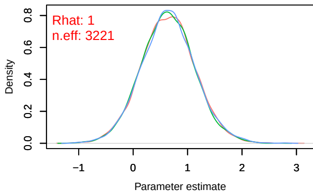
Density – B[p_milieuE (C7), Carduelis cannabina (S
