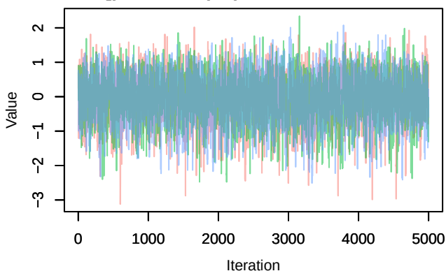
Trace – B[p_milieuF (C8), Carduelis cannabina (S
