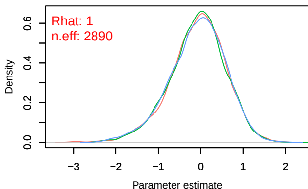
Density – B[p_milieuF (C8), Carduelis cannabina (S
