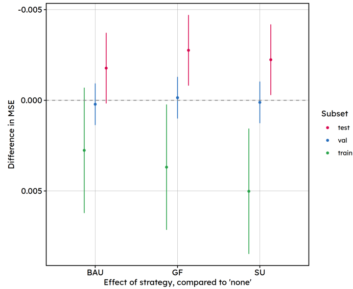
Comparison of scores per subset, k_fold mean + 95% CI. Model type: random=none, strategy: x-value, new samples=50, training size=125, n variables=6.
