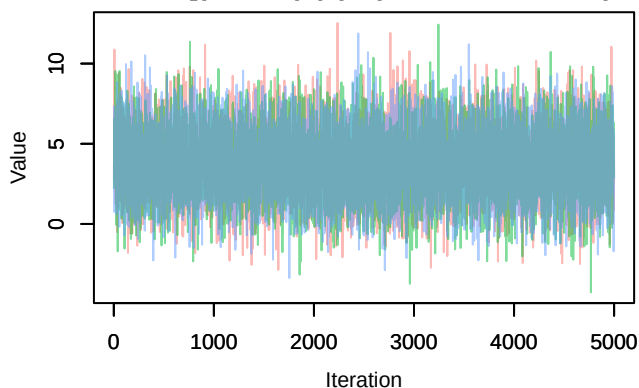
Trace – B[(Intercept) (C1), Turdus merula (S3)]
