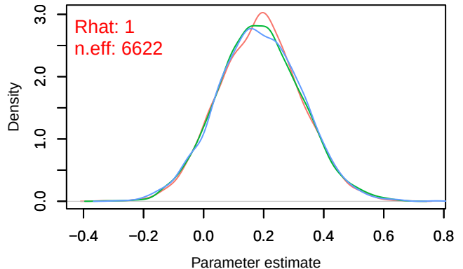
Trace – B[tmp_spring (C11), Carduelis_chloris (S8)]
