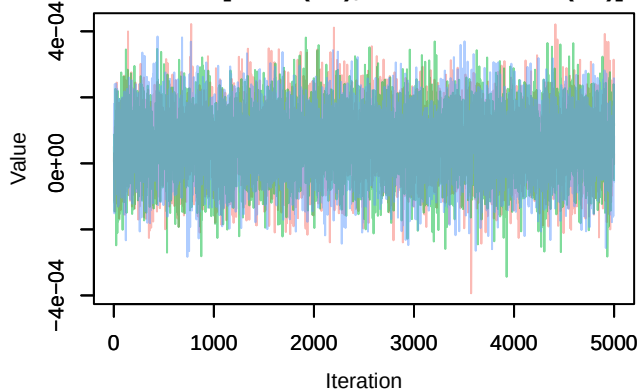
Trace – B[NDVI (C2), Turdus merula (S3)]
