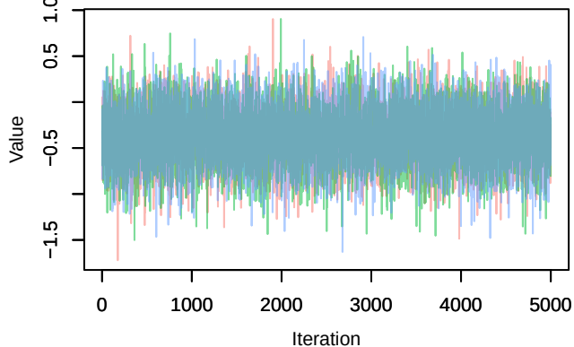
Trace – B[p_milieuB (C4), Parus_major (S4)]
