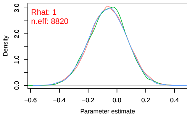
Density – B[tmp_spring (C11), Fringilla coelebs (S2)]
