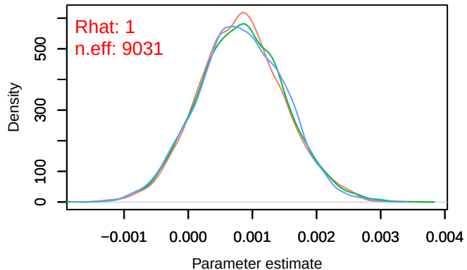
Density – B[altitude (C9), Sylvia atricapilla (S1)]
