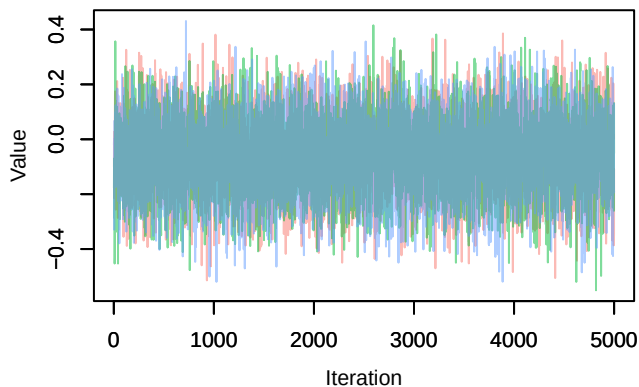
Trace – B[tmp_spring (C11), Fringilla coelebs (S2)]
