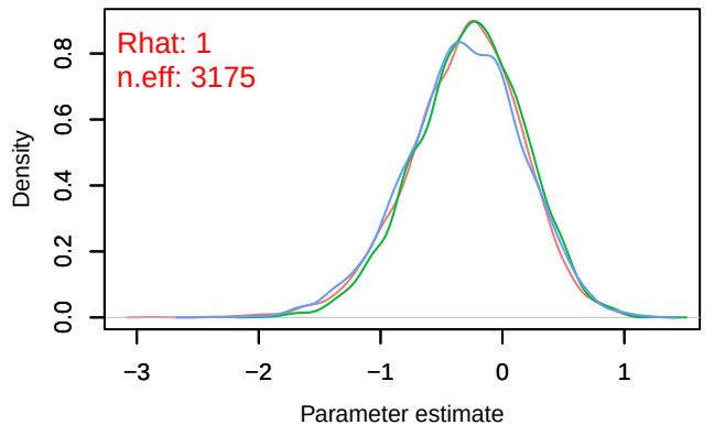
Trace – B[tmp_spring (C11), Sylvia_communis (S1 Density – B[tmp_spring (C11), Sylvia_communis (S
