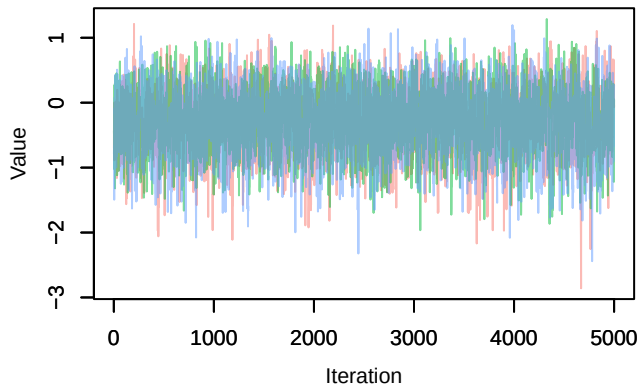
Trace – B[tmp_spring (C11), Sylvia_communis (S1 Density – B[tmp_spring (C11), Sylvia_communis (S
