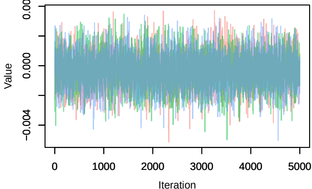
Trace – B[precip_spring (C10), Carduelis_cannabina
