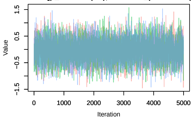
Trace – B[p_milieuB (C4), Columba_palumbus (S5)]
