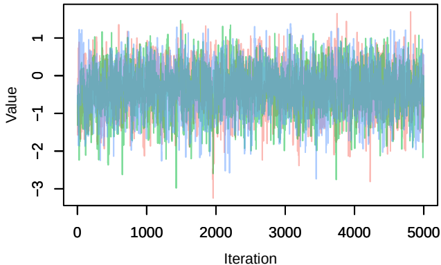
Trace – B[altitude (C9), Carduelis_cannabina (S11
