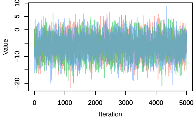
Trace – B[(Intercept) (C1), Carduelis_cannabina (S Density – B[(Intercept) (C1), Carduelis_cannabina (S
