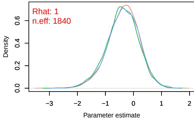
Density – B[altitude (C9), Carduelis_cannabina (S1
