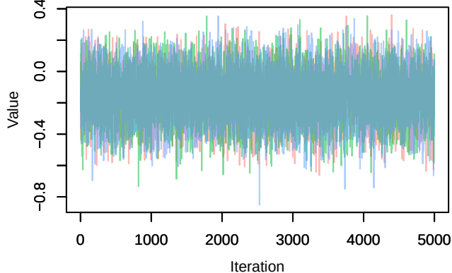
Trace – B[tmp_spring (C11), Columba_palumbus (S6)]
