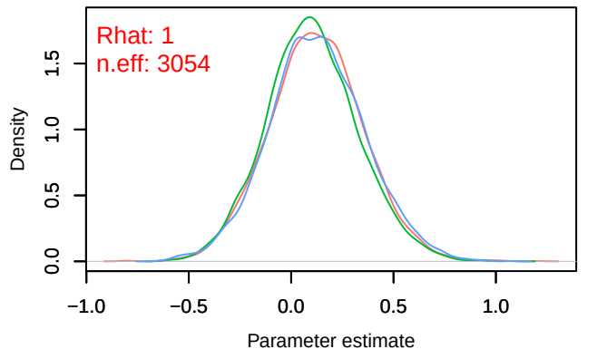
Trace – B[(Intercept) (C1), Carduelis_cannabina (S Density – B[(Intercept) (C1), Carduelis_cannabina (S
