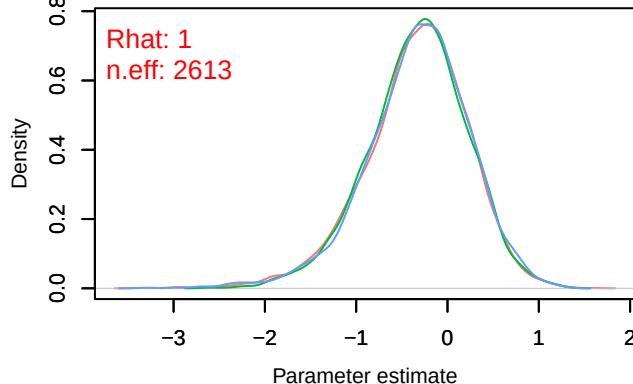
Density – B[p_milieuF (C6), Turdus_viscivorus (S13)
