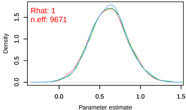
Density – B[p_milieuB (C2), Parus_major (S4)]
