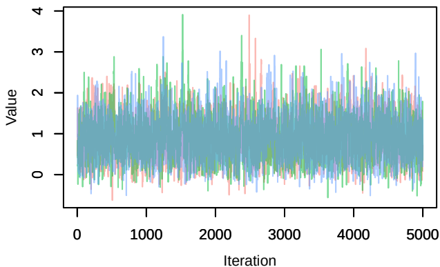
Trace – B[p_milieuE (C5), Phoenicurus_ochruros (S...)
