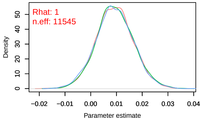
Trace – B[(Intercept) (C1), Dendrocopos_major (S5)] Density – B[(Intercept) (C1), Dendrocopos_major (S5)]
