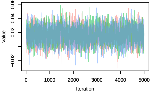
Trace – B[light_pollution (C7), Serinus_serinus (S12)
