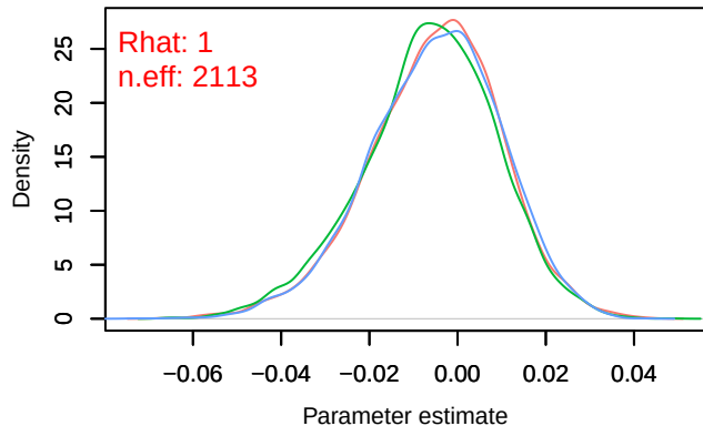
Density – B[light_pollution (C7), Periparus_ater (S15)]
