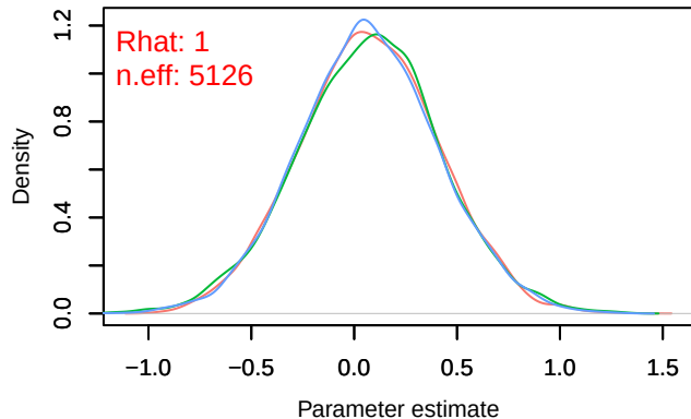
Density – B[p_milieuE (C5), Anthus_trivialis (S14)]
