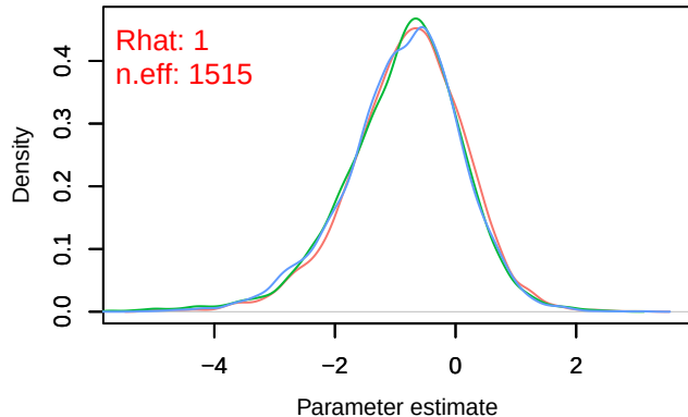
Density – B[p_milieuD (C4), Pica_pica (S8)]
