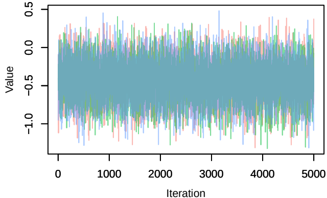
Trace – B[p_milieuD (C4), Parus_major (S4)]
