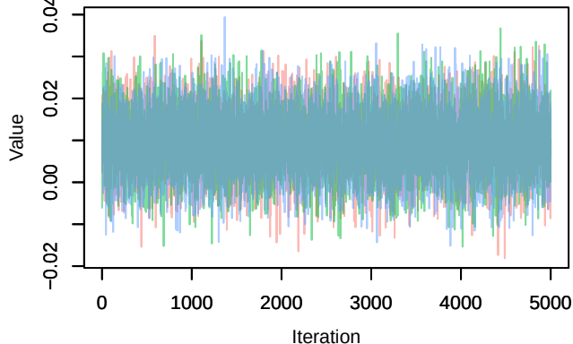
Trace – B[(Intercept) (C1), Dendrocopos_major (S5)] Density – B[(Intercept) (C1), Dendrocopos_major (S5)]
