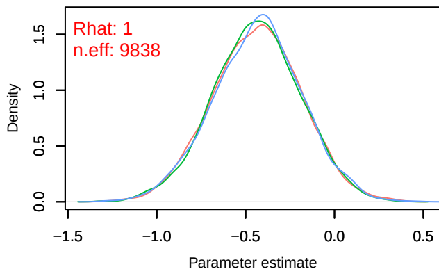
Density – B[p_milieuD (C4), Parus_major (S4)]
