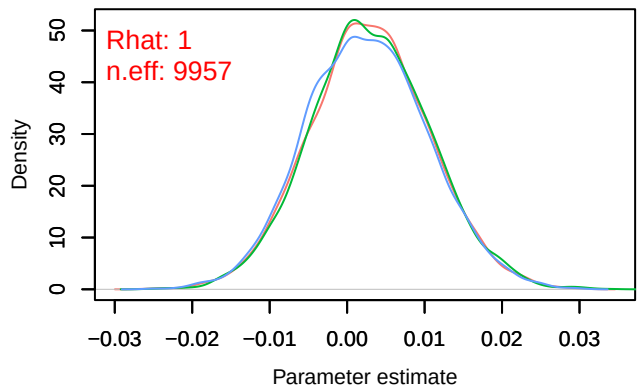
Density – B[light_pollution (C7), Turdus_merula (S3)]
