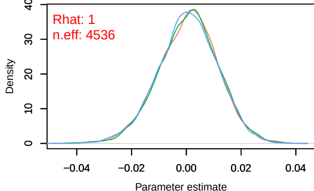
Density – B[(Intercept) (C1), Periparus_ater (S15)]
