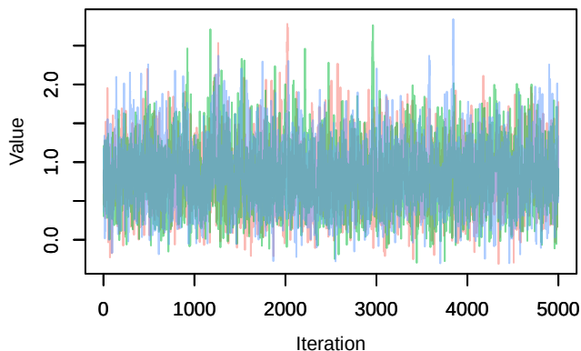
Trace – B[p_milieuE (C5), Carduelis cannabina (S:
