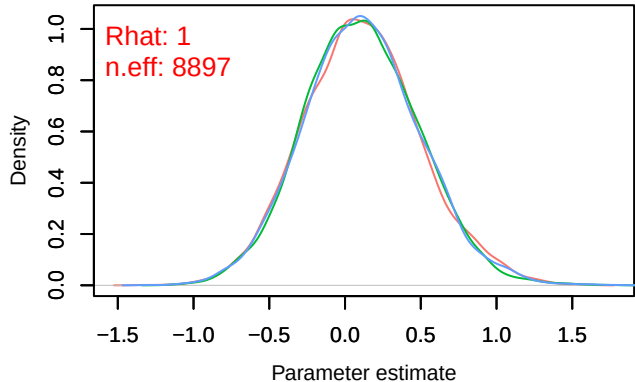
Trace – B[light_pollution (C7), Columba_palumbus (S5)] Density – B[light_pollution (C7), Columba_palumbus (S5)]
