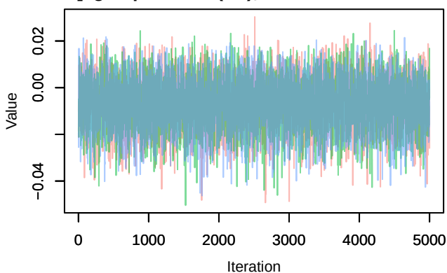
Trace – B[light_pollution (C7), Phoenicurus_ochruros (S...)
