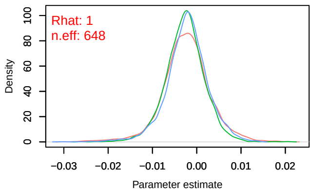
Density – B[altitude (C9), Anthus_trivialis (S14)]
