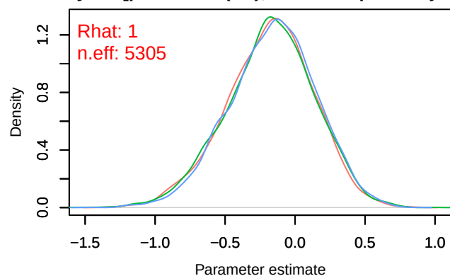
Density – B[p_milieuC (C5), Dendrocopos_major (S
