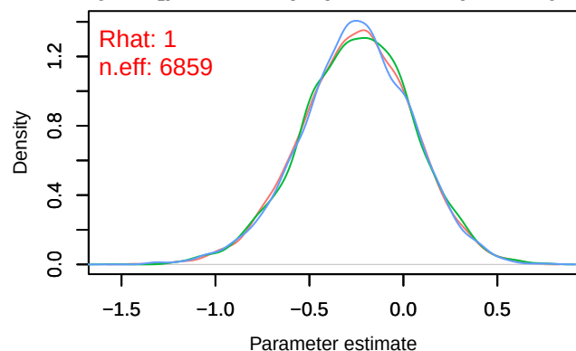
Density – B[p_milieuB (C4), Dendrocopos_major (S
