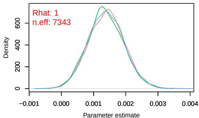
Density – B[altitude (C9), Sylvia atricapilla (S1)]
