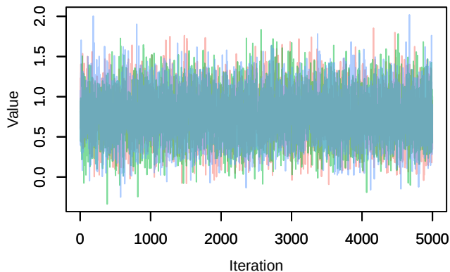
Trace – B[p_milieuE (C7), Carduelis_chloris (S7)]
