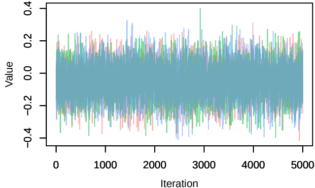
Trace – B[tmp_spring (C11), Dendrocopos_major (
