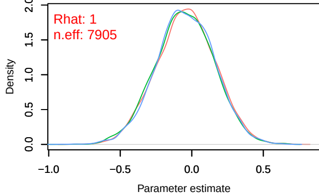
Density – B[tmp_spring (C11), Dendrocopos_major
