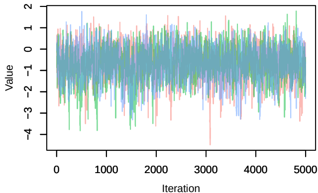
Trace – B[p_milieuF (C8), Periparus_ater (S15)]
