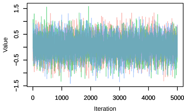
Trace – B[p_milieuF (C8), Sylvia atricapilla (S1)]
