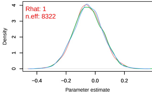
Density – B[tmp_spring (C11), Dendrocopos_major
