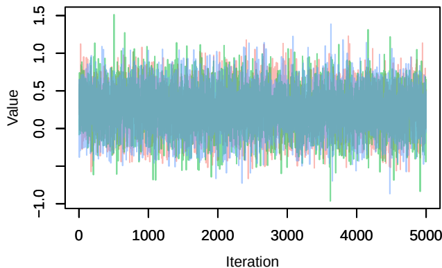
Trace – B[p_milieuE (C7), Sylvia atricapilla (S1)]
