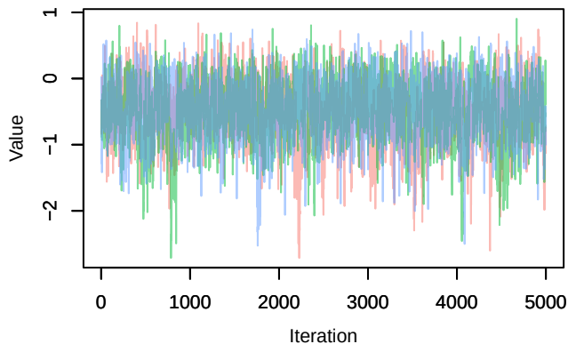
Trace – B[p_milieuD (C6), Periparus_ater (S15)]
