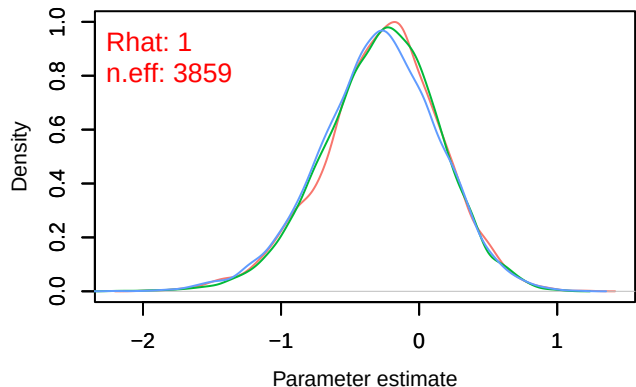
Density – B[p_milieuF (C8), Carduelis_chloris (S7)]
