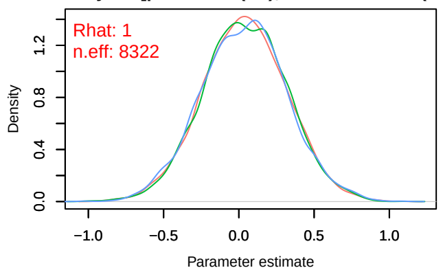
Density – B[p_milieuC (C5), Turdus_merula (S3)]
