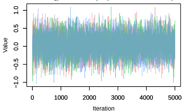
Trace – B[p_milieuC (C5), Turdus_merula (S3)]
