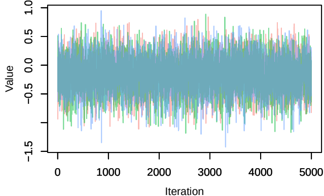
Trace – B[p_milieuB (C4), Carduelis_chloris (S7)
