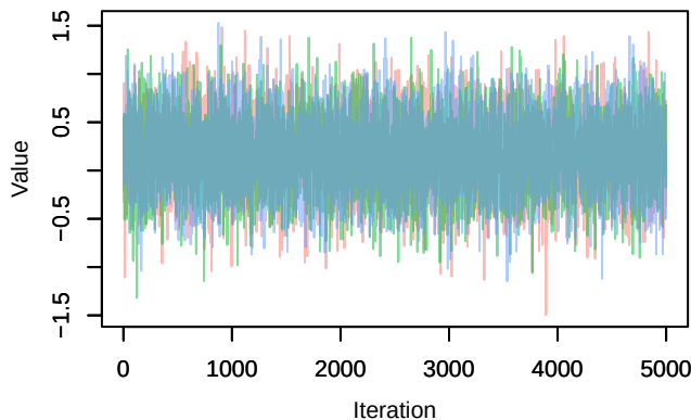
Trace – B[p_milieuF (C8), Fringilla_coelebs (S2)]
