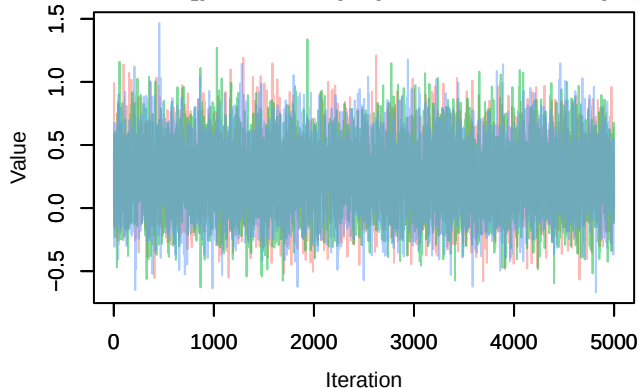
Trace – B[p_milieuB (C4), Turdus_merula (S3)]
