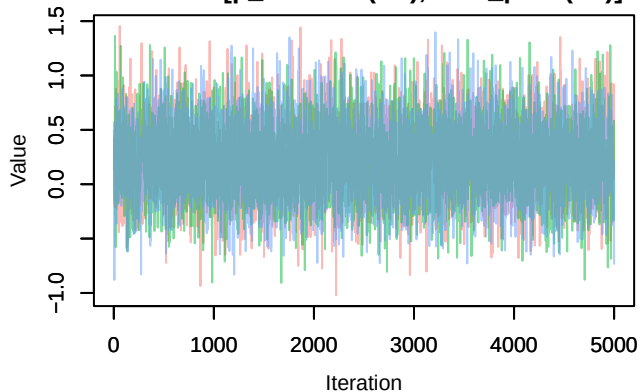
Trace – B[p_milieuD (C6), Pica_pica (S8)]
