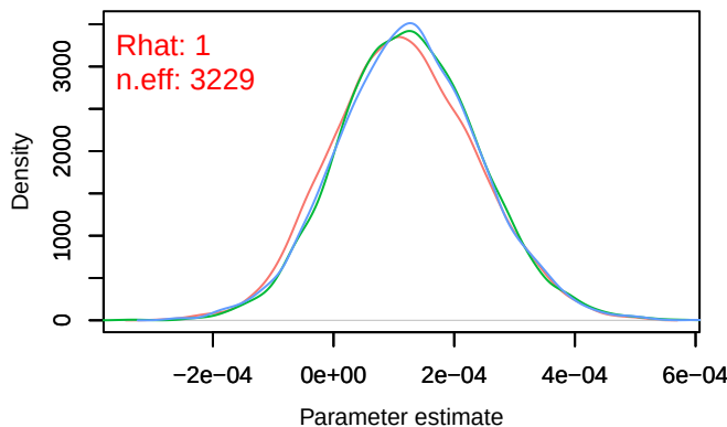
Density – B[NDVI (C2), Anthus_trivialis (S14)]
