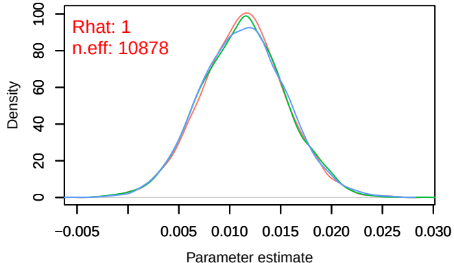
Density – B[p_milieuB (C4), Columba_palumbus (S5)]
