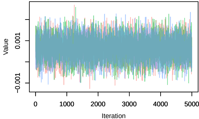
Trace – B[precip_spring (C10), Dendrocopos_major (S6)]
