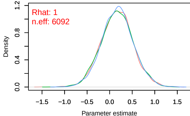
Density – B[p_milieuF (C8), Fringilla_coelebs (S2)]
