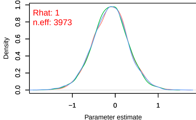
Density – B[p_milieuF (C8), Pica_pica (S8)]
