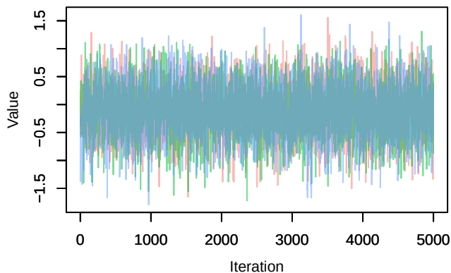
Trace – B[p_milieuF (C8), Pica_pica (S8)]
