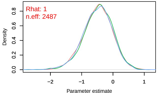
Density – B[altitude (C9), Turdus_viscivorus (S13)
