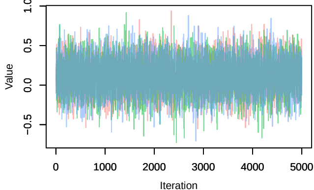
Trace – B[precip_spring (C10), Pica_pica (S8)]
