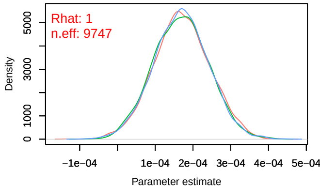
Density – B[NDVI (C2), Turdus merula (S3)]
