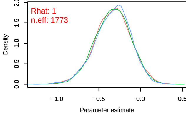
Density – B[tmp_spring (C11), Periparus_ater (S15)]
