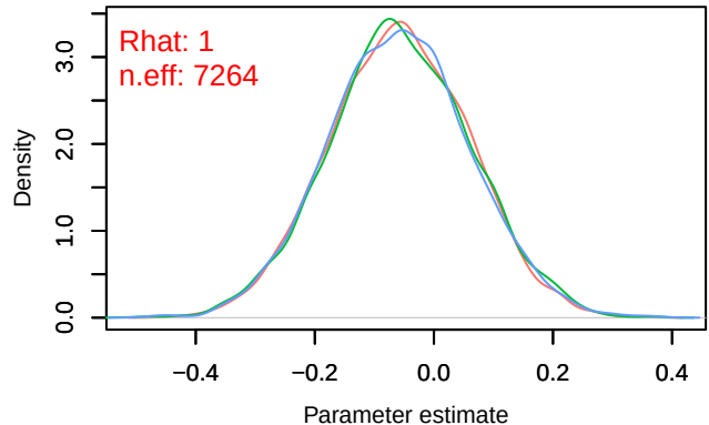
Density – B[tmp_spring (C11), Dendrocopos_major (S6)]
