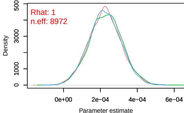
Density – B[NDVI (C2), Parus_major (S4)]
