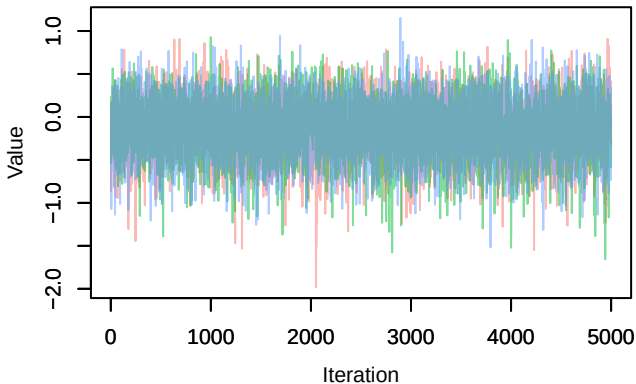
Trace – B[p_milieuC (C5), Dendrocopos_major (S)
