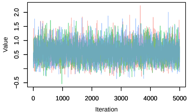
Trace – B[p_milieuE (C7), Carduelis cannabina (S
