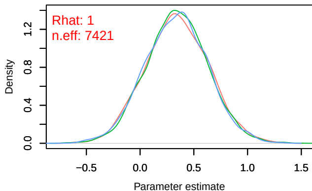
Density – B[p_milieuE (C7), Sylvia atricapilla (S1)]
