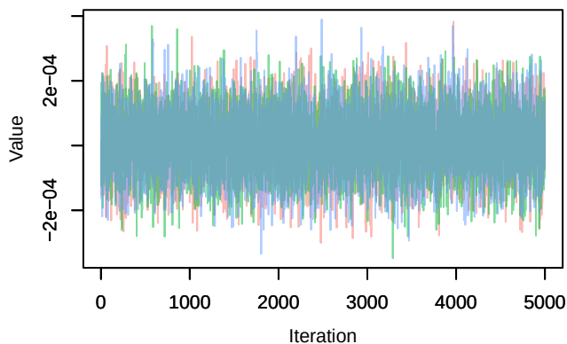
Trace – B[NDVI (C2), Carduelis_chloris (S7)]
