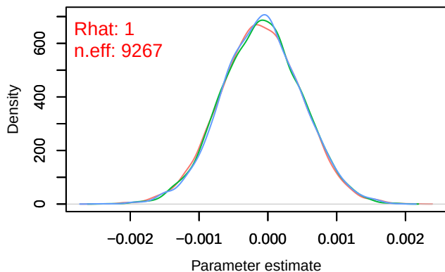
Density – B[altitude (C9), Turdus_merula (S3)]
