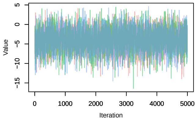
Trace – B[(Intercept) (C1), Turdus_viscivorus (S13)]
