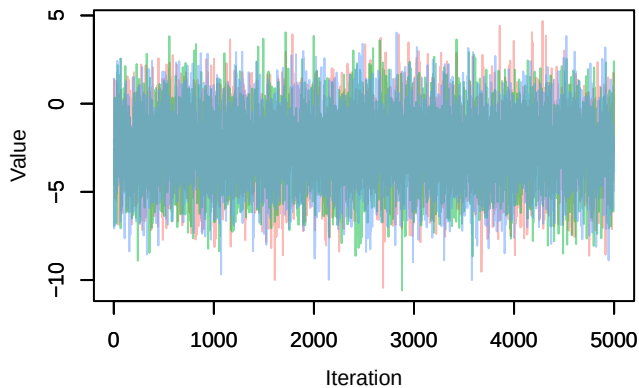
Trace – B[(Intercept) (C1), Carduelis_chloris (S7)]
