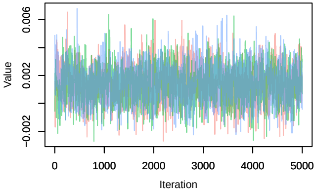
Trace – B[precip_spring (C10), Periparus_ater (S15)]
