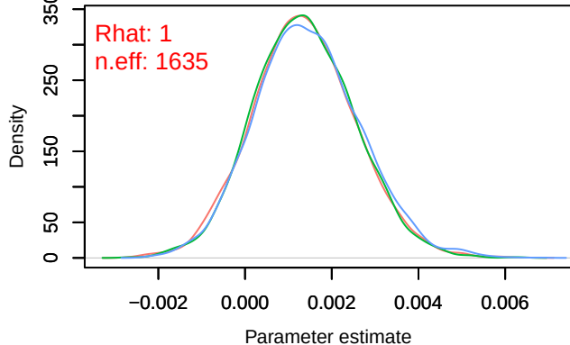
Density – B[precip_spring (C10), Periparus_ater (S15)]
