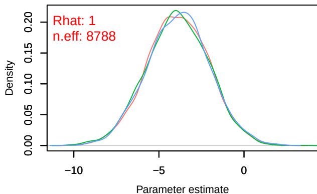
Density – B[(Intercept) (C1), Parus_major (S4)]
