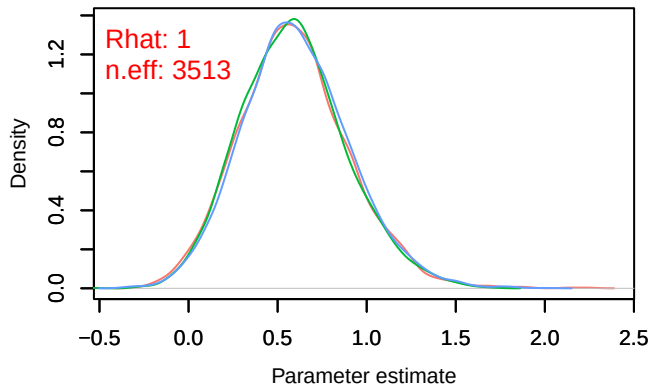
Density – B[p_milieuE (C7), Carduelis cannabina (S
