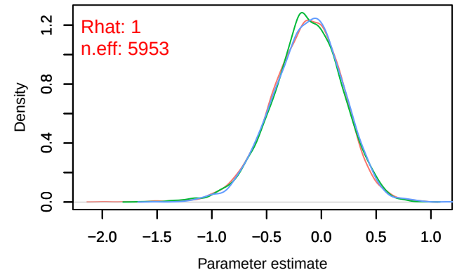
Density – B[p_milieuC (C5), Dendrocopos_major (S)
