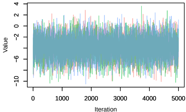
Trace – B[(Intercept) (C1), Parus_major (S4)]
