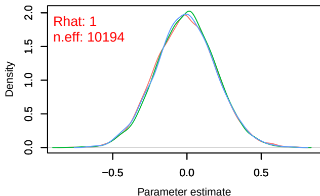
Density – B[precip_spring (C10), Turdus_merula (S3)]
