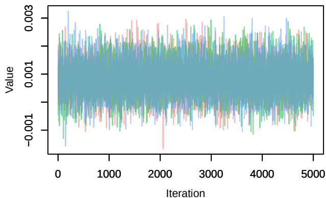
Trace – B[altitude (C9), Sylvia atricapilla (S1)]
