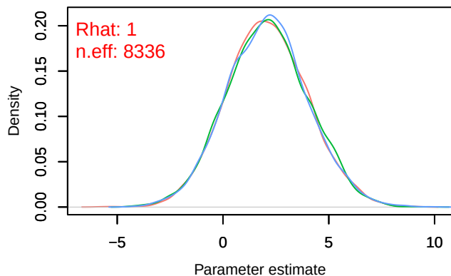
Density – B[(Intercept) (C1), Sylvia_atricapilla (S1)]
