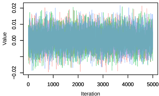
Trace – B[light_pollution (C3), Sylvia_atricapilla (S1)]
