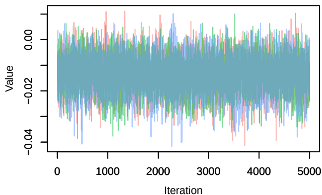
Trace – B[light_pollution (C3), Carduelis_chloris (S7)]
