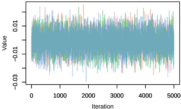
Trace – B[p_milieuB (C4), Dendrocopos_major (S)
