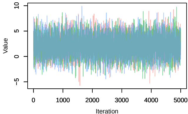
Trace – B[(Intercept) (C1), Sylvia_atricapilla (S1)]
