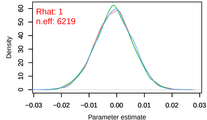
Density – B[p_milieuB (C4), Dendrocopos_major (S)
