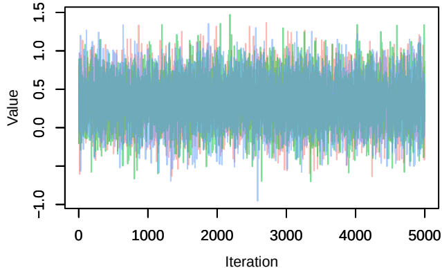
Trace – B[p_milieuE (C7), Sylvia atricapilla (S1)]
