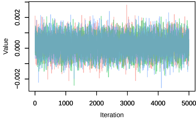
Trace – B[precip_spring (C10), Dendrocopos_major Density – B[precip_spring (C10), Dendrocopos_major
