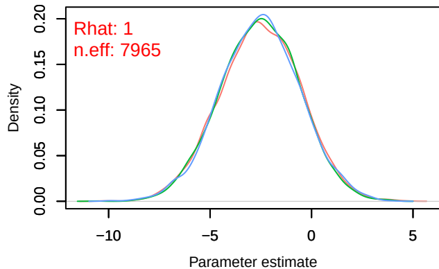
Density – B[(Intercept) (C1), Carduelis_chloris (S7)]
