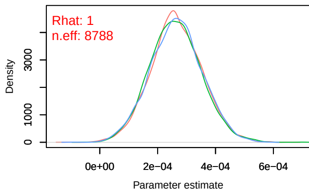
Density – B[NDVI (C2), Sylvia_atricapilla (S1)]
