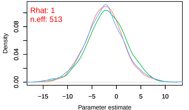
Density – B[NDVI (C2), Turdus_viscivorus (S13)]
