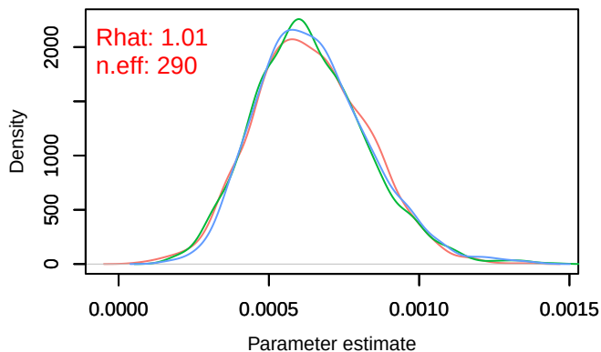
Density – B[NDVI (C2), Fringilla_coelebs (S2)]
