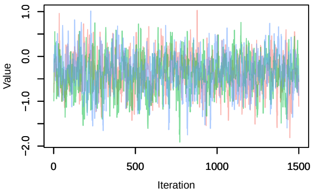
Trace – B[precip_spring (C10), Sylvia_communis (S
