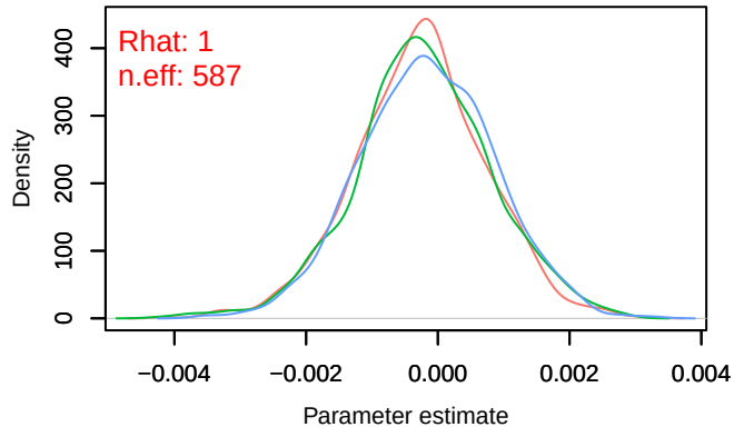
Density – B[altitude (C9), Turdus_viscivorus (S13)
