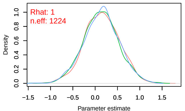
Density – B[p_milieuF (C8), Turdus_merula (S3)]
