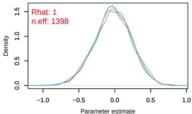
Density – B[p_milieuD (C6), Turdus_merula (S3)]
