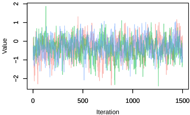
Trace – B[p_milieuF (C8), Carduelis_cannabina (S1) Density – B[p_milieuF (C8), Carduelis_cannabina (S1)
