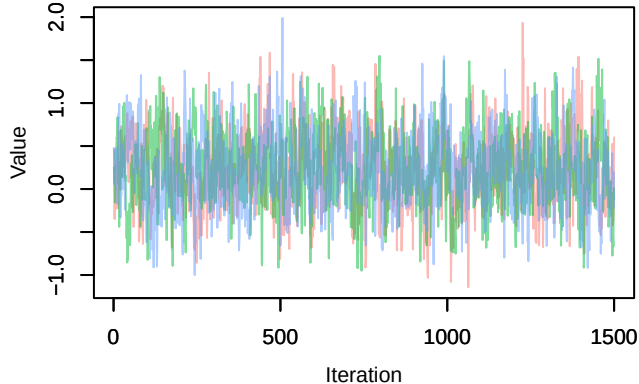
Trace – B[p_milieuB (C4), Carduelis cannabina (S
