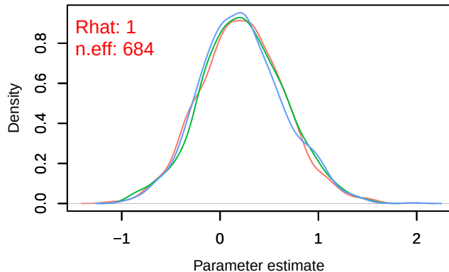
Density – B[p_milieuB (C4), Carduelis cannabina (S
