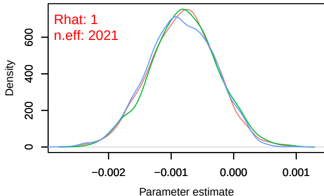
Density – B[precip_spring (C10), Columba_palumbus (S5)]
