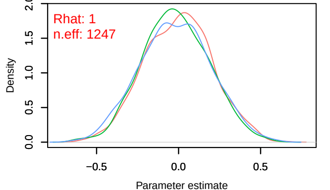
Density – B[tmp_spring (C11), Dendrocopos_major (S6)]
