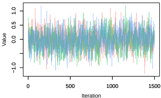
Trace – B[p_milieuB (C4), Fringilla_coelebs (S2)]
