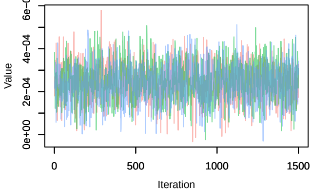
Trace – B[NDVI (C2), Fringilla_coelebs (S2)]
