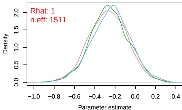
Density – B[precip_spring (C10), Columba_palumbus (S5)]
