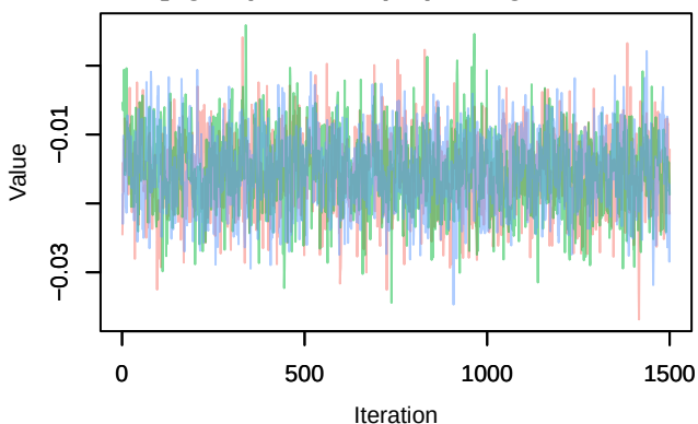
Trace – B[light_pollution (C3), Fringilla_coelebs (S2)]
