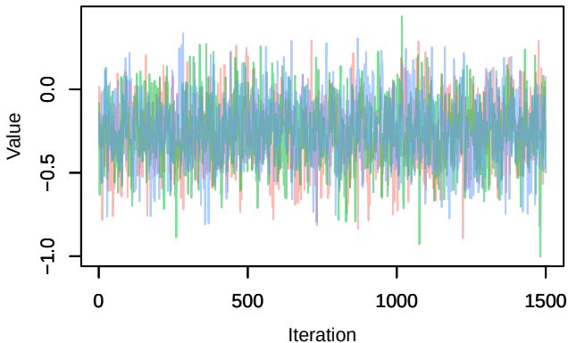
Trace – B[precip_spring (C10), Columba_palumbus (S5)]
