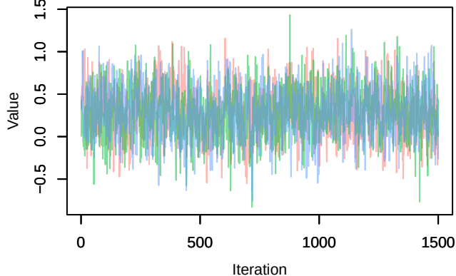
Trace – B[p_milieuC (C5), Fringilla_coelebs (S2)
