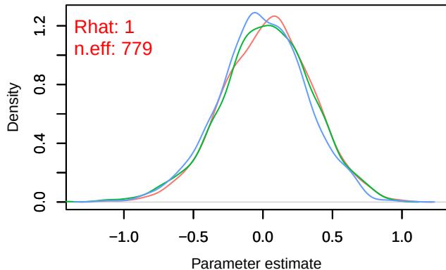
Trace – B[precip_spring (C10), Carduelis_cannabina (S11
