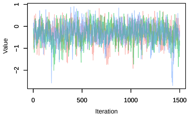
Trace – B[p_milieuF (C8), Carduelis_chloris (S7)]
