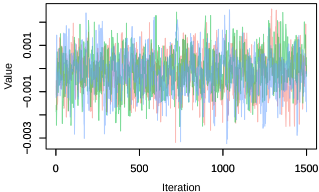
Trace – B[precip_spring (C10), Carduelis_cannabina (S11
