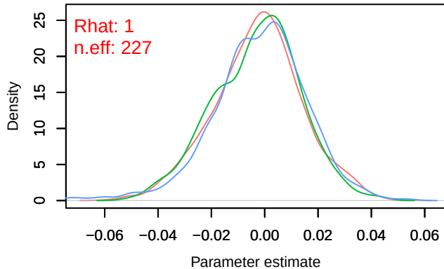
Density – B[p_milieuB (C4), Periparus_ater (S15)]
