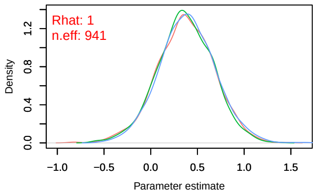
Density – B[tmp_spring (C11), Turdus_viscivorus (S14)]
