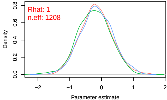
Density – B[p_milieuD (C6), Columba_palumbus (S
