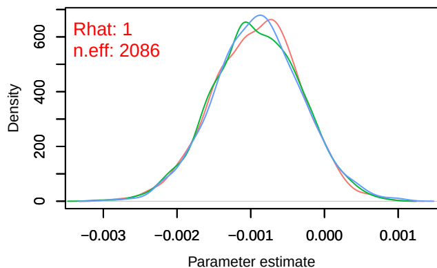
Density – B[altitude (C9), Columba_palumbus (S5)
