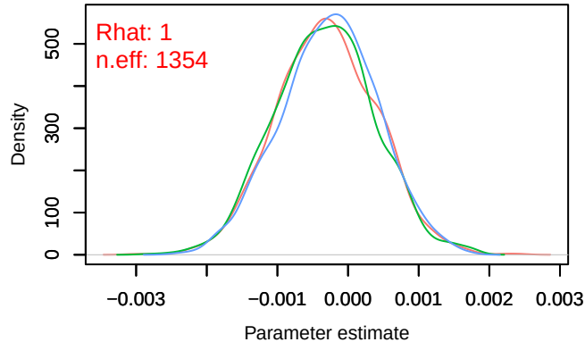
Trace – B[precip_spring (C10), Dendrocopos_major Density – B[precip_spring (C10), Dendrocopos_major
