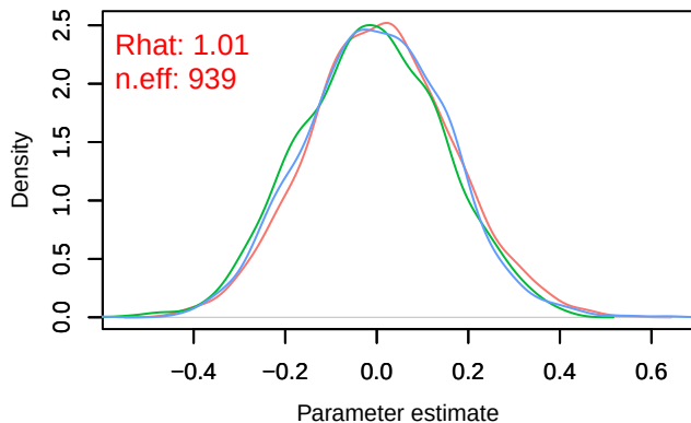
Density – B[tmp_spring (C11), Pica_pica (S8)]
