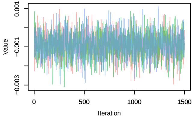
Trace – B[altitude (C9), Columba_palumbus (S5)
