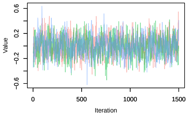
Trace – B[tmp_spring (C11), Pica_pica (S8)]
