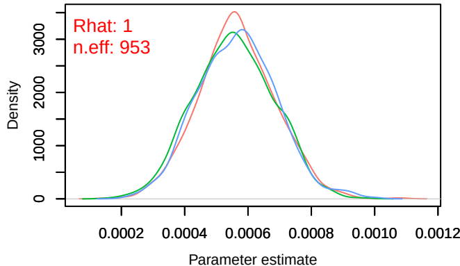
Density – B[light_pollution (C3), Fringilla_coelebs (S2)]
