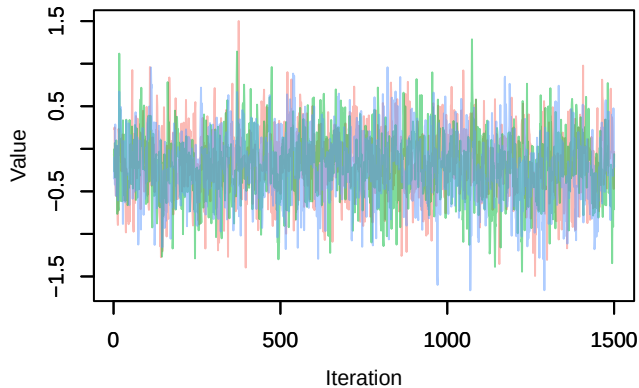
Trace – B[p_milieuB (C4), Sylvia atricapilla (S1)
