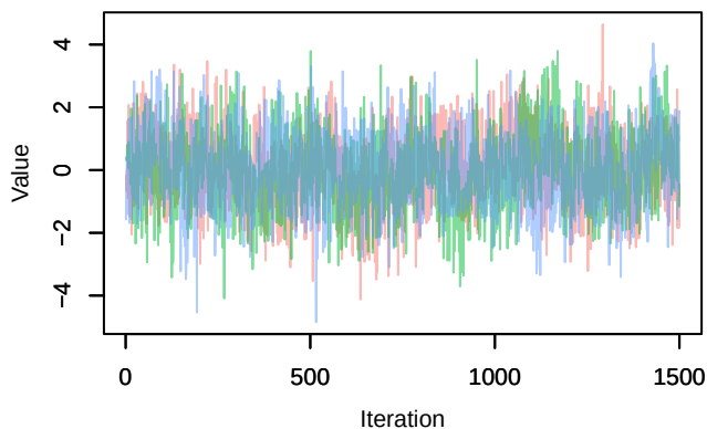
Trace – B[p_milieuC (C5), Sylvia atricapilla (S1)
