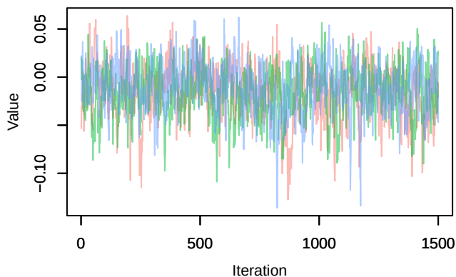
Trace – B[light_pollution (C3), Pica_pica (S8)]
