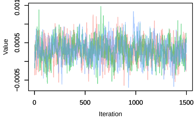
Trace – B[NDVI (C2), Pica_pica (S8)]
