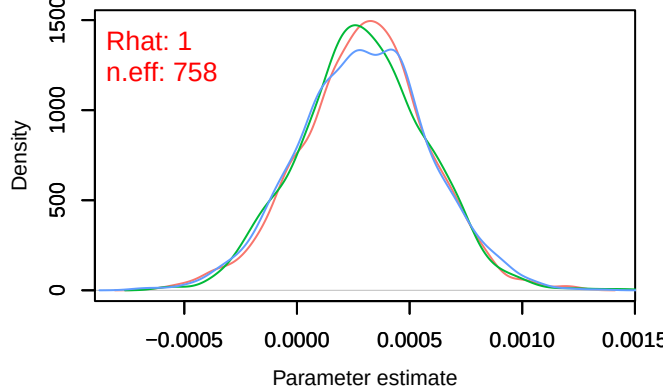
Density – B[NDVI (C2), Pica_pica (S8)]
