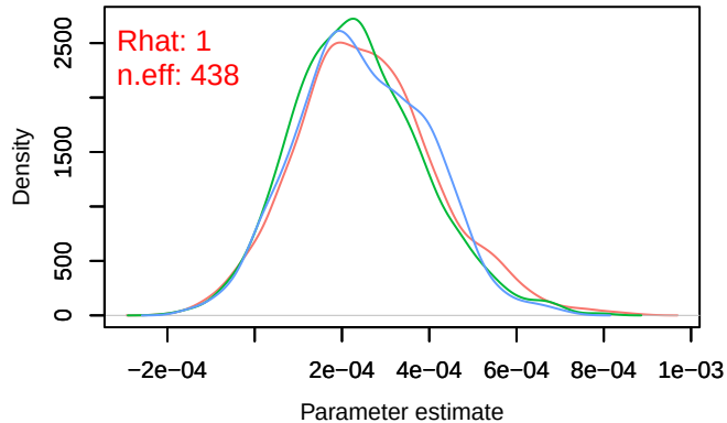
Density – B[light_pollution (C3), Anthus_trivialis (S
