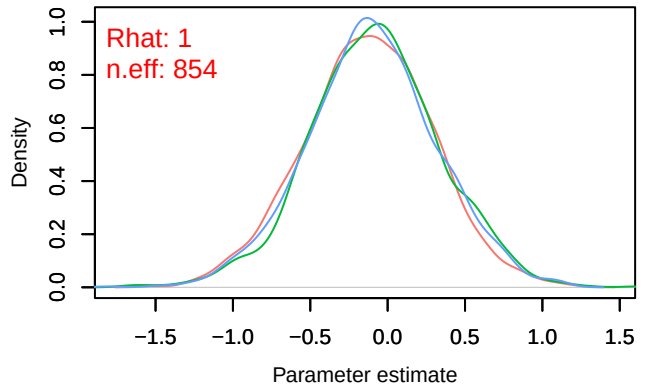
Density – B[p_milieuB (C4), Anthus_trivialis (S14)
