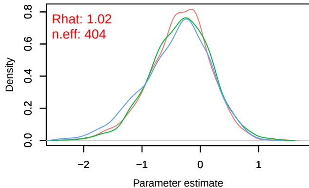
Trace – B[altitude (C9), Carduelis_cannabina (S1) Density – B[altitude (C9), Carduelis_cannabina (S1)
