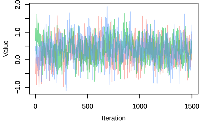
Trace – B[p_milieuE (C7), Parus_major (S4)]
