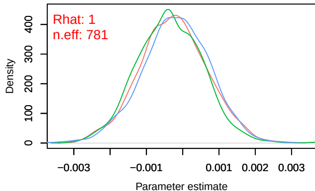
Trace – B[precip_spring (C10), Carduelis_cannabina (S1) Density – B[precip_spring (C10), Carduelis_cannabina (S1)
