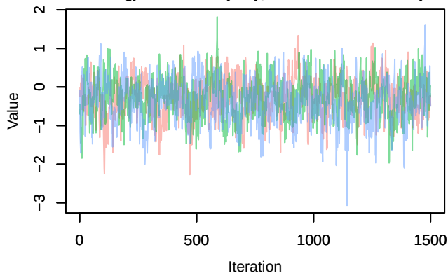
Trace – B[altitude (C9), Anthus_trivialis (S14)]
