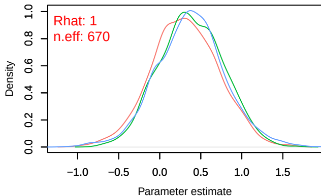
Density – B[p_milieuE (C7), Parus_major (S4)]
