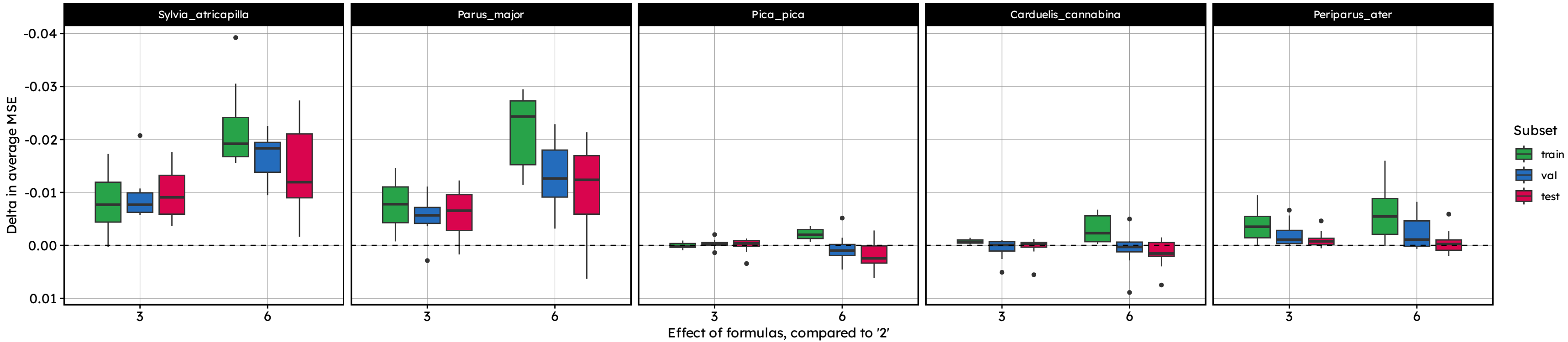
Distribution of per-fold differences across k_fold, per species
