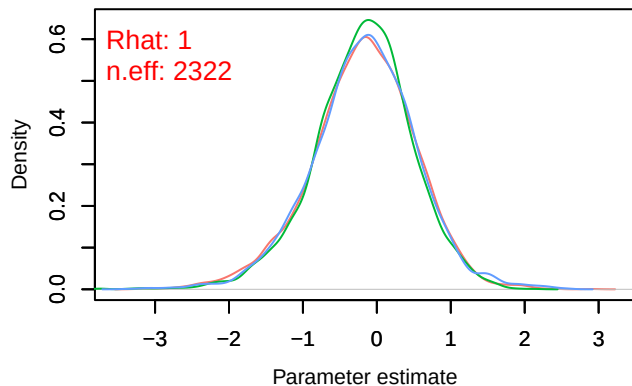
Density – B[p_milieuC (C3), Pica_pica (S3)]
