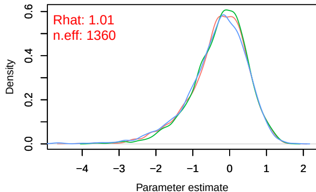
Density – B[p_milieuE (C5), Periparus_ater (S5)]
