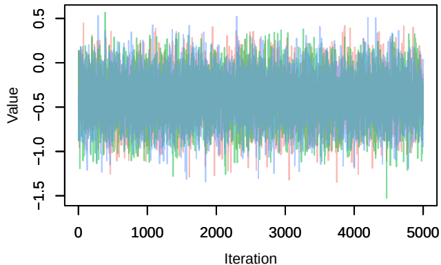
Trace – B[p_milieuE (C5), Parus_major (S2)]
