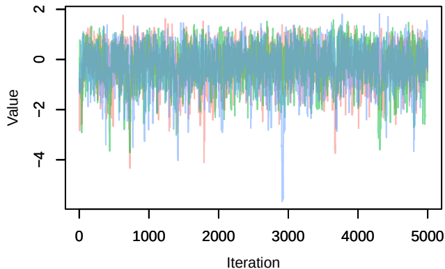
Trace – B[p_milieuE (C5), Periparus_ater (S5)]
