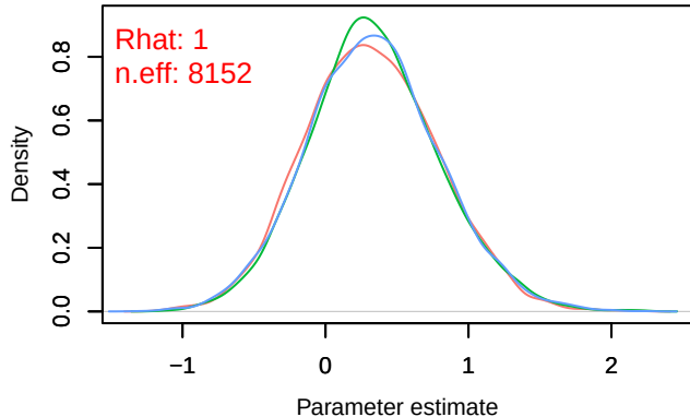
Density – B[light_pollution (C7), Parus_major (S2)]
