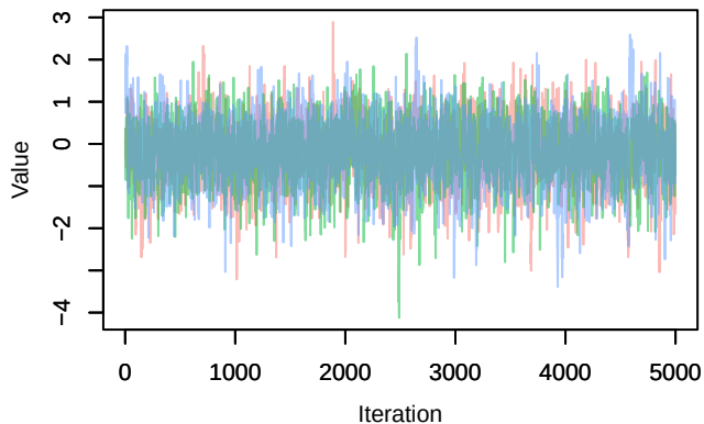
Trace – B[p_milieuC (C3), Pica_pica (S3)]
