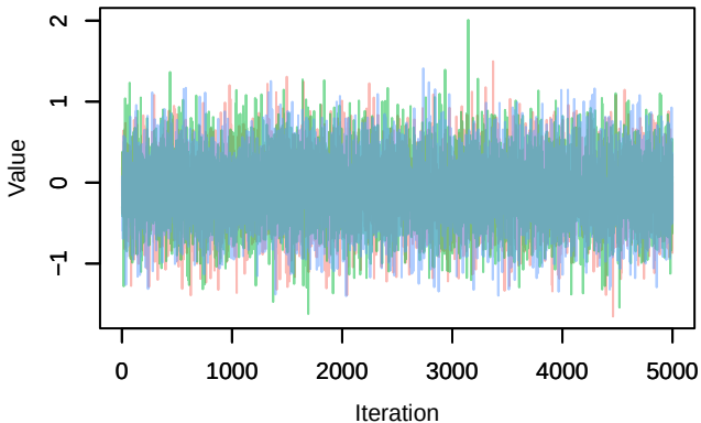
Trace – B[p_milieuB (C2), Parus_major (S2)]
