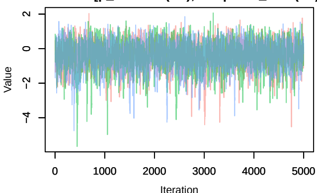
Trace – B[p_milieuB (C2), Periparus_ater (S5)]
