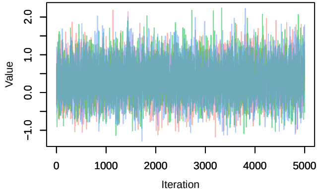
Trace – B[light_pollution (C7), Parus_major (S2)]
