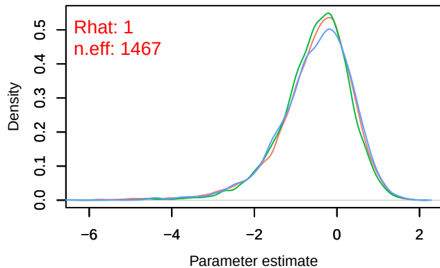
Density – B[light_pollution (C7), Periparus_ater (S5)]
