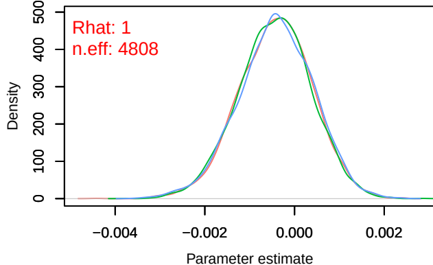
Density – B[altitude (C8), Pica_pica (S3)]
