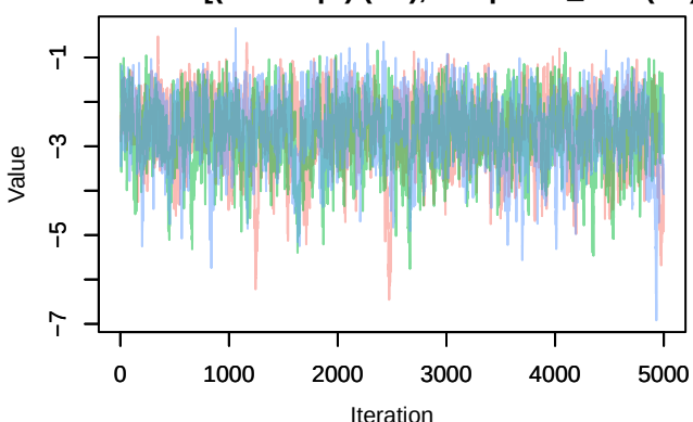
Trace – B[(Intercept) (C1), Periparus_ater (S5)]
