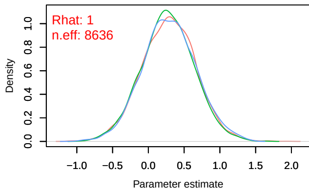
Density – B[p_milieuE (C5), Parus_major (S2)]
