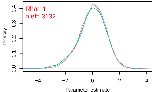
Density – B[p_milieuC (C3), Carduelis_cannabina (S
