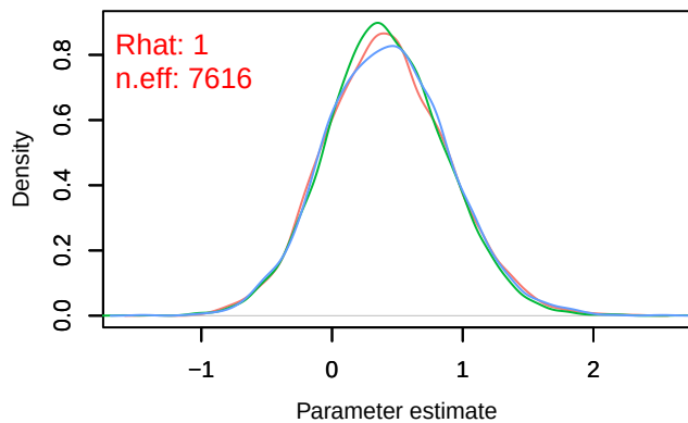
Density – B[p_milieuF (C6), Parus_major (S2)]
