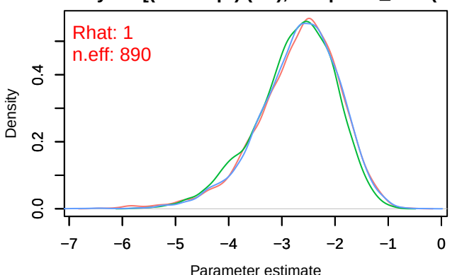
Density – B[(Intercept) (C1), Periparus_ater (S5)]
