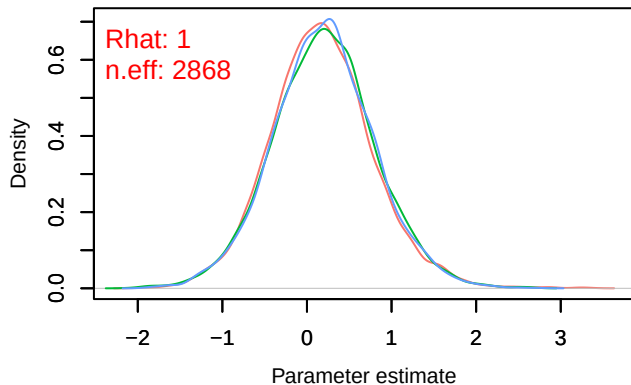
Density – B[light_pollution (C7), Pica_pica (S3)]
