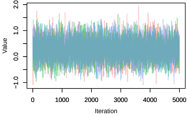
Trace – B[p_milieuE (C5), Parus_major (S2)]
