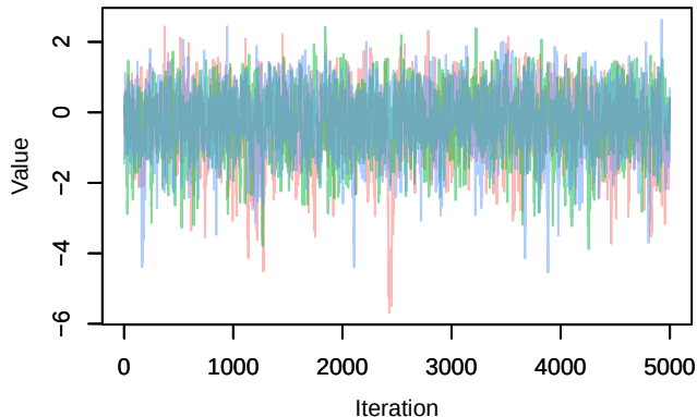
Trace – B[light_pollution (C7), Periparus_ater (S5)]
