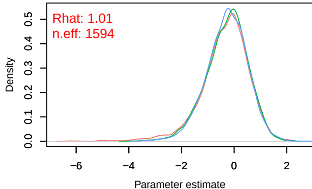
Density – B[p_milieuC (C3), Periparus_ater (S5)]
