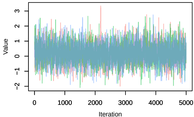
Trace – B[light_pollution (C7), Pica_pica (S3)]
