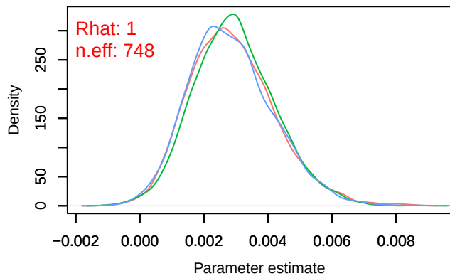
Density – B[altitude (C8), Periparus_ater (S5)]
