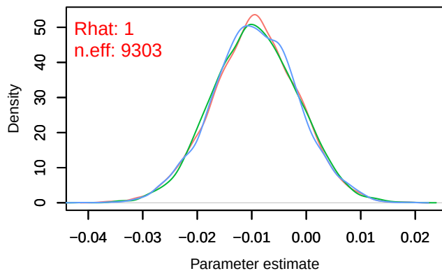
Density – B[light_pollution (C7), Parus_major (S2)]
