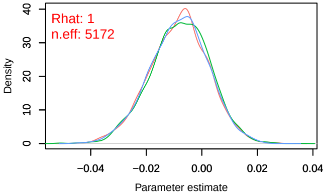
Density – B[altitude (C8), Carduelis_cannabina (S4
