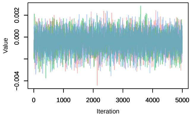
Trace – B[altitude (C8), Pica_pica (S3)]
