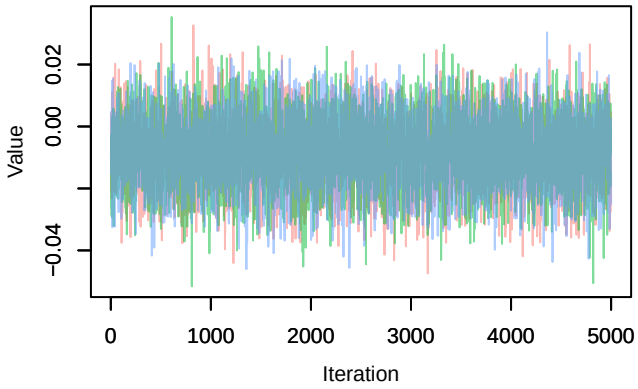
Trace – B[altitude (C8), Carduelis_cannabina (S4
