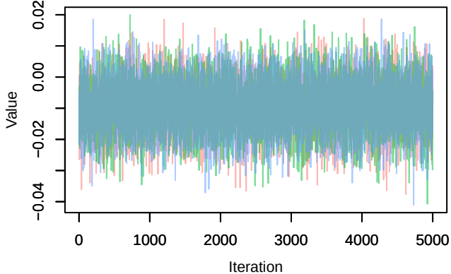
Trace – B[light_pollution (C7), Parus_major (S2)]
