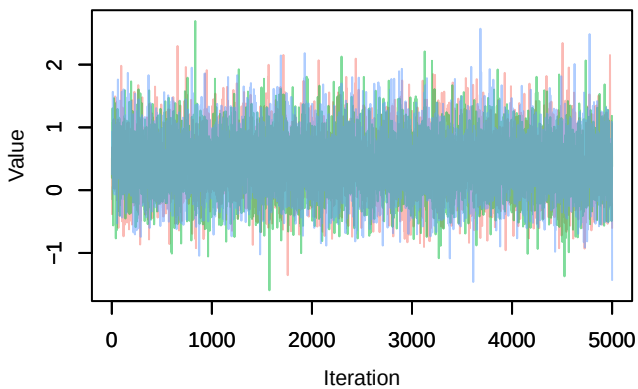
Trace – B[p_milieuF (C6), Parus_major (S2)]
