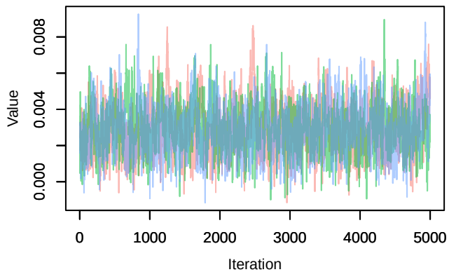
Trace – B[altitude (C8), Periparus_ater (S5)]
