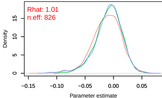
Density – B[light_pollution (C7), Periparus_ater (S5)]
