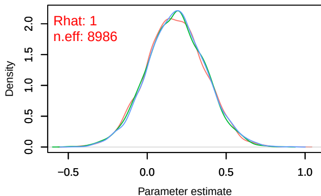
Density – B[tmp_spring (C11), Parus_major (S2)]
