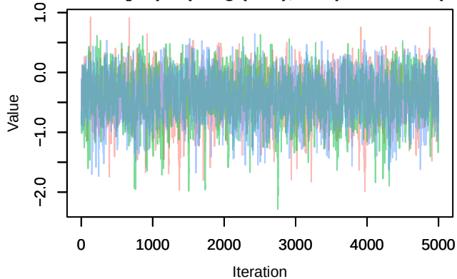
Trace – B[tmp_spring (C11), Periparus_ater (S5)
