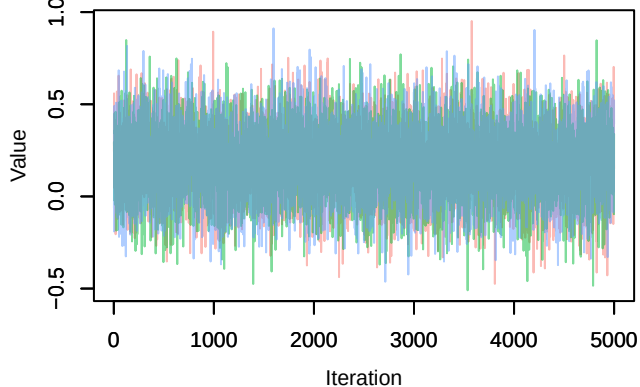
Trace – B[tmp_spring (C11), Parus_major (S2)]
