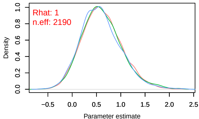
Density – B[p_milieuD (C6), Pica_pica (S3)]
