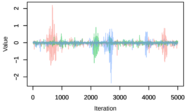
Trace – Omega1[Carduelis_cannabina (S4), Parus_majnsity – Omega1[Carduelis_cannabina (S4), Parus_majnsity]
