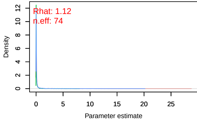
Density – Omega1[Pica_pica (S3), Parus_major (S2)]
