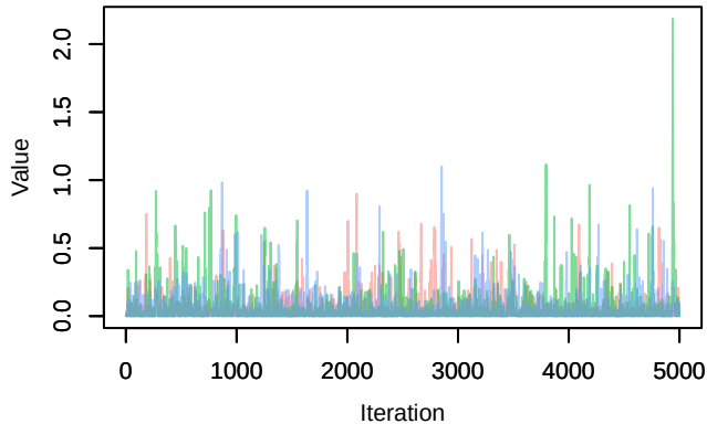
Trace – Omega1[Carduelis_cannabina (S4), Pica_pica (S4)]
