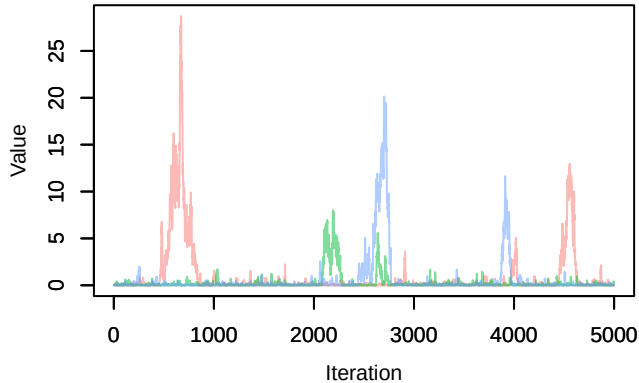
Trace – Omega1[Pica_pica (S3), Parus_major (S2)]
