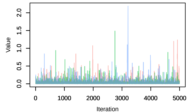
Trace – Omega1[Periparus_ater (S5), Periparus_aterDensity – Omega1[Periparus_ater (S5), Periparus_ate
