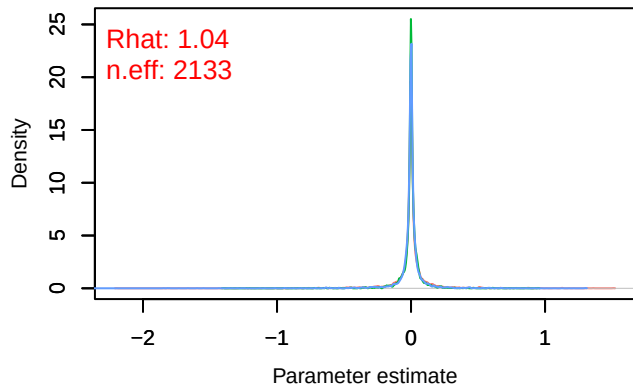
Density – Omega1[Pica_pica (S3), Periparus_ater (S
