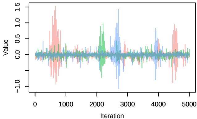
Trace – Omega1[Parus_major (S2), Pica_pica (S3
