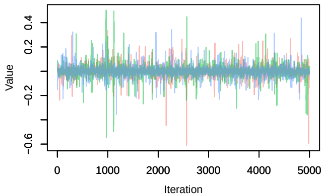
Trace – Omega1[Carduelis_cannabina (S4), Periparus_ater (S4)]
