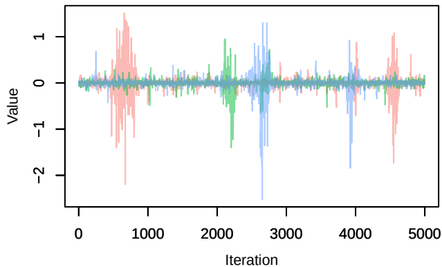
Trace – Omega1[Pica_pica (S3), Periparus_ater (S
