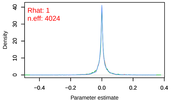
Density – Omega1[Periparus_ater (S5), Pica_pica (S5)]
