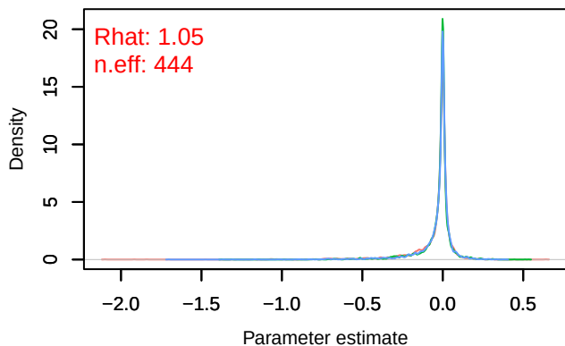
Density – Omega1[Parus_major (S2), Pica_pica (S3
