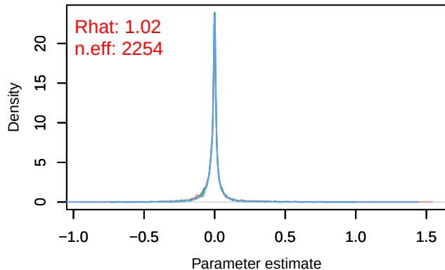
Trace – Omega1[Carduelis_cannabina (S4), Parus_majnsity – Omega1[Carduelis_cannabina (S4), Parus_majnsity]
