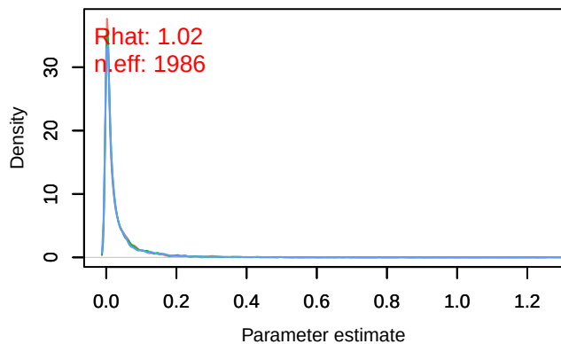
Trace – Omega1[Periparus_ater (S5), Periparus_aterDensity – Omega1[Periparus_ater (S5), Periparus_ate
