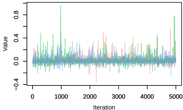
Trace – Omega1[Periparus_ater (S5), Pica_pica (S5)]
