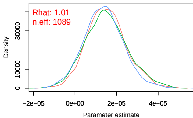
Trace – B[distance.to.permanent.crops (C9), sp_24 (Density – B[distance.to.permanent.crops (C9), sp_24
