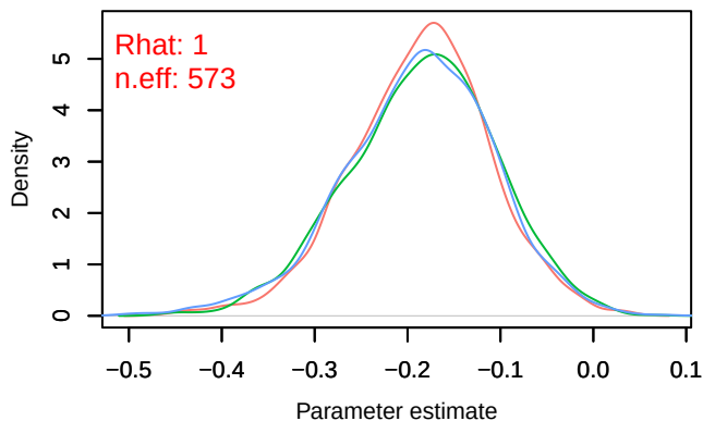
Density – B[chelsea_hurs (C2), sp_38 (S38)]
