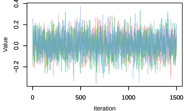
Trace – B[chelsa_tas (C4), sp_7 (S7)]
