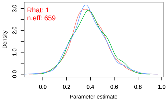
Density – B[ndvi (C5), sp_19 (S19)]
