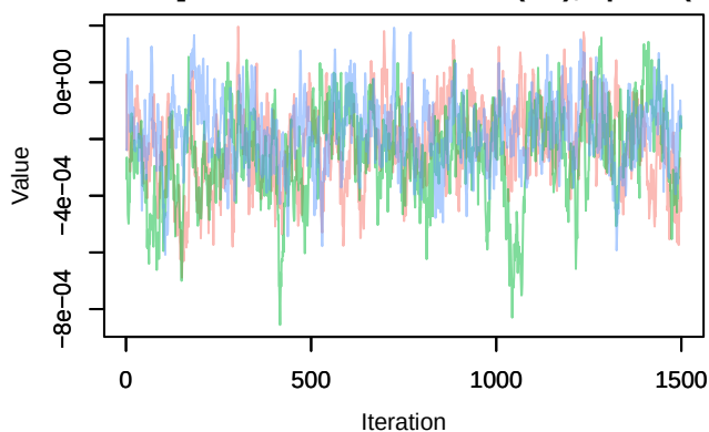
Trace – B[distance.to.arable.land (C8), sp_15 (S15)]
