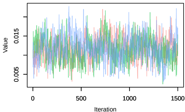
Trace – B[chelsea_pr (C3), sp_10 (S10)]
