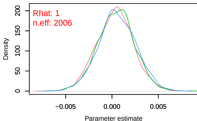
Density – B[chelsea_pr (C3), sp_35 (S35)]
