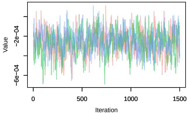
Trace – B[distance.to.arable.land (C8), sp_30 (S3
