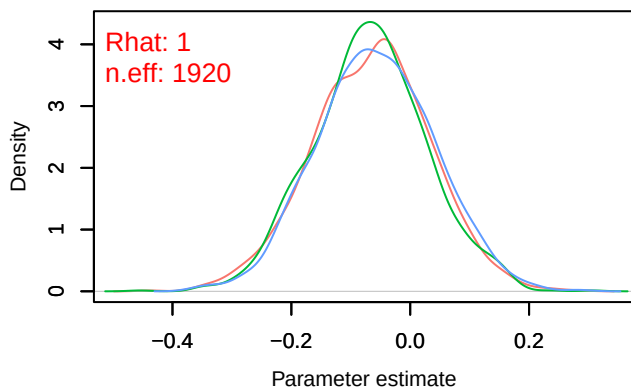
Density – B[chelsea_tas (C4), sp_35 (S35)]
