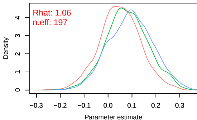
Density – B[chelsa_hurs (C2), sp_2 (S2)]
