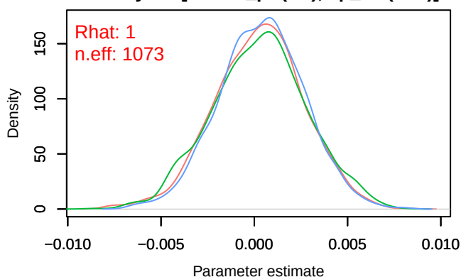
Density – B[chelsa_tas (C4), sp_23 (S23)]
