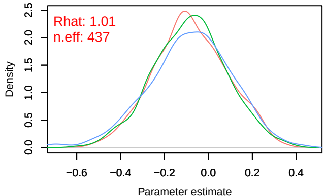
Density – B[chelsa_tas (C4), sp_33 (S33)]
