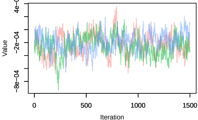
Trace – B[distance.to.water.bodies (C14), sp_29 (S29)]
