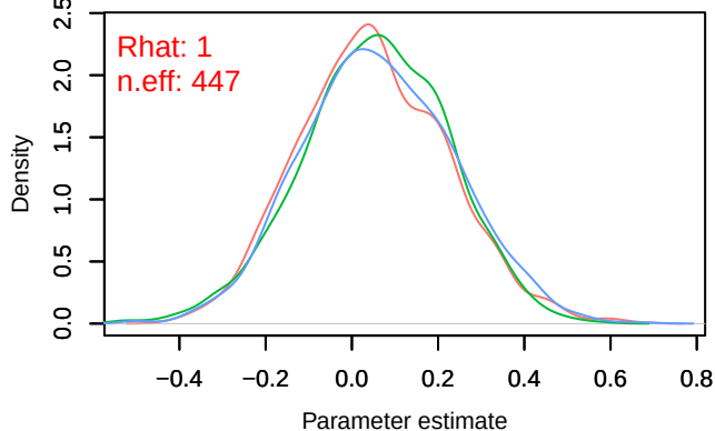
Density – B[chelsa_tas (C4), sp_2 (S2)]
