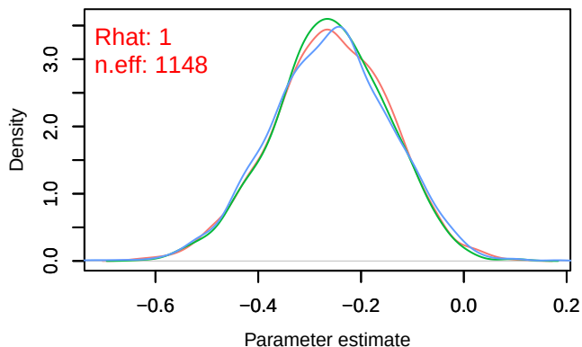
Density – B[chelsa_tas (C4), sp_24 (S24)]
