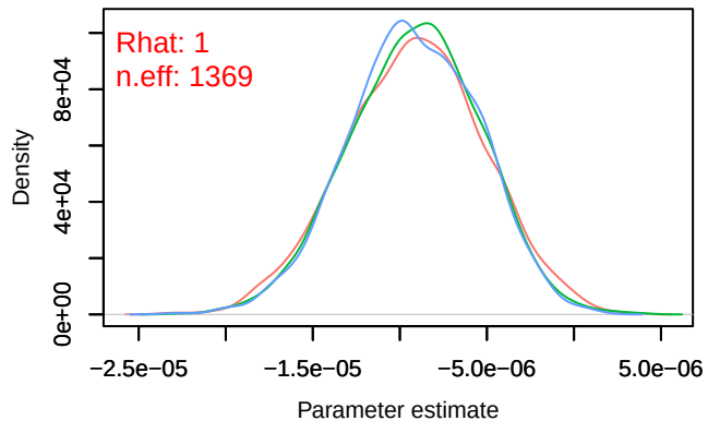
Density – B[distance.to.pastures (C10), sp_21 (S2
