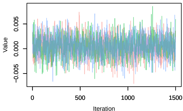
Trace – B[chelsea_pr (C3), sp_35 (S35)]
