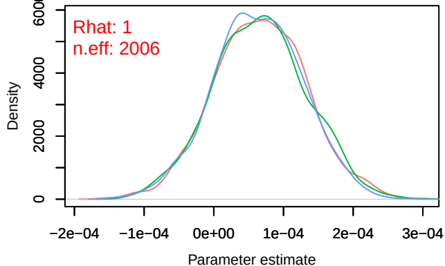
Density – B[(Intercept) (C1), sp_39 (S39)]
