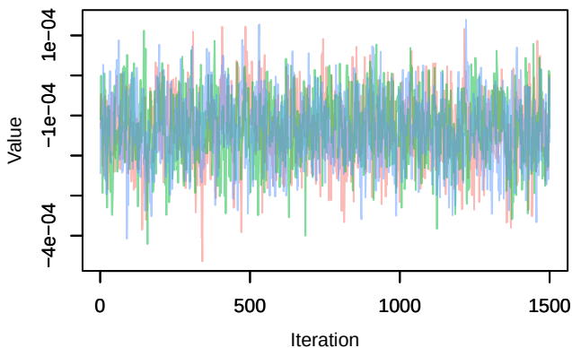
Trace – B[distance.to.arable.land (C8), sp_21 (S21
