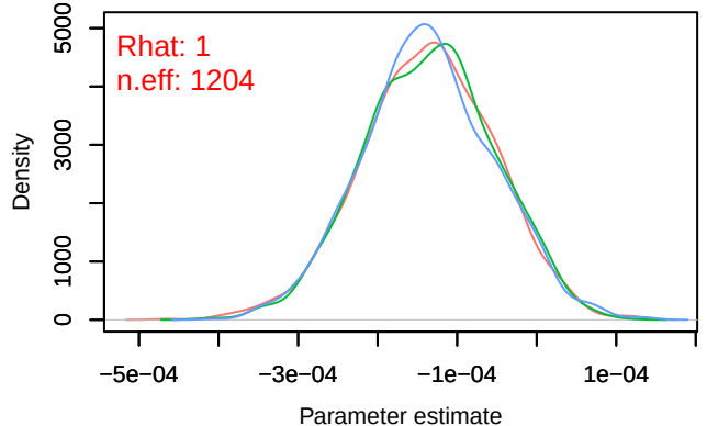
Density – B[distance.to.arable.land (C8), sp_21 (S21
