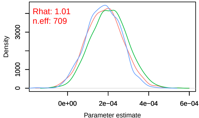
Density – B[distance.to.water.bodies (C14), sp_30 (S30)]
