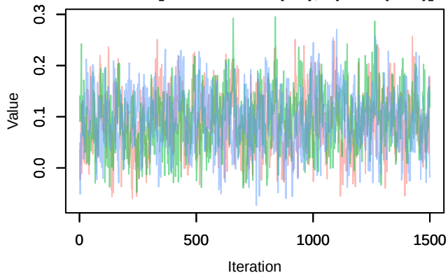
Trace – B[chelsa_pr (C3), sp_23 (S23)]
