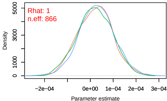
Density – B[distance.to.arable.land (C8), sp_30 (S3
