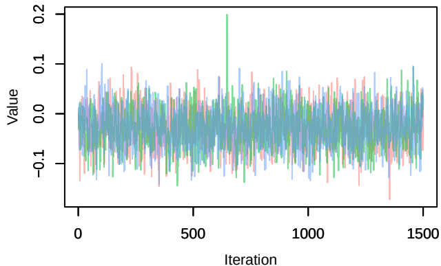
Trace – B[chelsea_hurs (C2), sp_35 (S35)]
