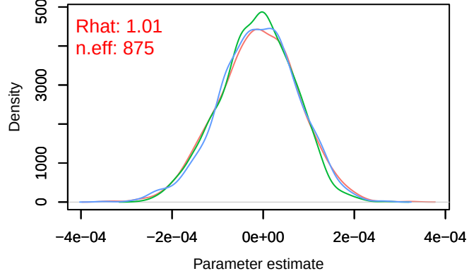
Density – B[distance.to.water.bodies (C14), sp_12 (S12)]
