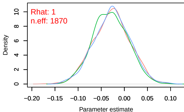
Density – B[chelsea_hurs (C2), sp_35 (S35)]
