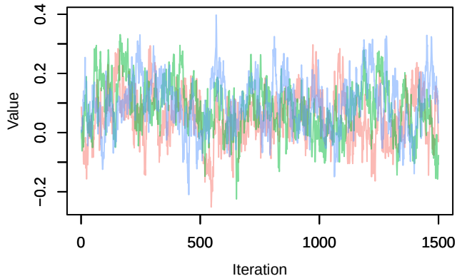
Trace – B[chelsa_hurs (C2), sp_2 (S2)]
