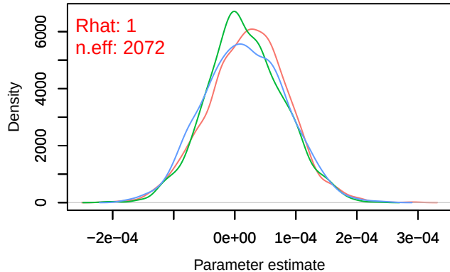
Density – B[distance.to.permanent.crops (C9), sp_38 (S38)]
