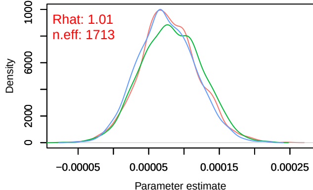
Density – B[distance.to.wetlands (C12), sp_7 (S7)]
