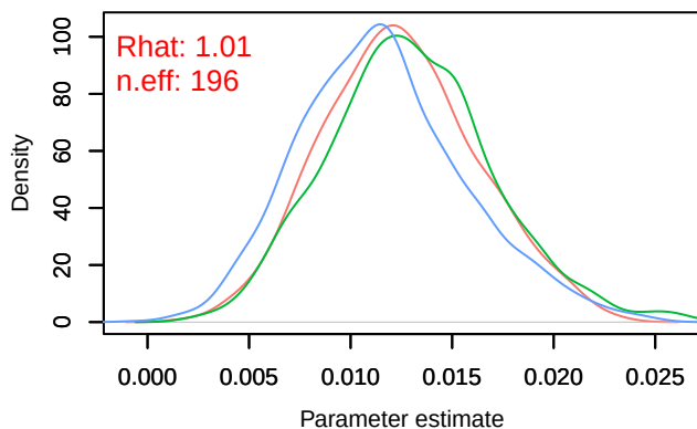
Density – B[chelsa_pr (C3), sp_29 (S29)]
