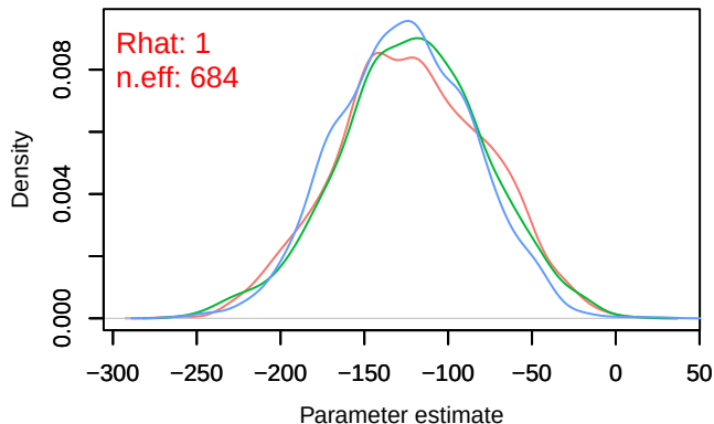
Density – B[chelsea_hurs (C2), sp_12 (S12)]
