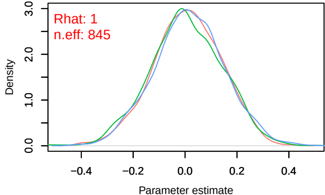
Density – B[chelsea_tas (C4), sp_26 (S26)]
