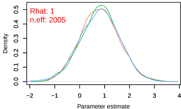
Density – B[light_pollution (C6), sp_38 (S38)]
