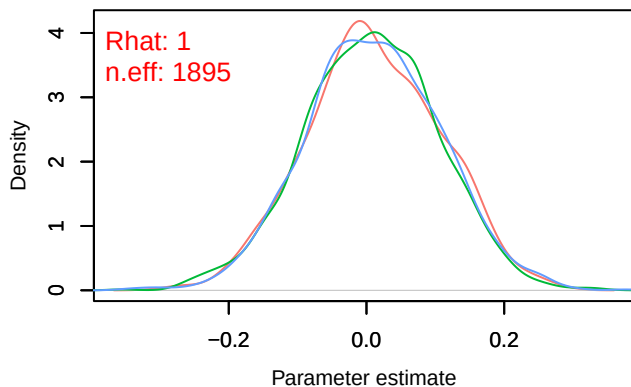
Density – B[chelsa_tas (C4), sp_7 (S7)]
