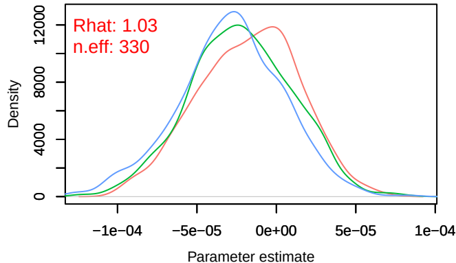
Density – B[distance.to.pastures (C10), sp_2 (S2)]
