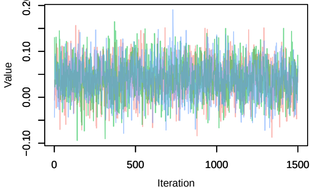
Trace – B[chelsea_hurs (C2), sp_9 (S9)]
