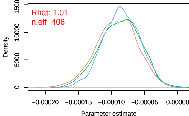
Density – B[distance.to.pastures (C10), sp_3 (S3)
