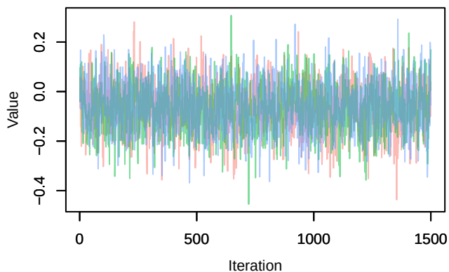
Trace – B[chelsea_tas (C4), sp_35 (S35)]
