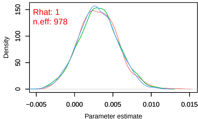
Density – B[chelsa_tas (C4), sp_27 (S27)]
