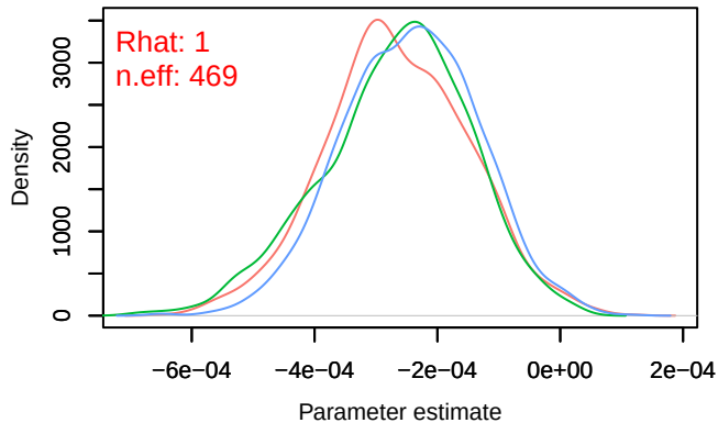
Density – B[distance.to.arable.land (C8), sp_30 (S3
