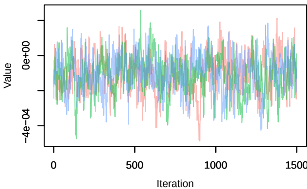
Trace – B[distance.to.artificial.surfaces (C7), sp_16 (Density – B[distance.to.artificial.surfaces (C7), sp_16
