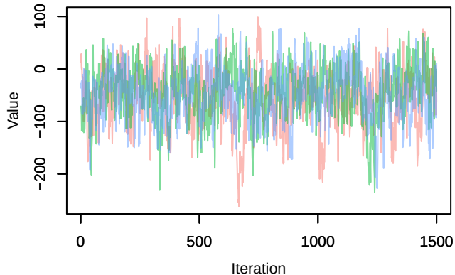
Trace – B[(Intercept) (C1), sp_4 (S4)]
