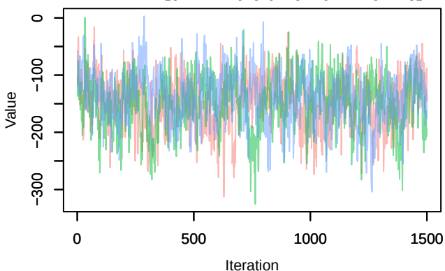
Trace – B[(Intercept) (C1), sp_30 (S30)]
