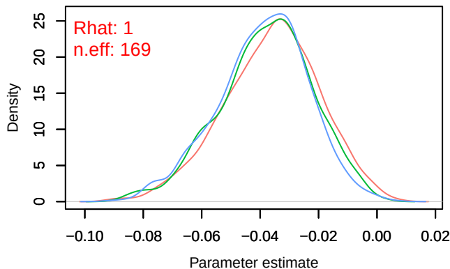
Density – B[light_pollution (C6), sp_10 (S10)]
