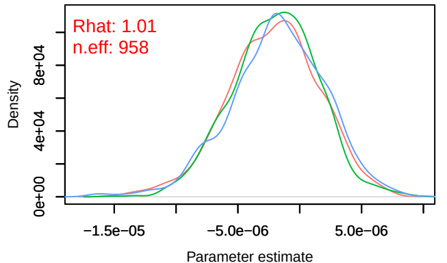
Trace – B[distance.to.water.bodies (C14), sp_27 (S27)] Density – B[distance.to.water.bodies (C14), sp_27 (S27)]
