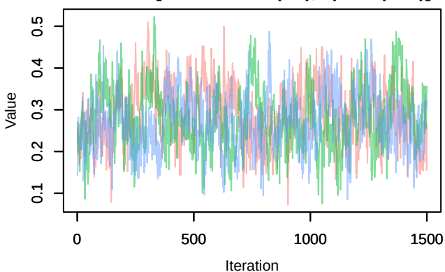
Trace – B[chelsea_hurs (C2), sp_30 (S30)]
