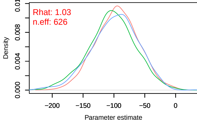
Density – B[chelsa_hurs (C2), sp_3 (S3)]
