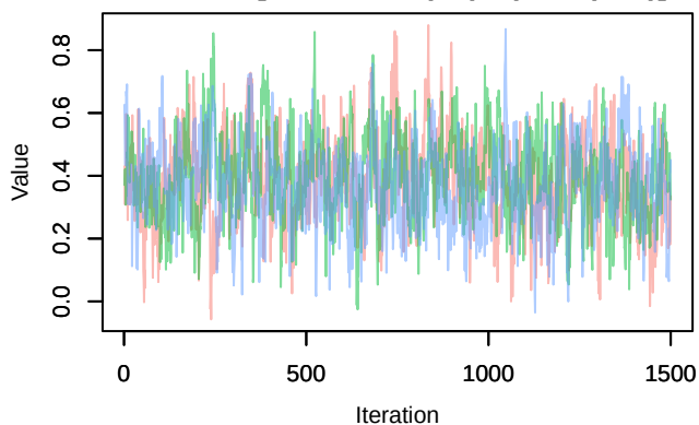
Trace – B[chelsea_tas (C4), sp_12 (S12)]
