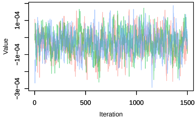
Trace – B[distance.to.wetlants (C12), sp_31 (S31]
