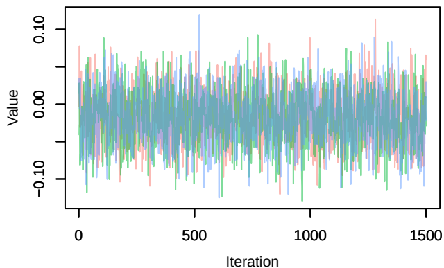
Trace – B[chelsa_hurs (C2), sp_20 (S20)]
