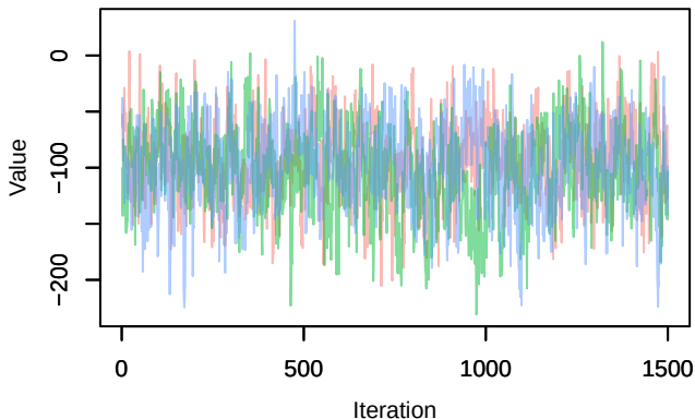
Trace – B[chelsa_hurs (C2), sp_3 (S3)]
