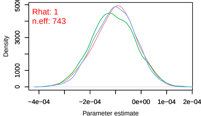
Density – B[distance.to.arable.land (C8), sp_1 (S1)
