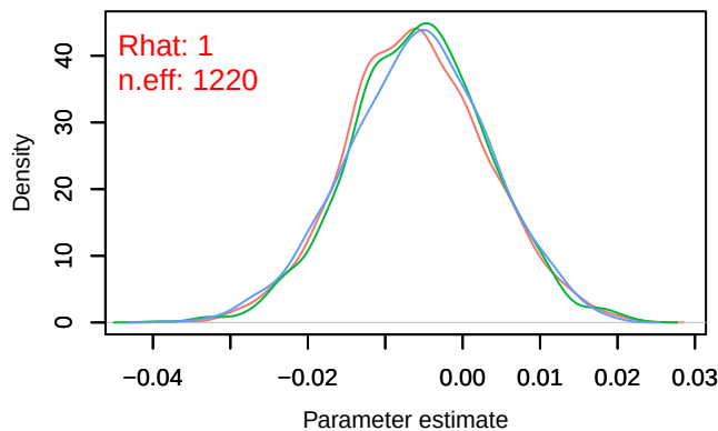
Density – B[light_pollution (C6), sp_1 (S1)]
