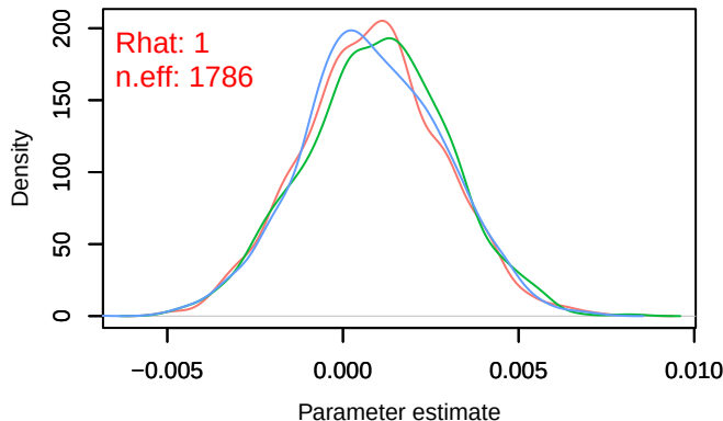
Density – B[chelsea_tas (C4), sp_35 (S35)]
