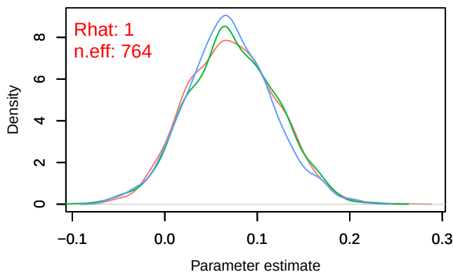
Density – B[chelsa_hurs (C2), sp_27 (S27)]
