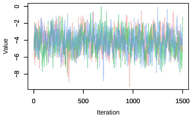
Trace – B[ndvi (C5), sp_21 (S21)]
