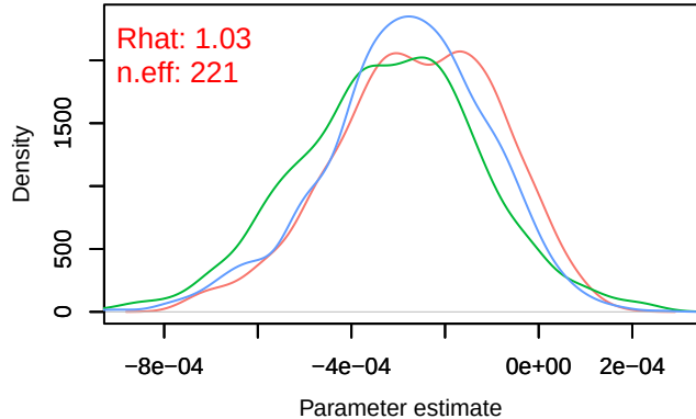
Density – B[distance.to.permanent.crops (C9), sp_2 (
