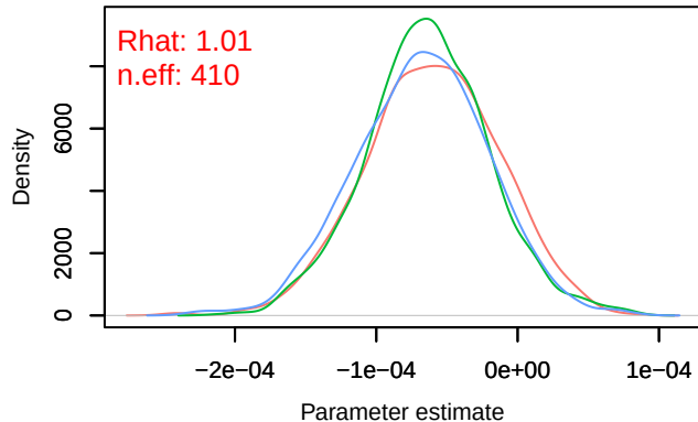
Density – B[distance.to.wetlants (C12), sp_31 (S31]
