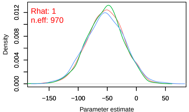
Density – B[chelsea_hurs (C2), sp_36 (S36)]
