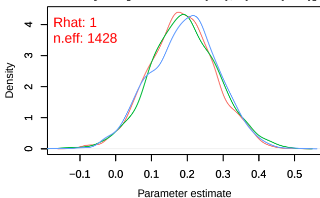
Density – B[chelsa_tas (C4), sp_32 (S32)]
