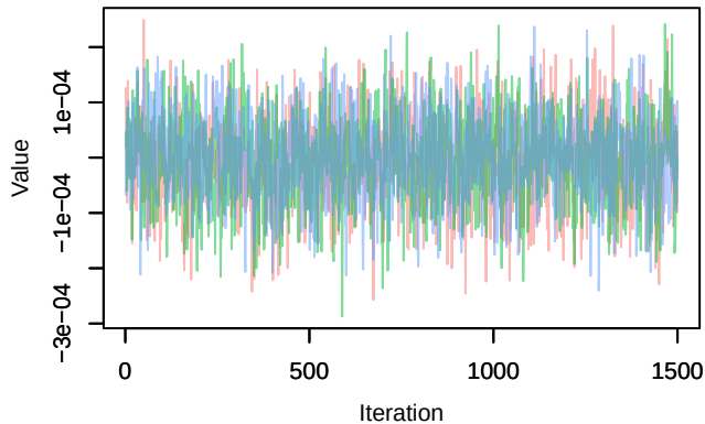
Trace – B[distance.to.water.bodies (C14), sp_9 (S9)]
