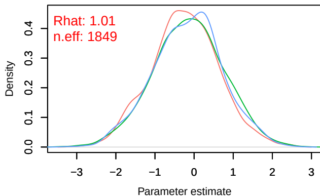
Density – B[ndvi (C5), sp_35 (S35)]
