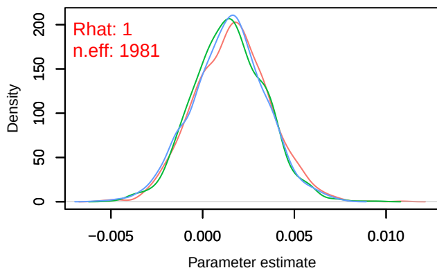
Density – B[chelsa_pr (C3), sp_20 (S20)]
