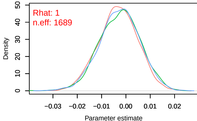
Density – B[light_pollution (C6), sp_9 (S9)]
