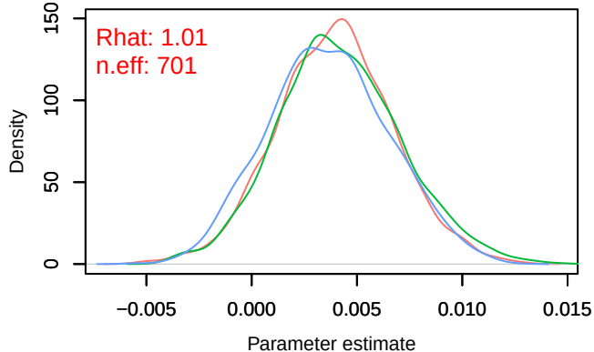
Density – B[chelsa_pr (C3), sp_3 (S3)]
