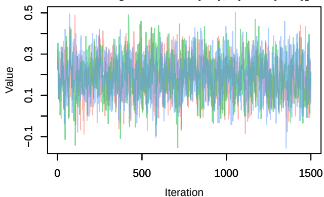
Trace – B[chelsa_tas (C4), sp_32 (S32)]
