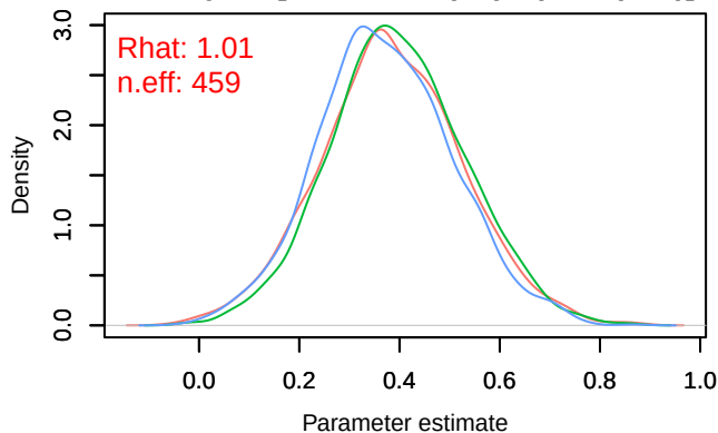
Density – B[chelsea_tas (C4), sp_12 (S12)]
