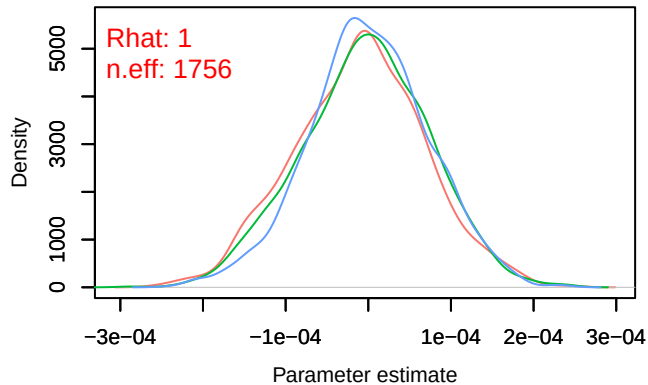
Density – B[distance.to.water.bodies (C14), sp_9 (S9)]
