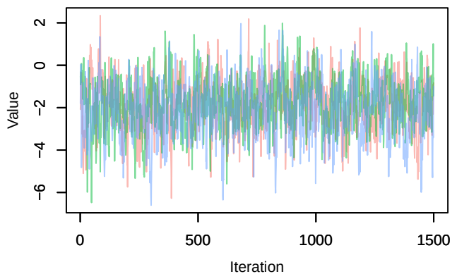
Trace – B[ndvi (C5), sp_12 (S12)]
