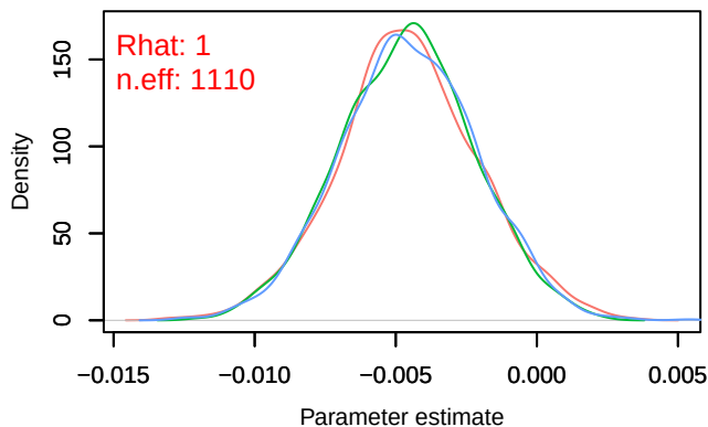
Density – B[chelsea_pr (C3), sp_21 (S21)]
