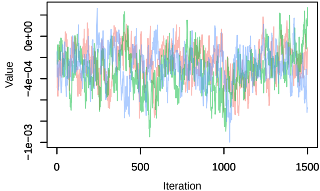
Trace – B[distance.to.permanent.crops (C9), sp_2 (
