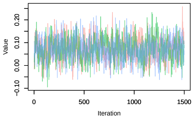
Trace – B[chelsa_hurs (C2), sp_27 (S27)]
