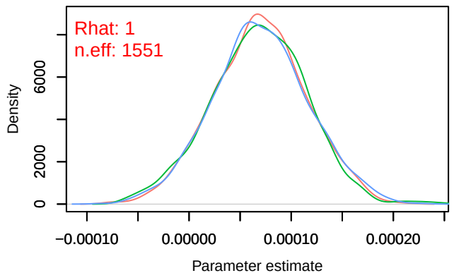
Trace – B[distance.to.heterogeneous.agricultural.areas (C11), sp_9 (S9)] Density – B[distance.to.heterogeneous.agricultural.areas (C11), sp_9 (S9)
