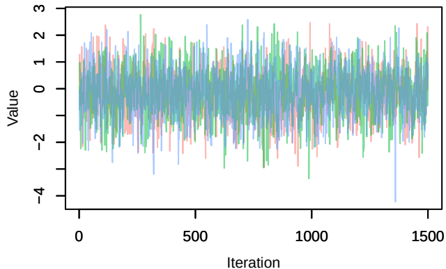
Trace – B[ndvi (C5), sp_35 (S35)]
