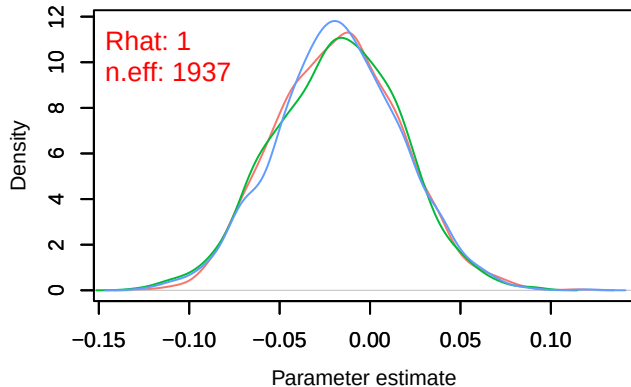
Density – B[chelsa_hurs (C2), sp_20 (S20)]
