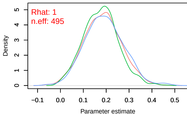
Density – B[chelsea_hurs (C2), sp_23 (S23)]
