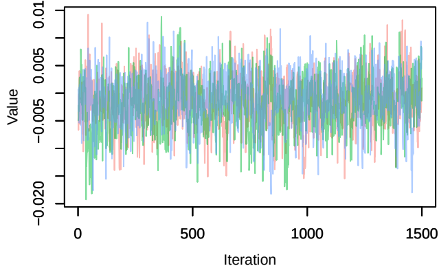
Trace – B[chelsa_pr (C3), sp_6 (S6)]
