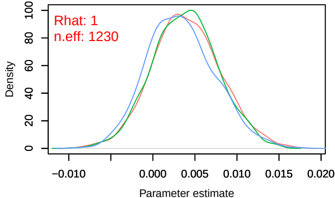
Density – B[chelsea_tas (C4), sp_9 (S9)]
