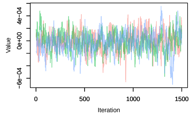
Trace – B[distance.to.arable.land (C8), sp_28 (S2 Density – B[distance.to.arable.land (C8), sp_28 (S2
