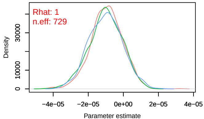
Density – B[distance.to.pastures (C10), sp_21 (S2
