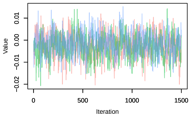
Trace – B[chelsea_pr (C3), sp_23 (S23)]
