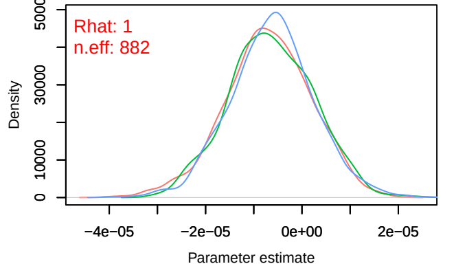
Density – B[distance.to.pastures (C10), sp_23 (S23)]
