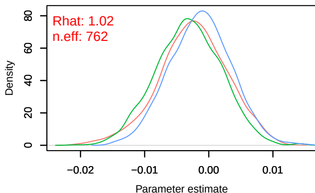
Density – B[chelsea_pr (C3), sp_23 (S23)]
