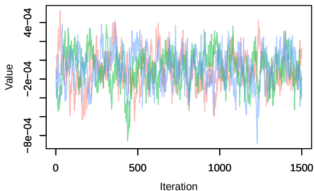
Trace – B[distance.to.arable.land (C8), sp_33 (S33
