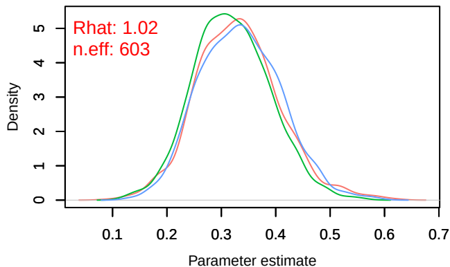
Density – B[chelsa_hurs (C2), sp_21 (S21)]
