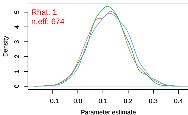
Density – B[chelsa_hurs (C2), sp_26 (S26)]
