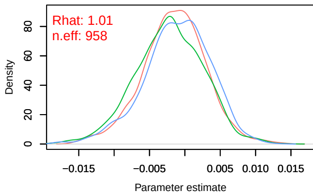
Density – B[chelsa_pr (C3), sp_6 (S6)]
