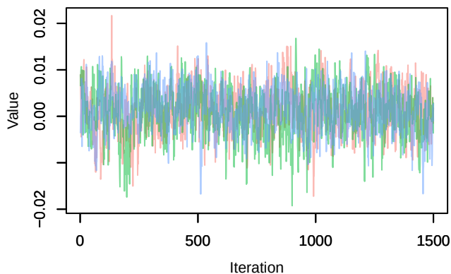
Trace – B[chelsea_pr (C3), sp_1 (S1)]
