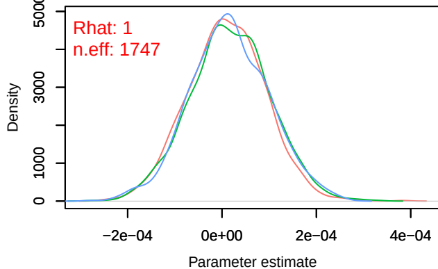
Density – B[distance.to.artificial.surfaces (C7), sp_20 (S20)]
