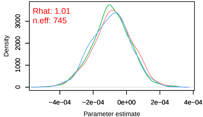
Trace – B[distance.to.permanent.crops (C9), sp_23 (S23)]
