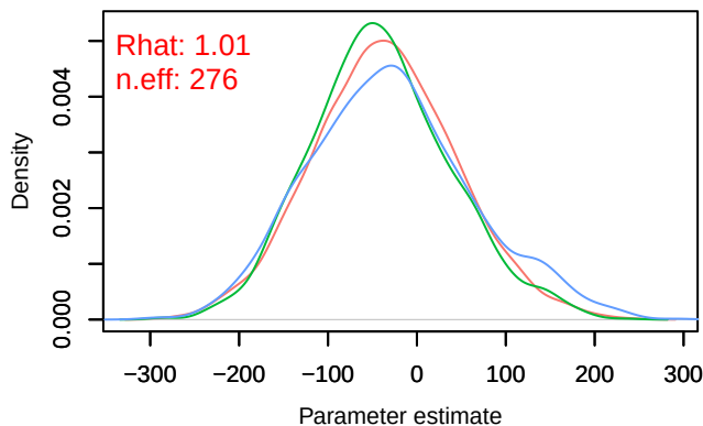
Density – B[(Intercept) (C1), sp_10 (S10)]
