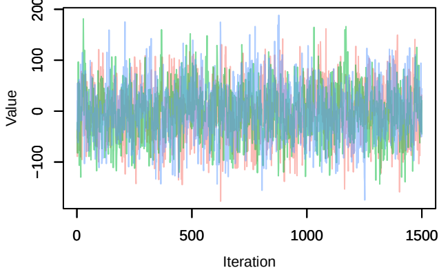
Trace – B[(Intercept) (C1), sp_9 (S9)]
