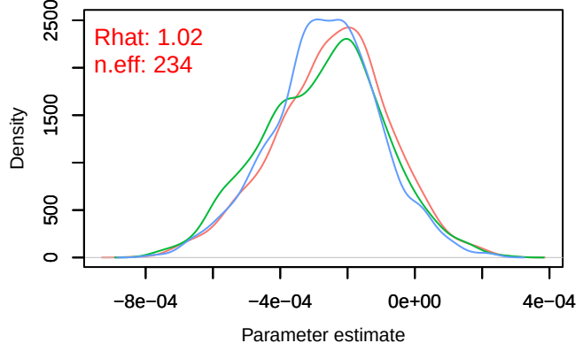
Trace – B[distance.to.arable.land (C8), sp_28 (S2 Density – B[distance.to.arable.land (C8), sp_28 (S2
