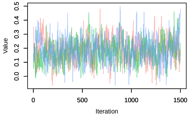
Trace – B[chelsea_hurs (C2), sp_23 (S23)]
