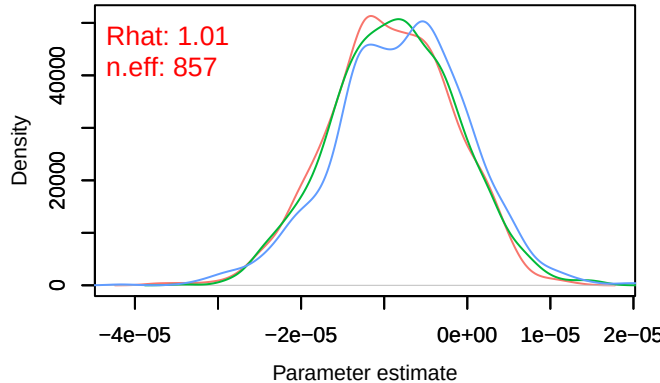
Trace – B[distance.to.permanent.crops (C9), sp_6 ( Density – B[distance.to.permanent.crops (C9), sp_6
