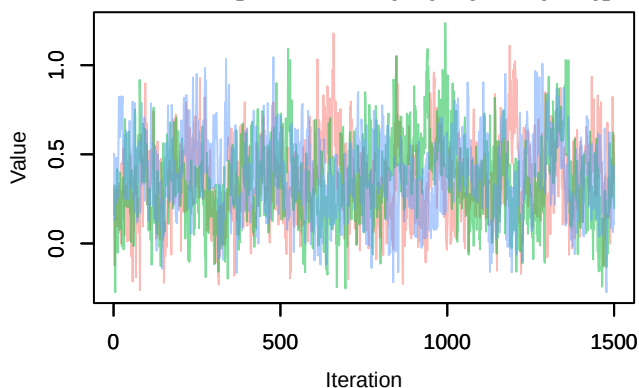
Trace – B[chelsea_tas (C4), sp_30 (S30)]
