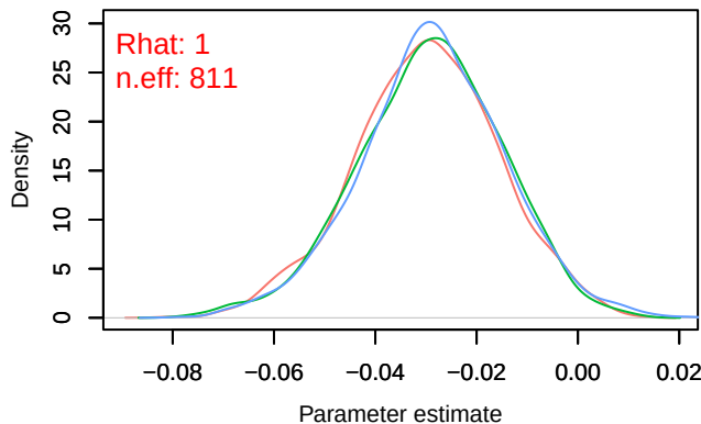
Density – B[light_pollution (C6), sp_19 (S19)]
