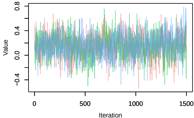
Trace – B[chelsa_tas (C4), sp_24 (S24)]
