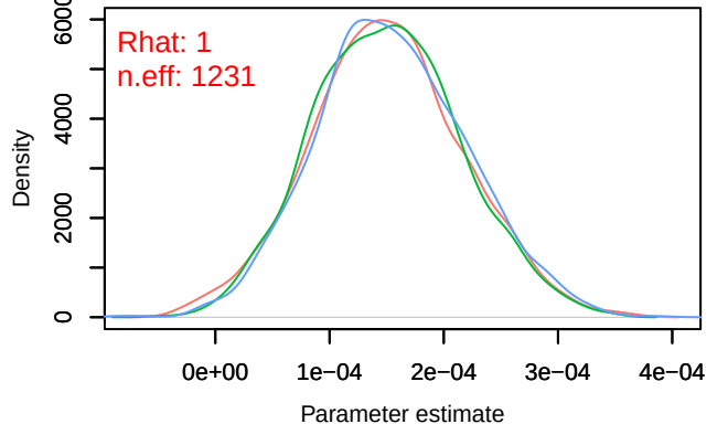
Trace – B[distance.to.heterogeneous.agricultural.areas (C11), sp_6 (S6)] Density – B[distance.to.heterogeneous.agricultural.areas (C11), sp_6 (S6)]
