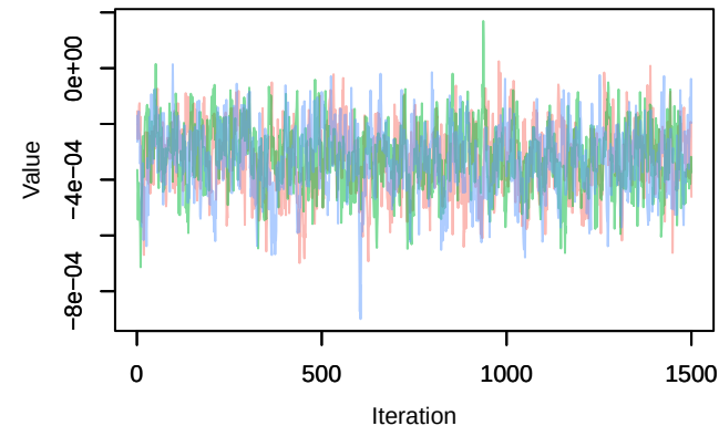
Trace – B[distance.to.permanent.crops (C9), sp_13 (Density – B[distance.to.permanent.crops (C9), sp_13
