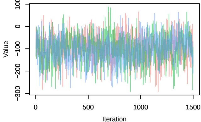
Trace – B[(Intercept) (C1), sp_6 (S6)]
