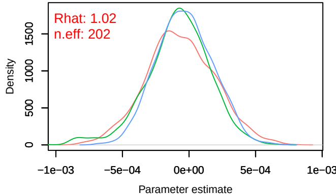
Density – B[(Intercept) (C1), sp_3 (S3)]
