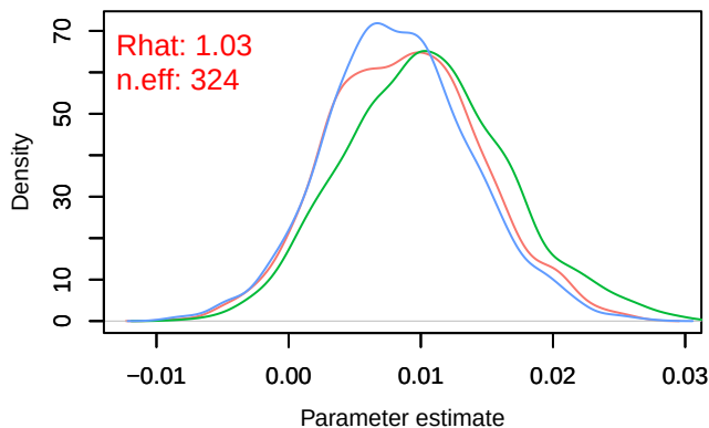
Density – B[chelsea_pr (C3), sp_15 (S15)]
