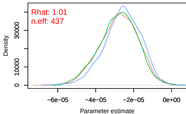
Trace – B[distance.to.permanent.crops (C9), sp_12 (Density – B[distance.to.permanent.crops (C9), sp_12
