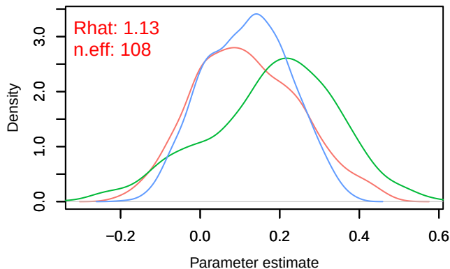
Density – B[chelsa_hurs (C2), sp_33 (S33)]
