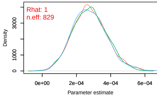
Trace – B[distance.to.arable.land (C8), sp_13 (S1: Density – B[distance.to.arable.land (C8), sp_13 (S1:
