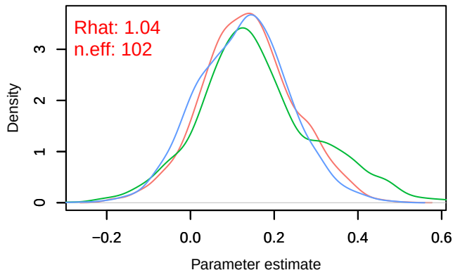
Density – B[chelsa_pr (C3), sp_10 (S10)]
