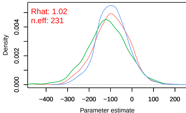
Density – B[chelsa_hurs (C2), sp_10 (S10)]
