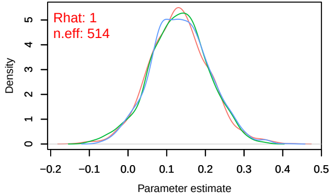
Density – B[chelsea_pr (C3), sp_17 (S17)]
