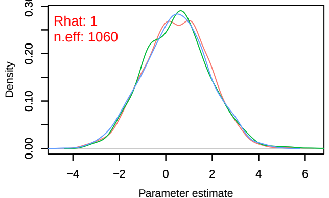
Density – B[ndvi (C5), sp_24 (S24)]
