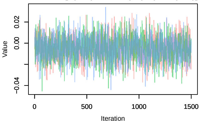
Trace – B[light_pollution (C6), sp_20 (S20)]
