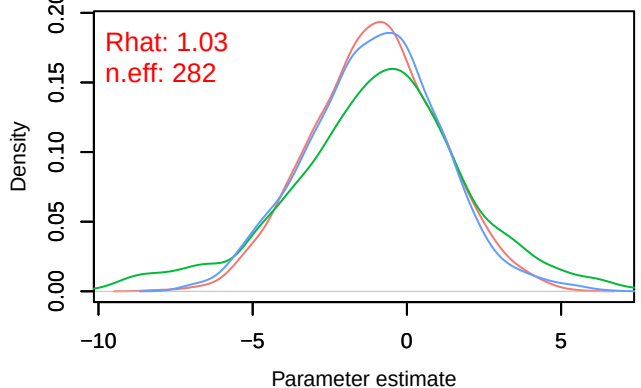
Density – B[ndvi (C5), sp_15 (S15)]
