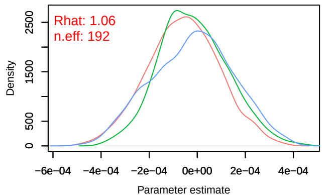
Density – B[distance.to.wetlands (C12), sp_2 (S2)]
