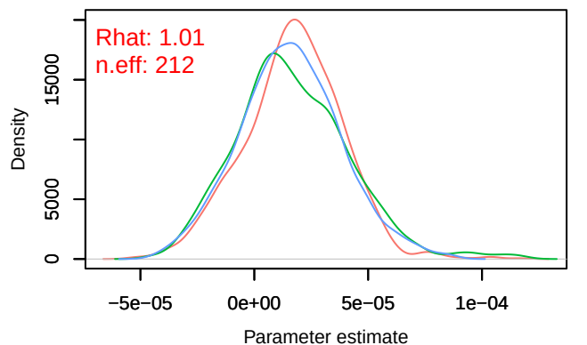
Trace – B[distance.to forest and semi.natural areas (C13), ty – B[distance.to forest and semi.natural areas (C13)]
