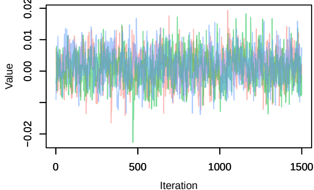
Trace – B[chelsa_pr (C3), sp_21 (S21)]
