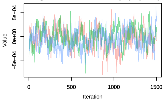
Trace – B[distance.to.arable.land (C8), sp_33 (S3:
