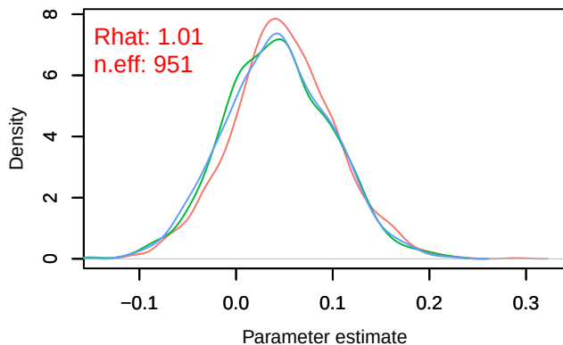
Density – B[chelsa_hurs (C2), sp_14 (S14)]
