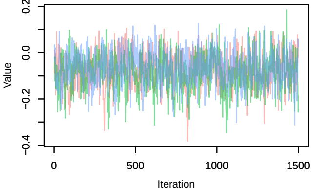
Trace – B[chelsea_hurs (C2), sp_39 (S39)]
