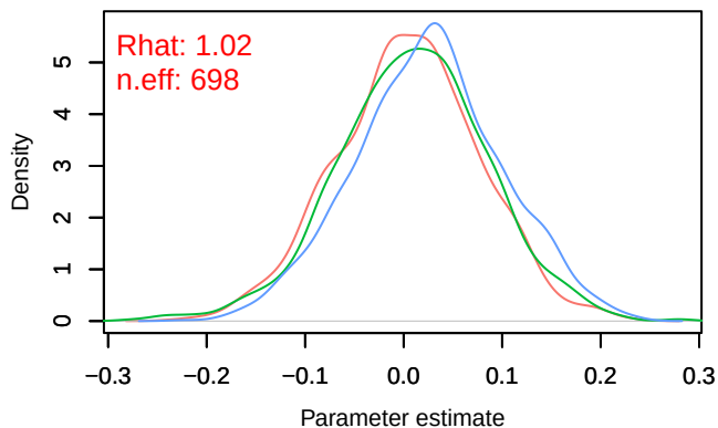
Density – B[chelsea_hurs (C2), sp_24 (S24)]
