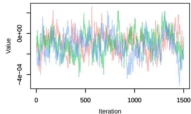
Trace – B[distance.to forest and semi.natural areas (C13), ty – B[distance.to forest and semi.natural areas (C13)]
