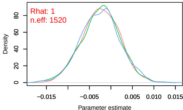
Density – B[chelsa_tas (C4), sp_35 (S35)]
