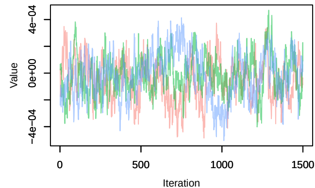
Trace – B[distance.to.wetlands (C12), sp_2 (S2)]
