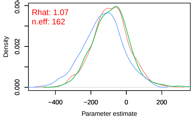
Density – B[(Intercept) (C1), sp_15 (S15)]
