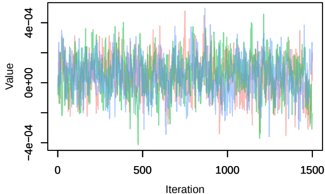
Trace – B[distance.to.permanent.crops (C9), sp_26 (S26) Density – B[distance.to.permanent.crops (C9), sp_26 (S26)
