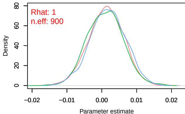
Density – B[chelsa_pr (C3), sp_21 (S21)]
