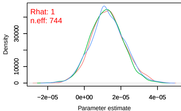
Density – B[distance.to.pastures (C10), sp_18 (S18
