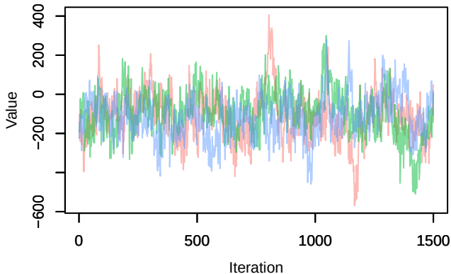
Trace – B[(Intercept) (C1), sp_16 (S16)]
