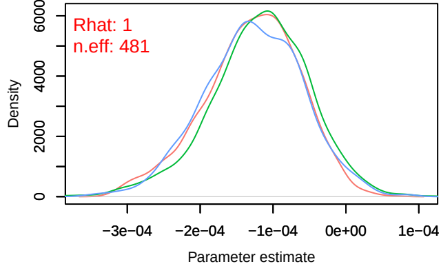
– B[distance.to.forest.and.semi.natural.areas (C13), \gamma – B[distance.to.forest.and.semi.natural.areas (C13),
