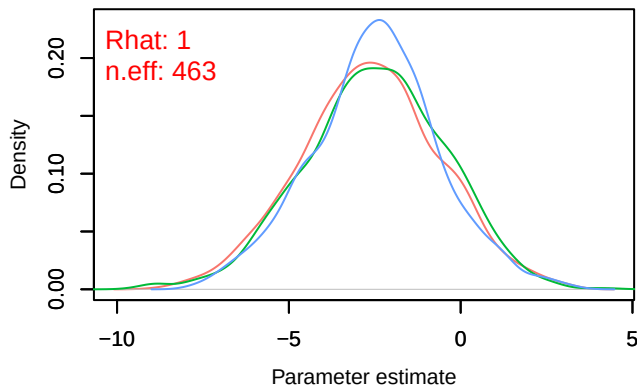
Density – B[ndvi (C5), sp_3 (S3)]
