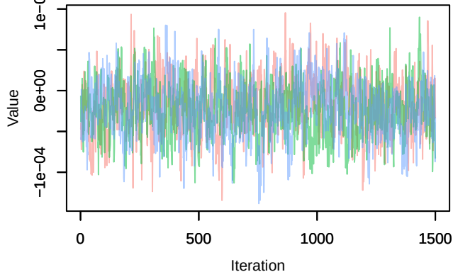
Trace – B[distance.to.pastures (C10), sp_26 (S26) Density – B[distance.to.pastures (C10), sp_26 (S26)
