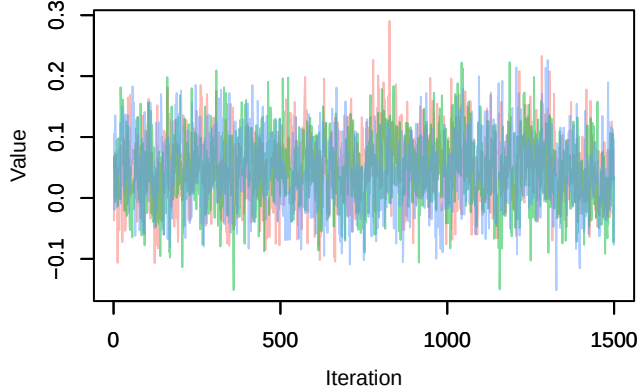
Trace – B[chelsa_hurs (C2), sp_14 (S14)]
