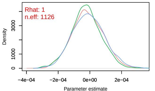
Trace – B[distance.to.arable.land (C8), sp_21 (S2: Density – B[distance.to.arable.land (C8), sp_21 (S2
