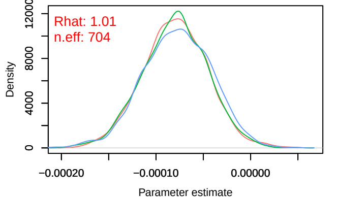
Density – B[distance.to.pastures (C10), sp_12 (S1
