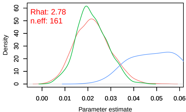
Density – B[chelsa_pr (C3), sp_18 (S18)]
