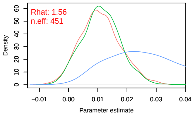
Density – B[chelsa_pr (C3), sp_27 (S27)]
