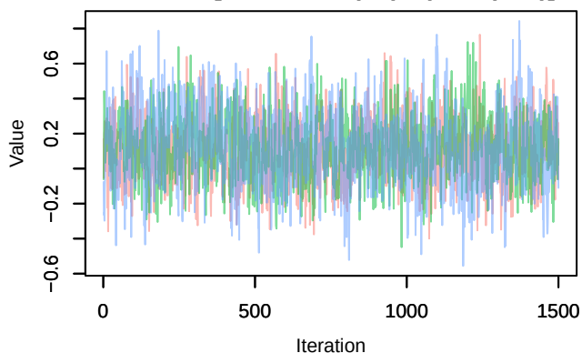
Trace – B[chelsa_tas (C4), sp_12 (S12)]
