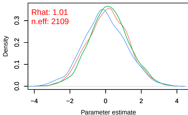
Density – B[ndvi (C5), sp_14 (S14)]
