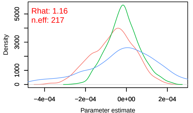
Density – B[distance.to.wetlants (C12), sp_40 (S40
