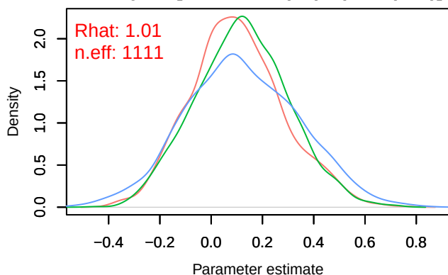
Density – B[chelsa_tas (C4), sp_12 (S12)]
