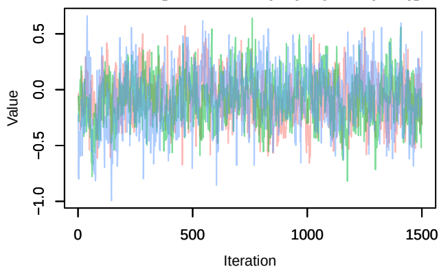
Trace – B[chelsa_tas (C4), sp_18 (S18)]
