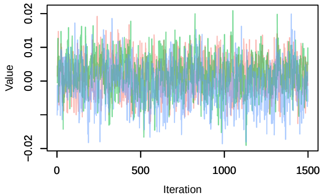
Trace – B[chelsa_pr (C3), sp_12 (S12)]
