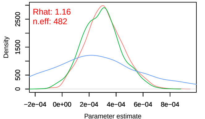
Trace – B[distance.to.water.bodies (C14), sp_30 (S30)] Density – B[distance.to.water.bodies (C14), sp_30 (S30)]
