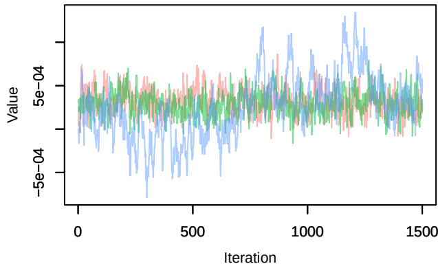
Trace – B[distance.to.water.bodies (C14), sp_30 (S30)] Density – B[distance.to.water.bodies (C14), sp_30 (S30)]
