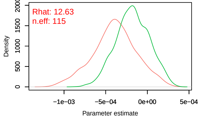
Trace – B[distance.to.permanent.crops (C9), sp_22 (Density – B[distance.to.permanent.crops (C9), sp_22
