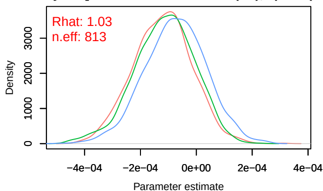
Density – B[distance.to.arable.land (C8), sp_24 (S24)]
