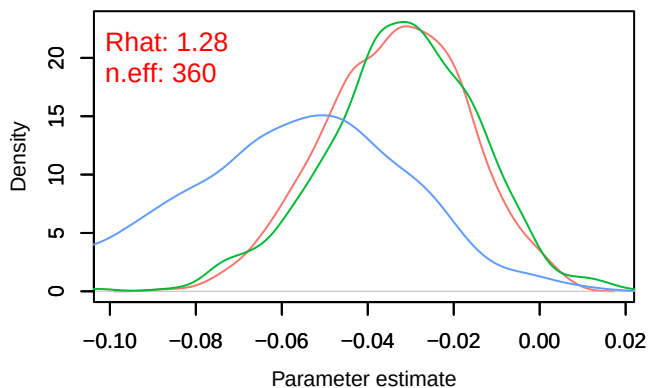
Density – B[light_pollution (C6), sp_31 (S31)]
