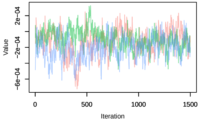
Trace – B[distance.to.wetlants (C12), sp_40 (S40
