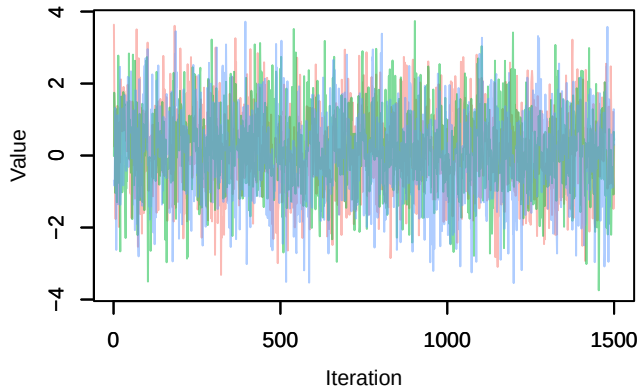
Trace – B[ndvi (C5), sp_14 (S14)]
