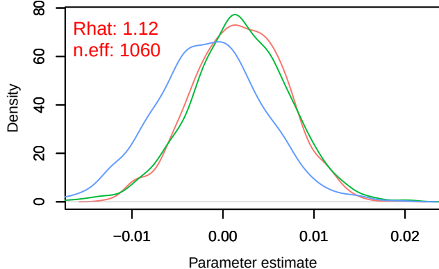
Density – B[chelsa_pr (C3), sp_12 (S12)]
