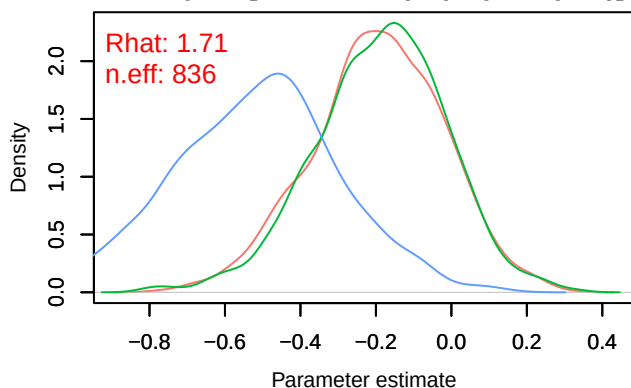
Density – B[chelsa_tas (C4), sp_39 (S39)]
