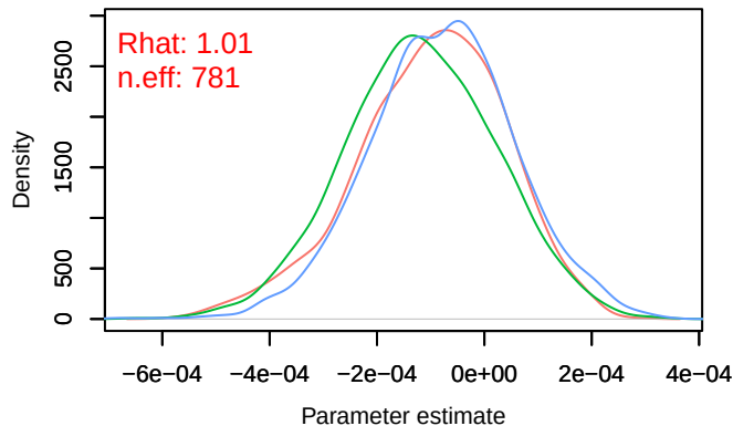
Density – B[(Intercept) (C1), sp_12 (S12)]
