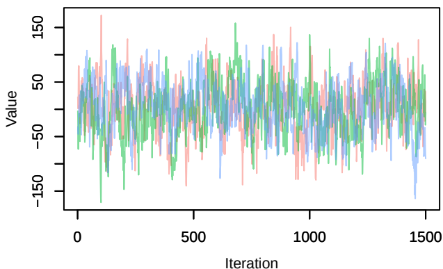
Trace – B[(Intercept) (C1), sp_33 (S33)]
