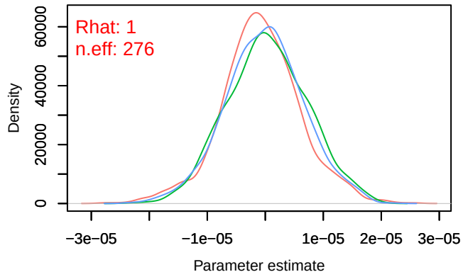
Trace – B[distance.to.permanent.crops (C9), sp_4 ( Density – B[distance.to.permanent.crops (C9), sp_4
