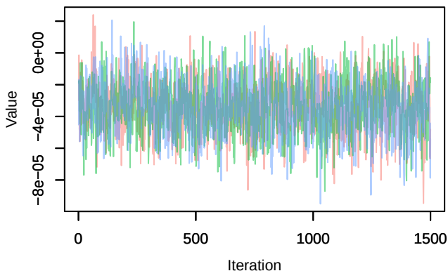
Trace – B[distance.to.heterogeneous.agricultural.areas (C11), sp_6 (S6)]
