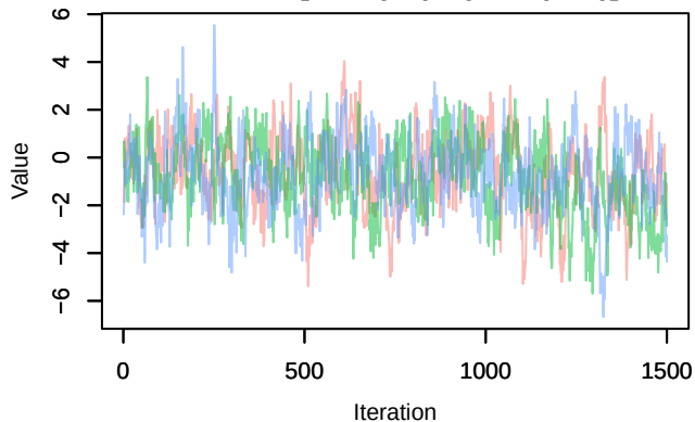
Trace – B[light_pollution (C6), sp_29 (S29)]
