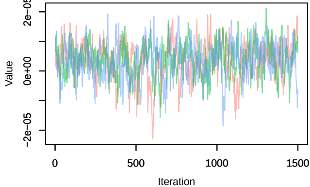
Trace – B[distance.to.water.bodies (C14), sp_33 (S33)]
