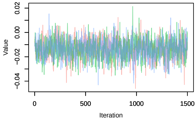
Trace – B[light_pollution (C6), sp_6 (S6)]
