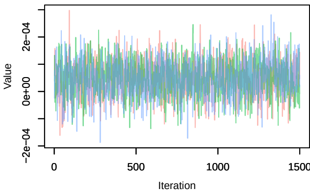
Trace – B[distance.to.arable.land (C8), sp_25 (S2: Density – B[distance.to.arable.land (C8), sp_25 (S2:
