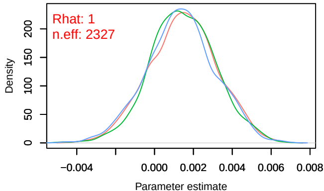
Density – B[chelsea_tas (C4), sp_38 (S38)]
