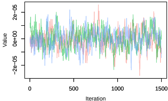
Trace – B[distance.to.permanent.crops (C9), sp_4 ( Density – B[distance.to.permanent.crops (C9), sp_4
