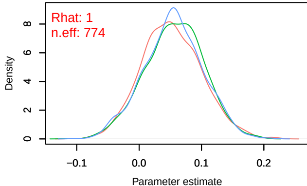
Density – B[chelsea_pr (C3), sp_26 (S26)]
