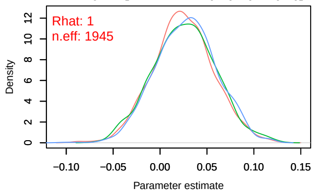
Density – B[chelsea_hurs (C2), sp_7 (S7)]
