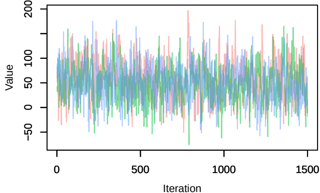
Trace – B[(Intercept) (C1), sp_16 (S16)]
