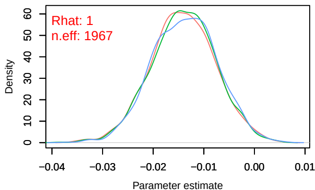
Density – B[light_pollution (C6), sp_7 (S7)]
