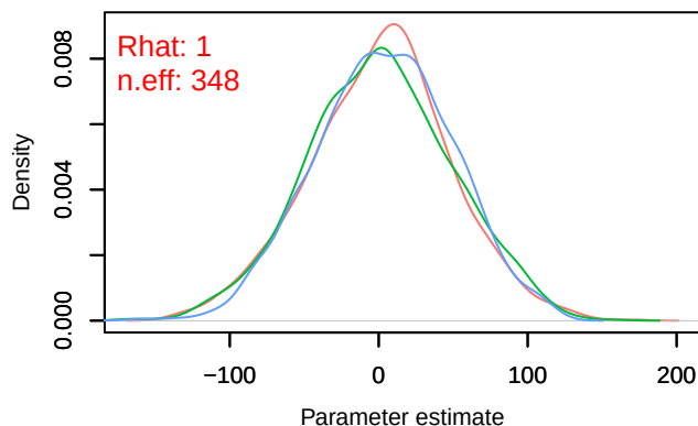
Density – B[(Intercept) (C1), sp_33 (S33)]
