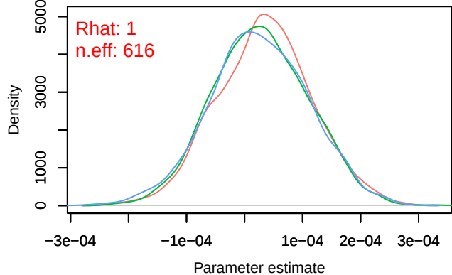
Trace – B[distance.to.water.bodies (C14), sp_27 (S27) Density – B[distance.to.water.bodies (C14), sp_27 (S27)
