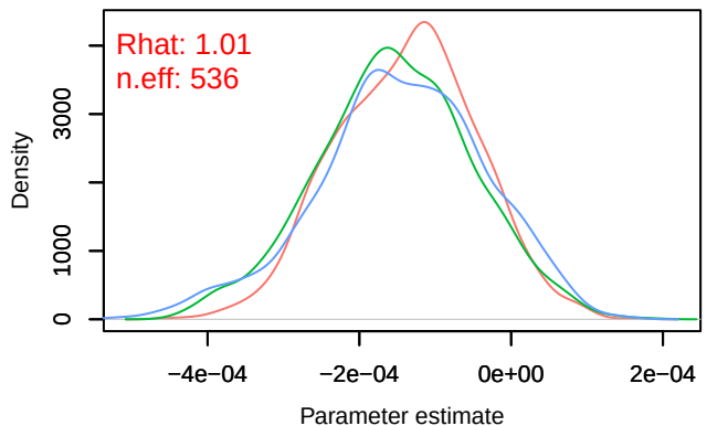
Trace – B[distance.to.arable.land (C8), sp_30 (S30) Density – B[distance.to.arable.land (C8), sp_30 (S30)]
