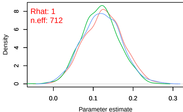
Density – B[chelsa_pr (C3), sp_23 (S23)]
