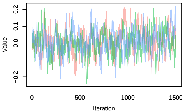
Trace – B[chelsea_hurs (C2), sp_33 (S33)]
