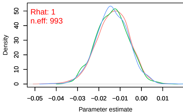
Density – B[light_pollution (C6), sp_6 (S6)]
