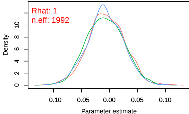
Density – B[chelsea_pr (C3), sp_38 (S38)]
