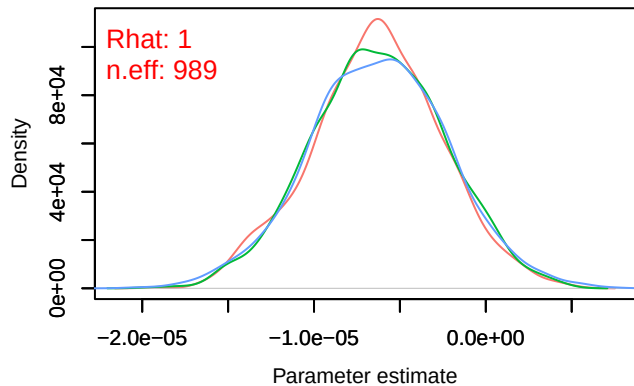
Density – B[distance.to.pastures (C10), sp_39 (S3
