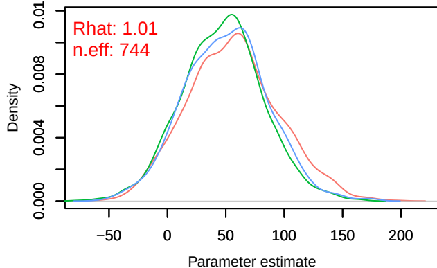
Density – B[(Intercept) (C1), sp_16 (S16)]
