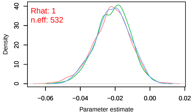
Trace – B[distance.to.artificial.surfaces (C7), sp_30 (Density – B[distance.to.artificial.surfaces (C7), sp_30
