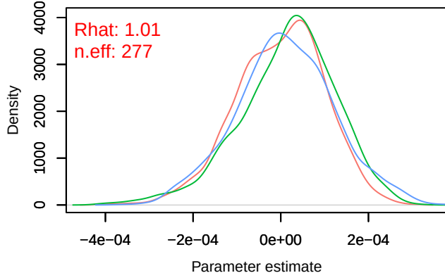
Density – B[distance.to.artificial.surfaces (C7), sp_29 (S29)]
