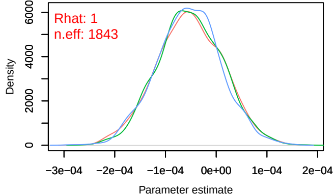
Density – B[distance.to.permanent.crops (C9), sp_35 (S35)]
