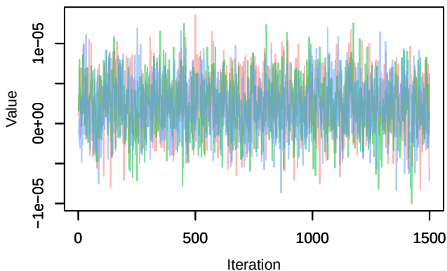
Trace – B[distance.to.pastures (C10), sp_32 (S32
