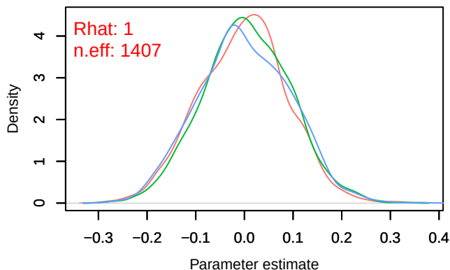
Density – B[ndvi (C5), sp_39 (S39)]
