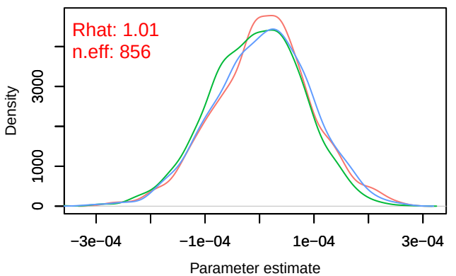
Trace – B[distance.to.permanent.crops (C9), sp_25 (Density – B[distance.to.permanent.crops (C9), sp_25
