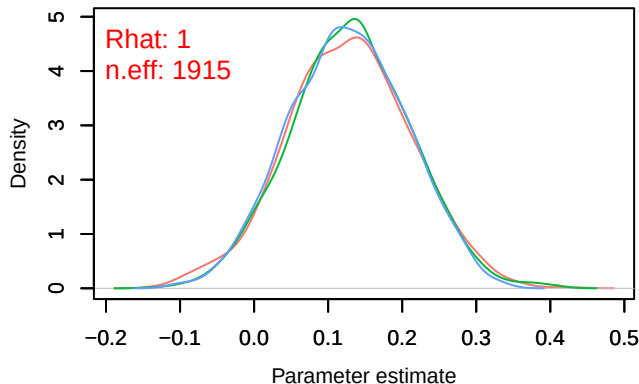
Density – B[ndvi (C5), sp_9 (S9)]
