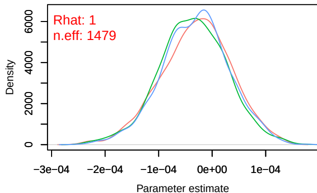
Density – B[distance.to.water.bodies (C14), sp_9 (S9)]
