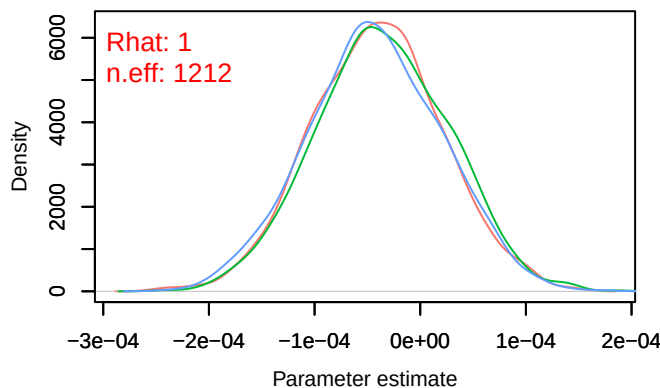
Trace – B[distance.to.artificial.surfaces (C7), sp_18 (Density – B[distance.to.artificial.surfaces (C7), sp_18
