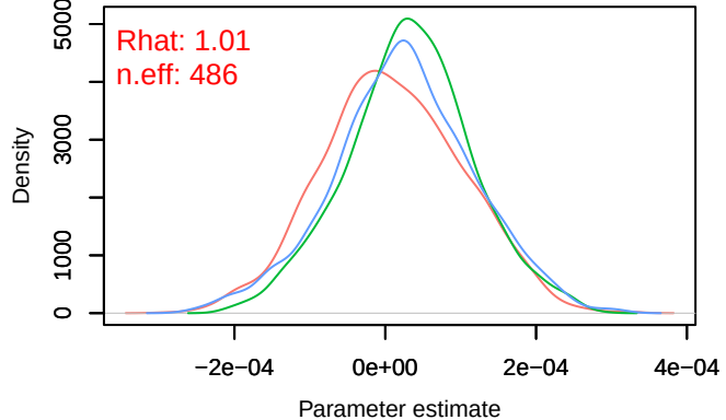
Density – B[distance.to.arable.land (C8), sp_4 (S4)
