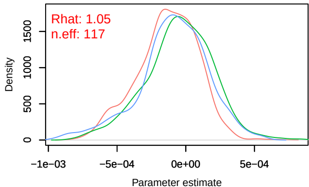
Density – B[(Intercept) (C1), sp_30 (S30)]
