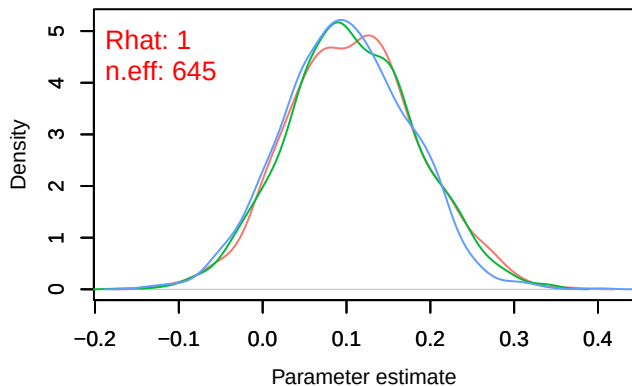
Density – B[chelsa_hurs (C2), sp_27 (S27)]
