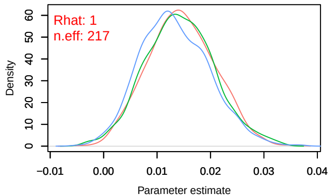
Density – B[chelsa_pr (C3), sp_4 (S4)]
