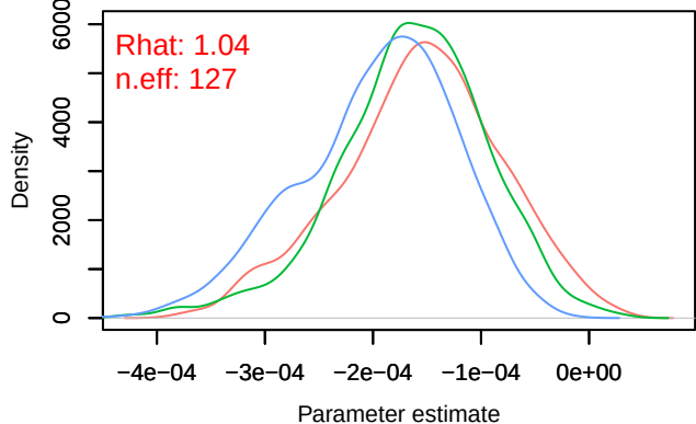
Density – B[distance.to.wetlands (C12), sp_3 (S3)]
