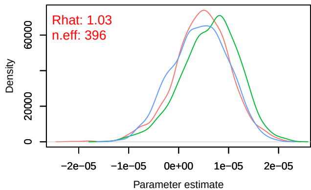
– B[distance.to.forest.and.semi.natural.areas (C13), sy – B[distance.to.forest.and.semi.natural.areas (C13),
