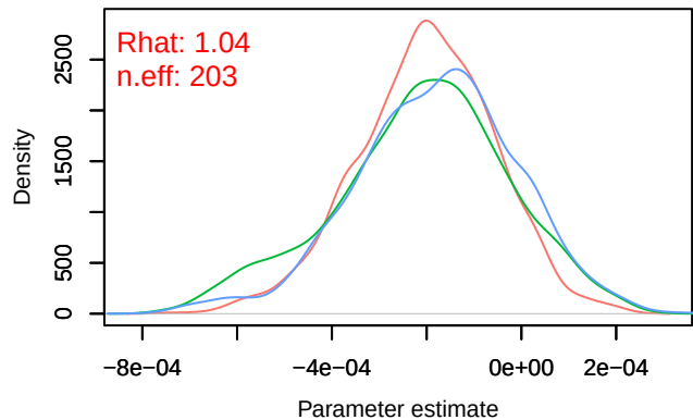
Trace – B[distance.to.arable.land (C8), sp_16 (S16) (Density – B[distance.to.arable.land (C8), sp_16 (S16)
