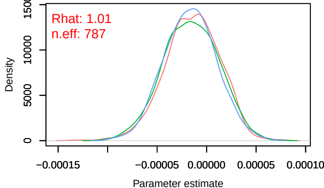
Density – B[distance.to.pastures (C10), sp_11 (S11)]
