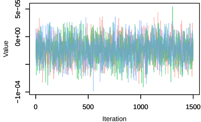
Trace – B[distance.to.pastures (C10), sp_38 (S38)]
