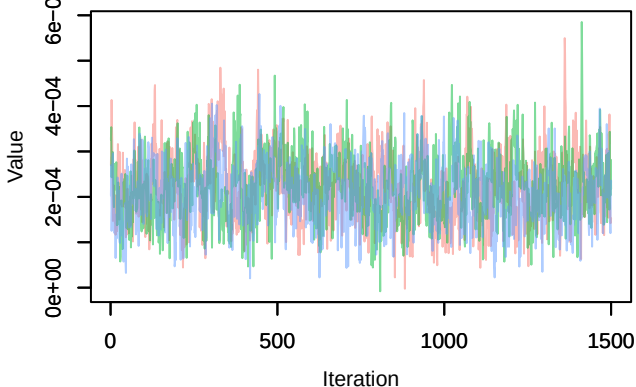
Trace – B[distance.to.heterogeneous.agricultural.areas (C11), sp_1 (S1)]
