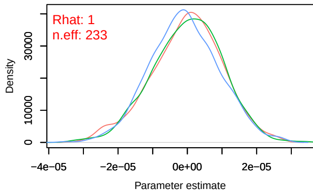
Density – B[distance.to.permanent.crops (C9), sp_4 (
