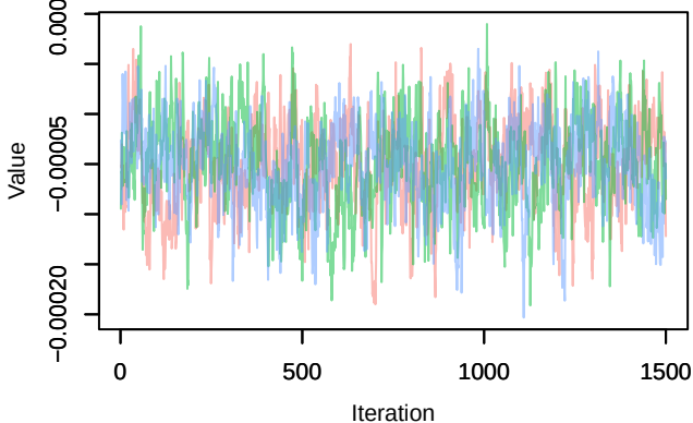
Trace – B[distance.to.wetlands (C12), sp_1 (S1)]
