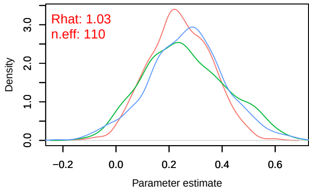
Density – B[chelsa_pr (C3), sp_16 (S16)]
