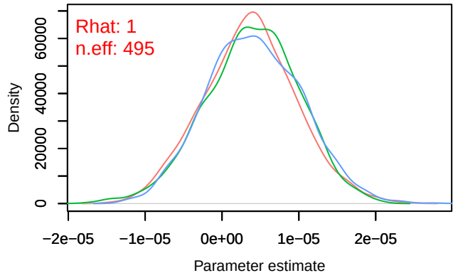
Trace – B[distance.to.permanent.crops (C9), sp_30 (Density – B[distance.to.permanent.crops (C9), sp_30
