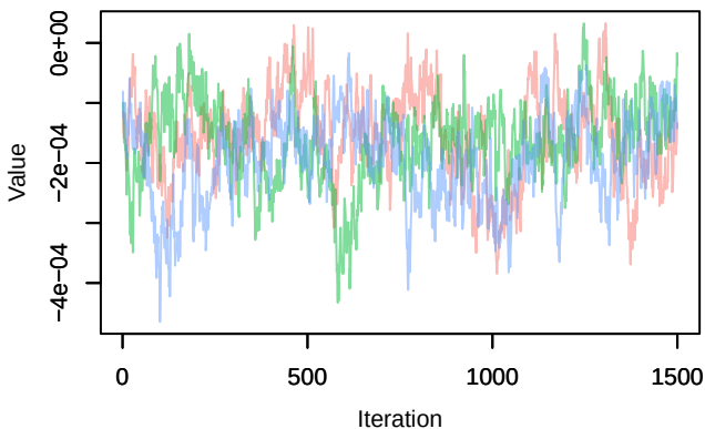
Trace – B[distance.to.wetlands (C12), sp_3 (S3)]
