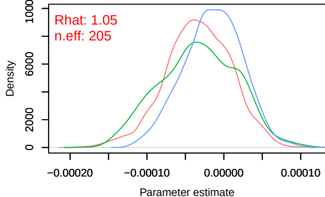
Trace – B[distance.to.heterogeneous.agricultural.areas (C11), sp_4 (S4)]
