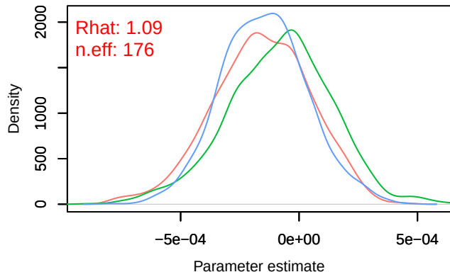
Density – B[distance.to.permanent.crops (C9), sp_4 (
