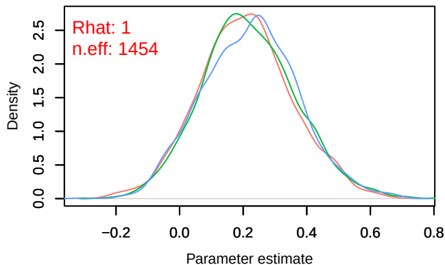
Density – B[chelsea_tas (C4), sp_32 (S32)]
