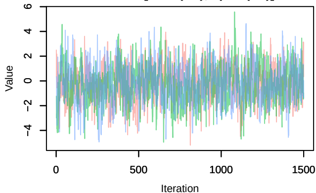
Trace – B[light_pollution (C6), sp_8 (S8)]
