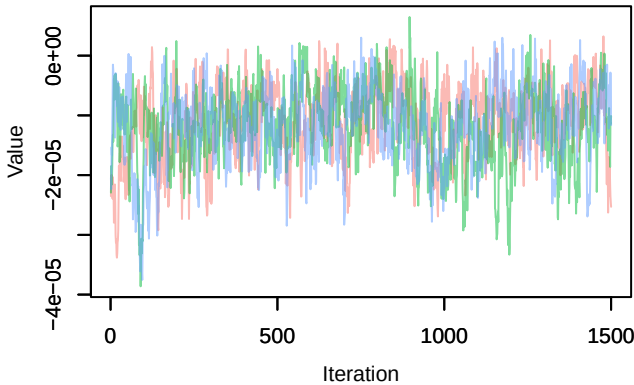
Trace – B[distance.to.water.bodies (C14), sp_12 (S12)] Density – B[distance.to.water.bodies (C14), sp_12 (S12)]
