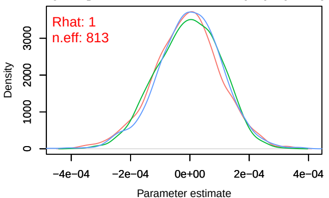
Density – B[distance.to.arable.land (C8), sp_25 (S2:
