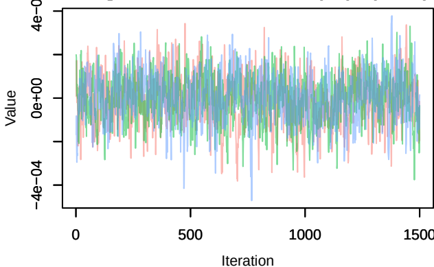
Trace – B[distance.to.arable.land (C8), sp_25 (S2:
