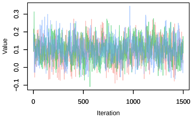
Trace – B[chelsea_hurs (C2), sp_12 (S12)]
