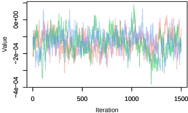
Trace – B[distance.to.forest.and.semi.natural.areas (C13), sp_36 (S36)]
