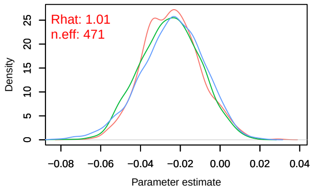
Density – B[light_pollution (C6), sp_25 (S25)]
