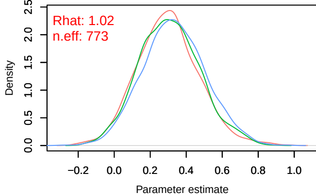
Density – B[chelsea_tas (C4), sp_1 (S1)]
