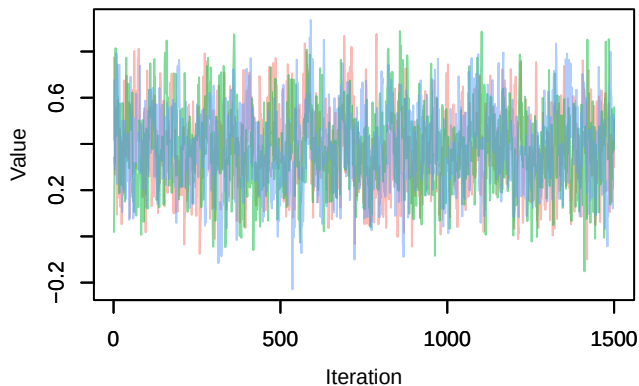
Trace – B[chelsea_tas (C4), sp_5 (S5)]
