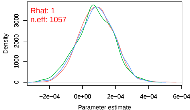
Density – B[(Intercept) (C1), sp_18 (S18)]
