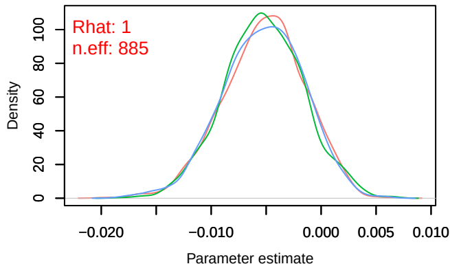
Density – B[chelsea_tas (C4), sp_5 (S5)]
