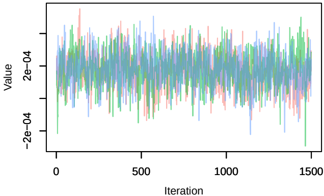
Trace – B[distance.to.water.bodies (C14), sp_21 (S21]
