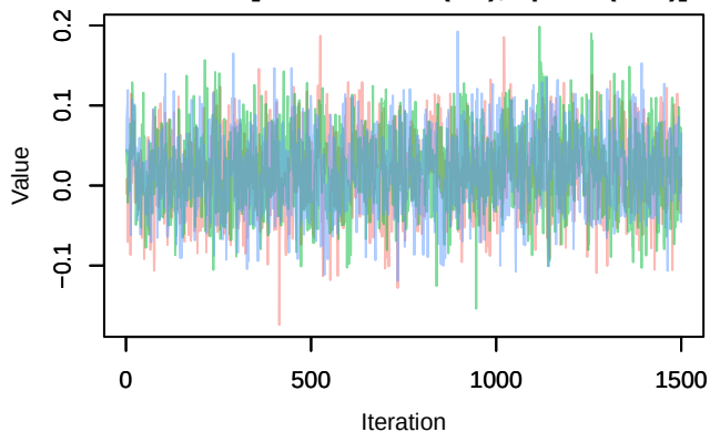
Trace – B[chelsea_pr (C3), sp_14 (S14)]
