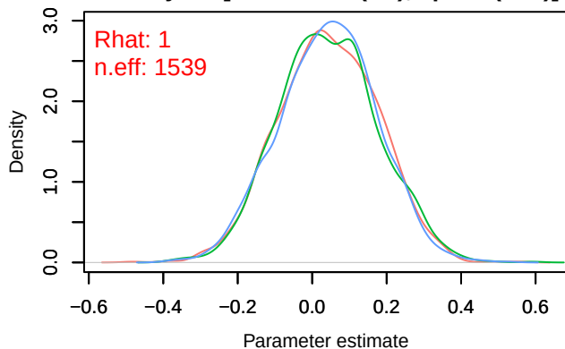
Density – B[chelsea_tas (C4), sp_14 (S14)]
