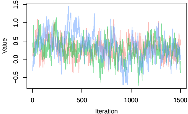
Trace – B[chelsea_tas (C4), sp_4 (S4)]
