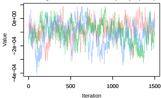
Trace – B[distance.to.wetlands (C12), sp_4 (S4)]
