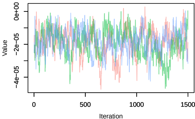
Trace – B[distance.to.forest.and.semi.natural.areas (C13), sp_36 (S36)]
