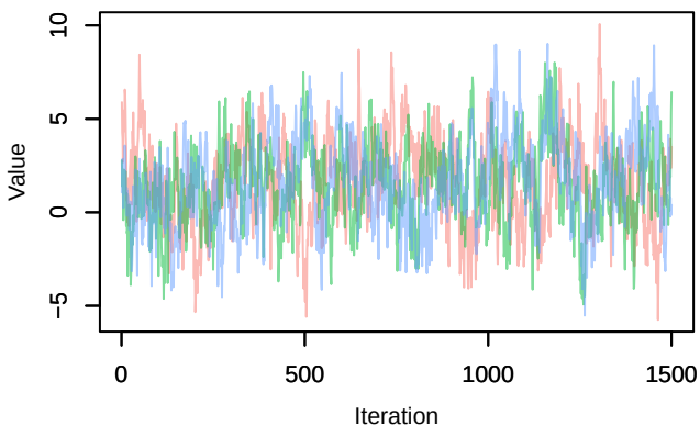
Trace – B[ndvi (C5), sp_4 (S4)]
