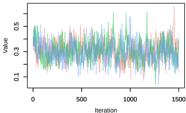
Trace – B[chelsea_hurs (C2), sp_19 (S19)]
