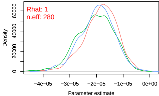
Density – B[distance.to.water.bodies (C14), sp_21 (S21]
