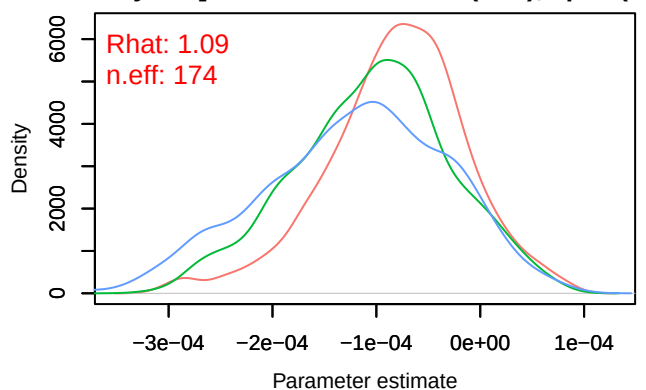
Density – B[distance.to.wetlands (C12), sp_4 (S4)]
