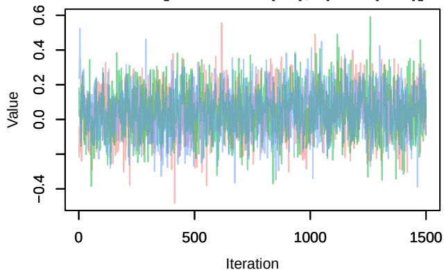
Trace – B[chelsea_tas (C4), sp_14 (S14)]
