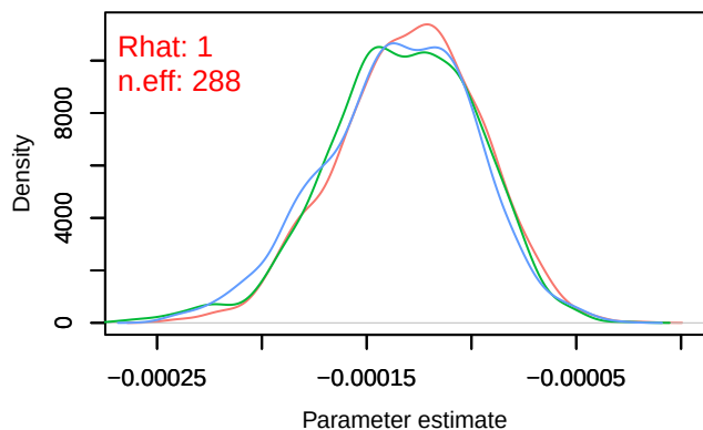
Density – B[distance.to.pastures (C10), sp_21 (S2
