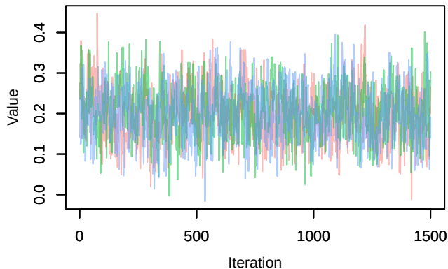
Trace – B[chelsea_pr (C3), sp_5 (S5)]
