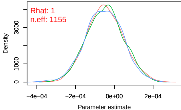
Density – B[distance.to.permanent.crops (C9), sp_5 (S5)]
