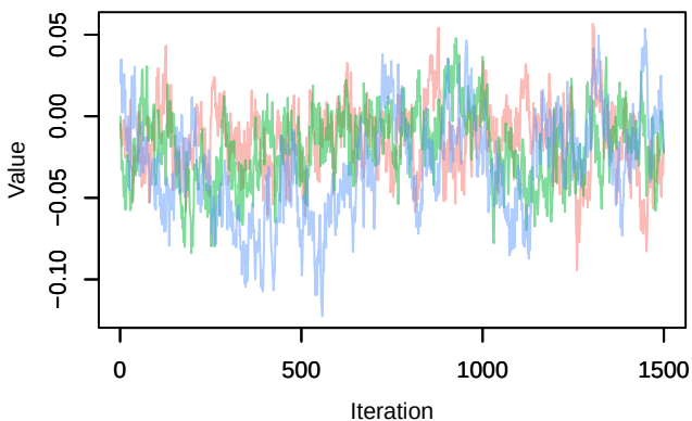
Trace – B[light_pollution (C6), sp_4 (S4)]
