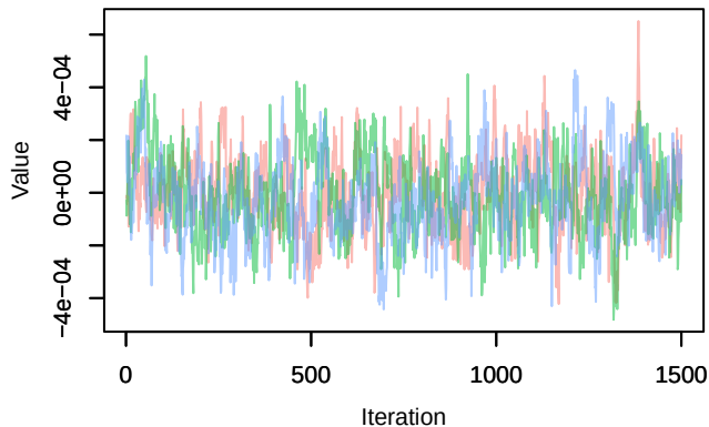
Trace – B[distance.to.arable.land (C8), sp_15 (S1
