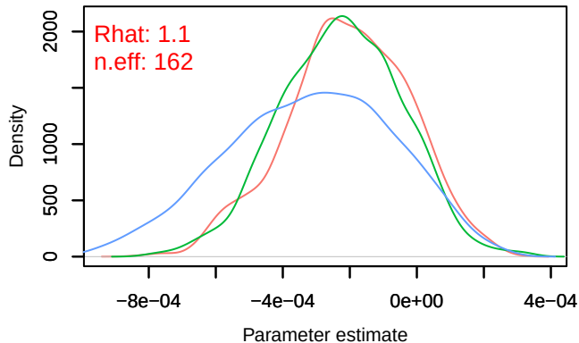
Density – B[distance.to.arable.land (C8), sp_15 (S1
