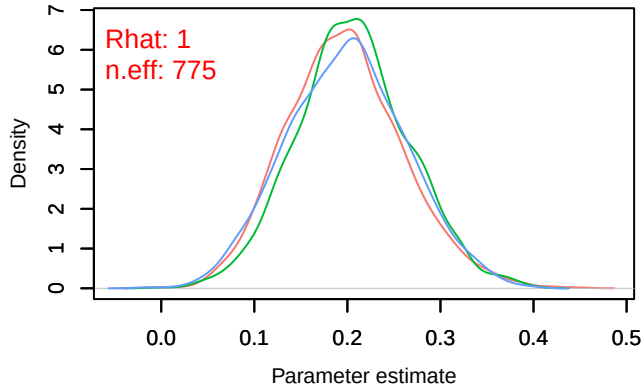
Density – B[chelsea_pr (C3), sp_5 (S5)]
