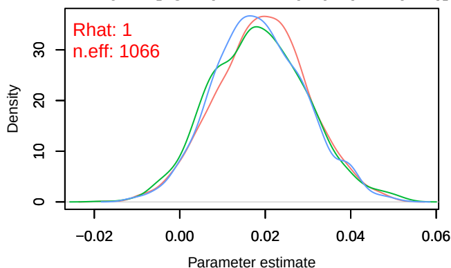
Density – B[light_pollution (C6), sp_11 (S11)]
