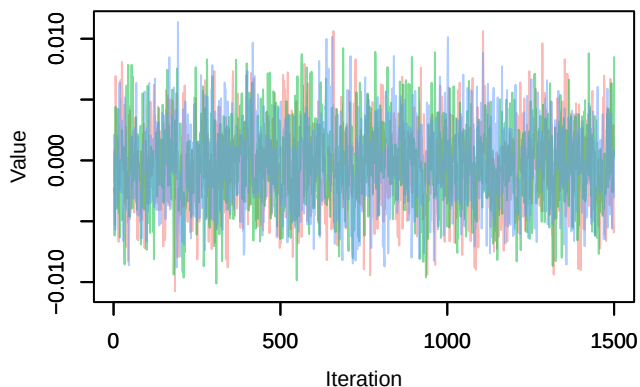
Trace – B[chelsea_pr (C3), sp_38 (S38)]
