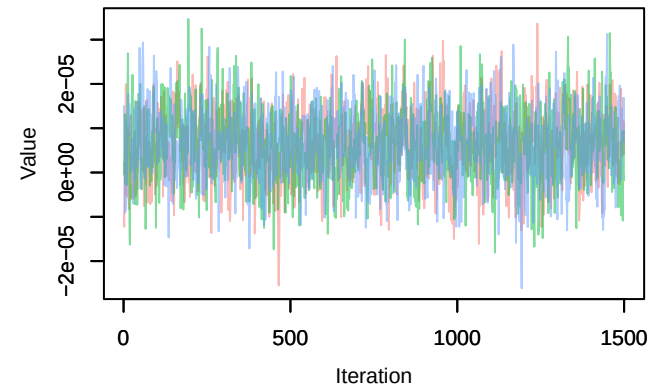
Trace – B[distance.to.pastures (C10), sp_24 (S24
