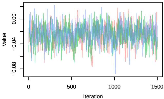
Trace – B[light_pollution (C6), sp_31 (S31)]
