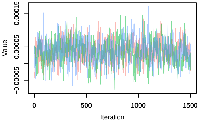
Trace – B[distance.to.pastures (C10), sp_8 (S8)]
