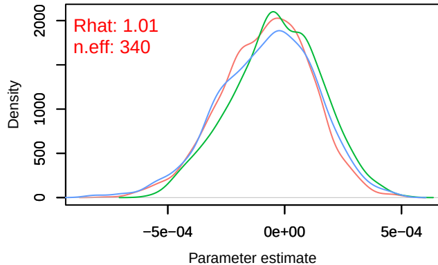
Density – B[(Intercept) (C1), sp_3 (S3)]
