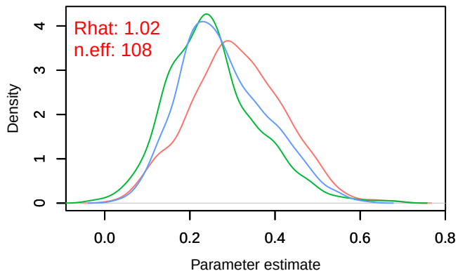
Density – B[chelsa_hurs (C2), sp_15 (S15)]
