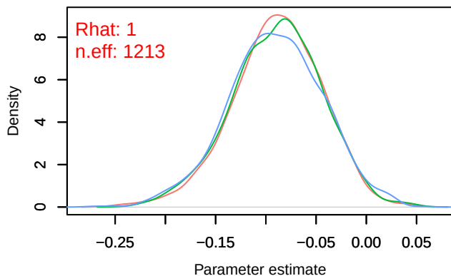
Density – B[chelsea_hurs (C2), sp_38 (S38)]
