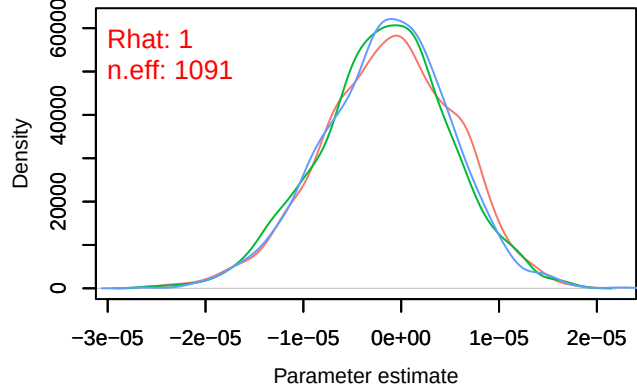
– B[distance.to.forest.and.semi.natural.areas (C13), y – B[distance.to.forest.and.semi.natural.areas (C13), y]
