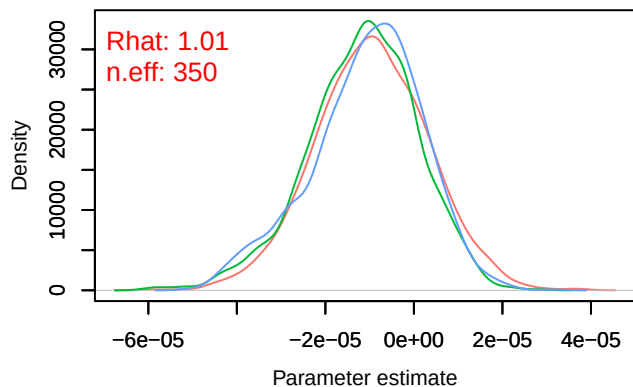
Density – B[distance.to.pastures (C10), sp_15 (S1
