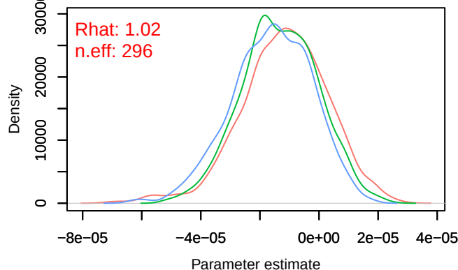
Trace – B[distance.to.permanent.crops (C9), sp_16 (Density – B[distance.to.permanent.crops (C9), sp_16
