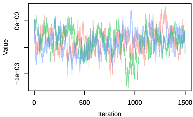
Trace – B[distance.to.arable.land (C8), sp_15 (S1
