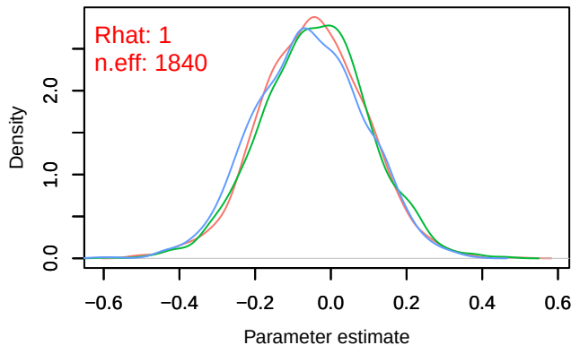
Density – B[ndvi (C5), sp_37 (S37)]
