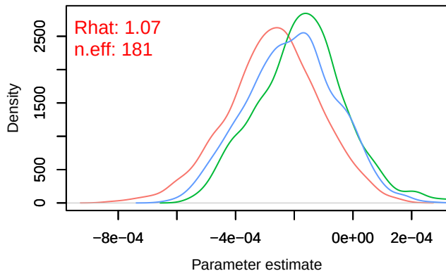
Density – B[distance.to.wetlants (C12), sp_16 (S16]
