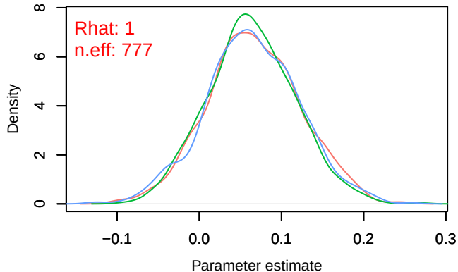
Density – B[chelsea_hurs (C2), sp_18 (S18)]
