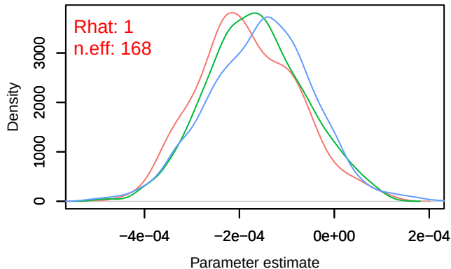
Density – B[distance.to.wetlants (C12), sp_16 (S16]
