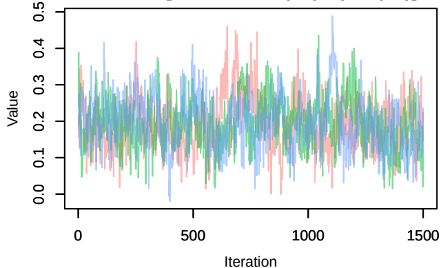
Trace – B[chelsa_pr (C3), sp_8 (S8)]
