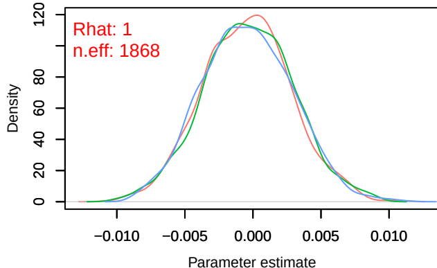
Density – B[chelsea_pr (C3), sp_38 (S38)]
