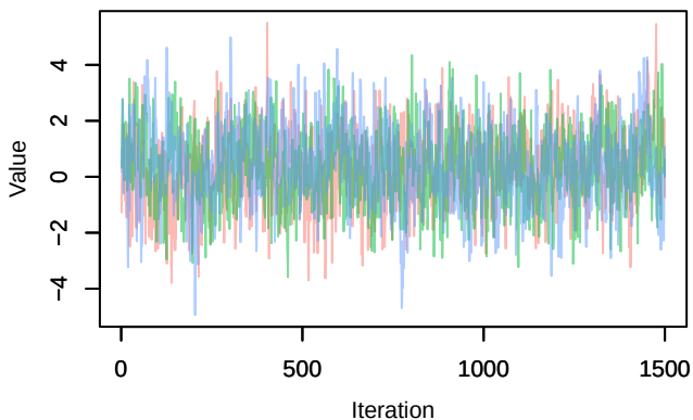
Trace – B[ndvi (C5), sp_31 (S31)]
