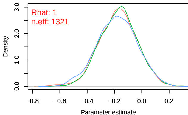
Density – B[chelsea_tas (C4), sp_38 (S38)]
