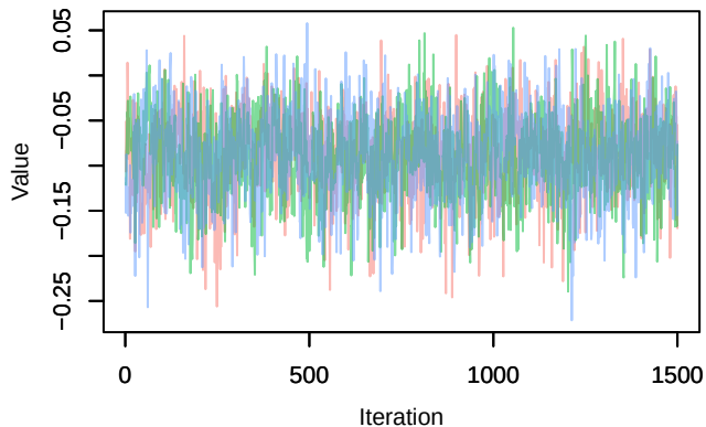
Trace – B[chelsea_hurs (C2), sp_38 (S38)]
