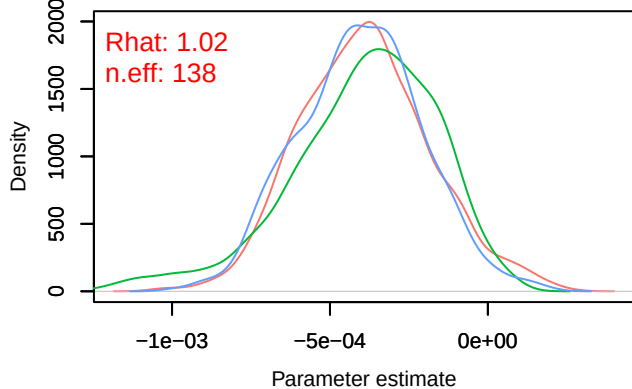
Density – B[distance.to.arable.land (C8), sp_15 (S1
