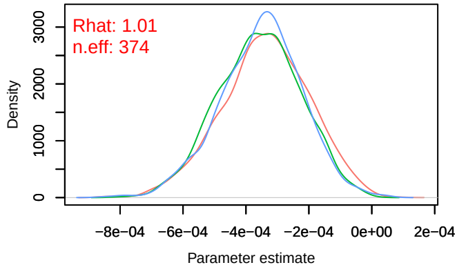
Density – B[distance.to.permanent.crops (C9), sp_8 (S8)]
