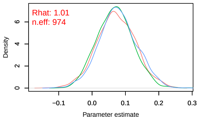
Density – B[chelsea_hurs (C2), sp_25 (S25)]
