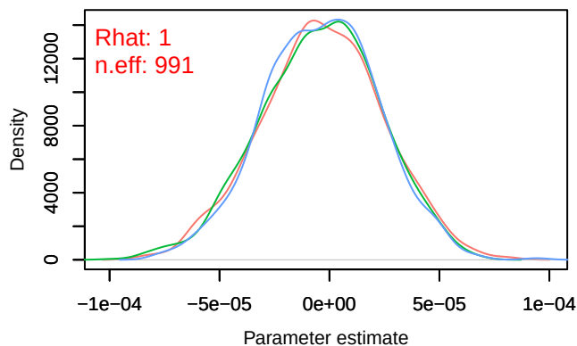
Density – B[distance.to.pastures (C10), sp_24 (S24
