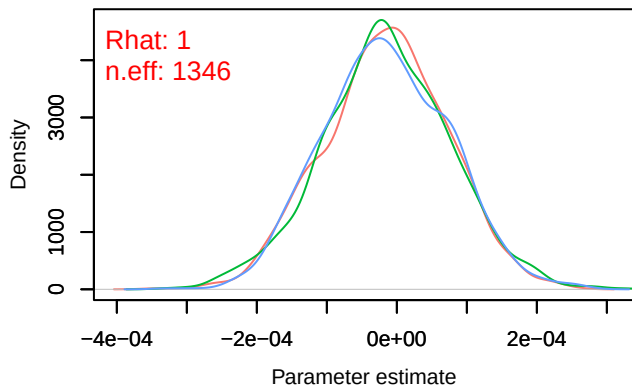
Trace – B[distance.to.arable.land (C8), sp_21 (S2: Density – B[distance.to.arable.land (C8), sp_21 (S2
