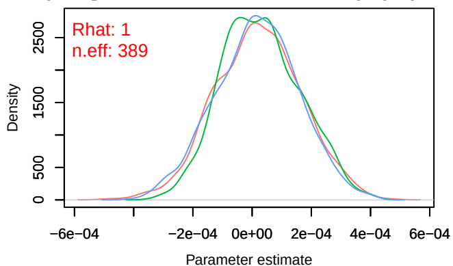
Trace – B[distance.to.artificial.surfaces (C7), sp_15 (Density – B[distance.to.artificial.surfaces (C7), sp_15
