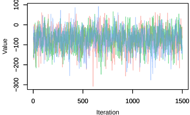
Trace – B[(Intercept) (C1), sp_12 (S12)]
