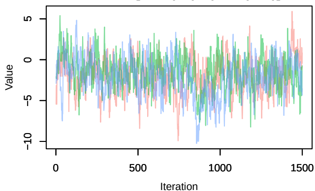
Trace – B[ndvi (C5), sp_22 (S22)]
