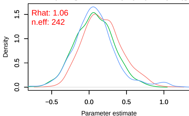
Density – B[chelsea_tas (C4), sp_22 (S22)]
