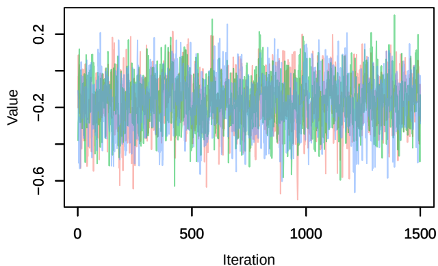
Trace – B[chelsea_tas (C4), sp_38 (S38)]
