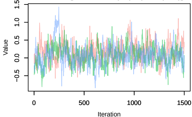
Trace – B[chelsea_tas (C4), sp_22 (S22)]
