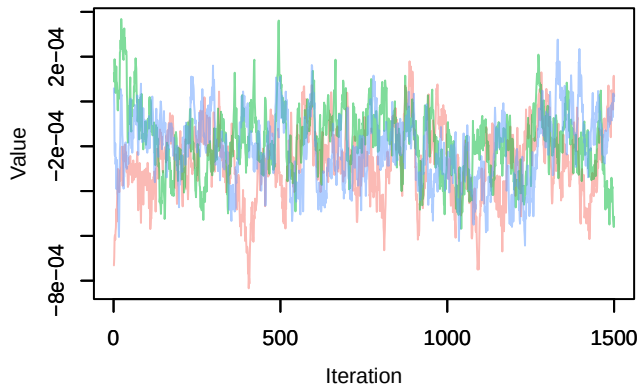
Trace – B[distance.to.wetlants (C12), sp_16 (S16]
