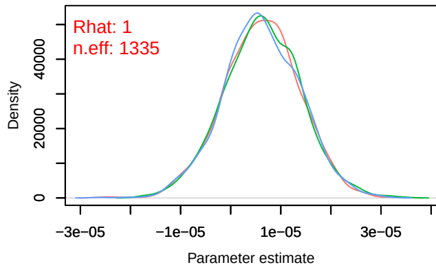
Density – B[distance.to.pastures (C10), sp_24 (S24
