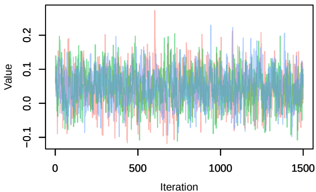
Trace – B[chelsa_hurs (C2), sp_12 (S12)]
