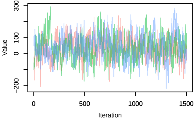
Trace – B[(Intercept) (C1), sp_15 (S15)]
