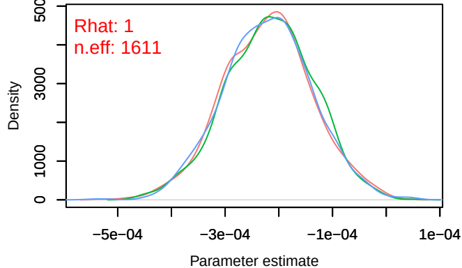
Density – B[distance.to.arable.land (C8), sp_7 (S7)
