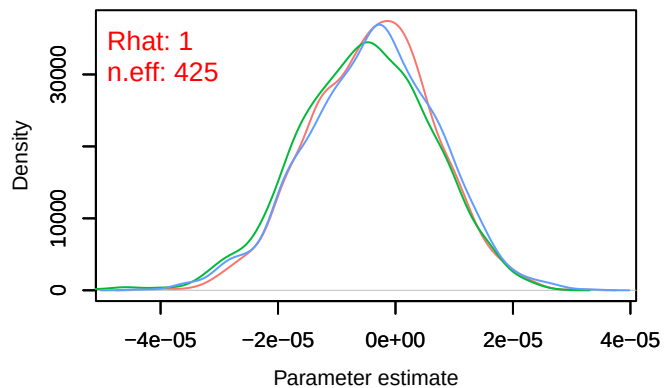
Density – B[distance.to.pastures (C10), sp_36 (S36
