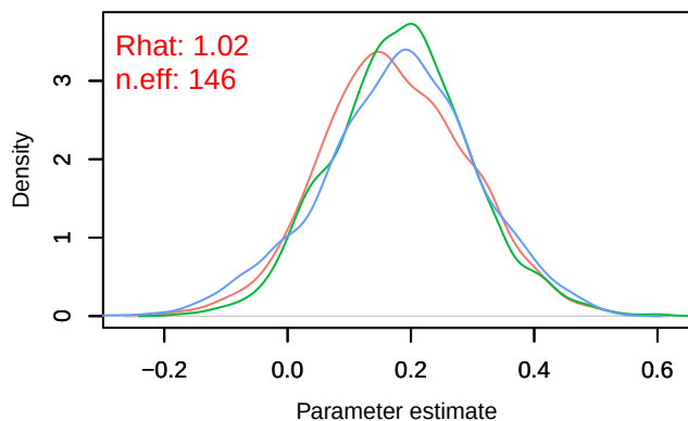
Density – B[chelsea_hurs (C2), sp_15 (S15)]
