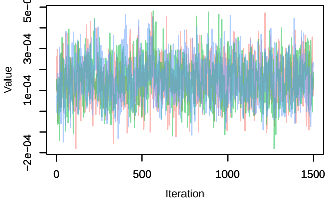
Trace – B[distance.to.water.bodies (C14), sp_14 (S14)]
