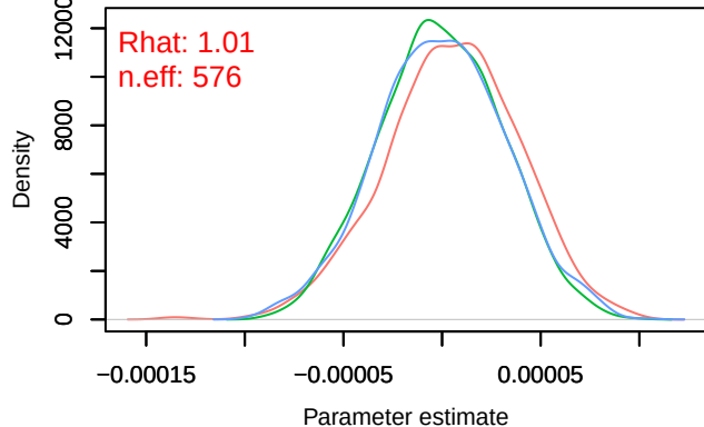
Density – B[distance.to.pastures (C10), sp_23 (S2
