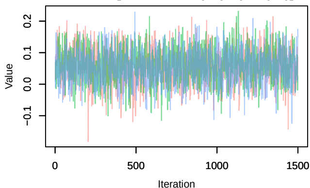
Trace – B[chelsa_hurs (C2), sp_7 (S7)]
