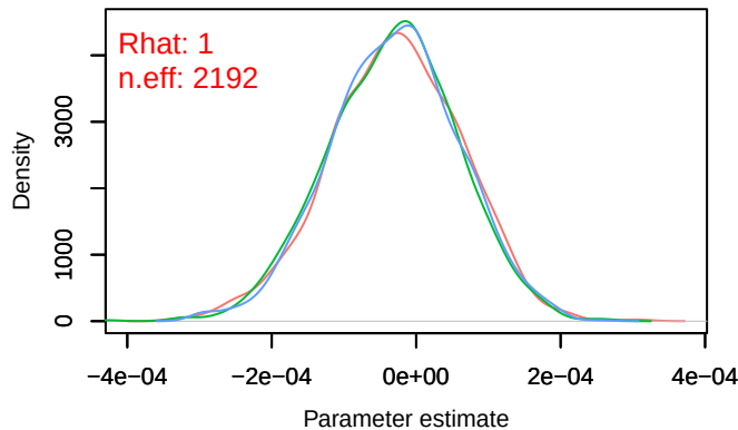
Density – B[(Intercept) (C1), sp_36 (S36)]
