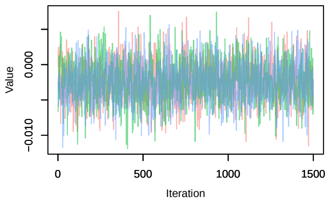
Trace – B[chelsa_pr (C3), sp_7 (S7)]
