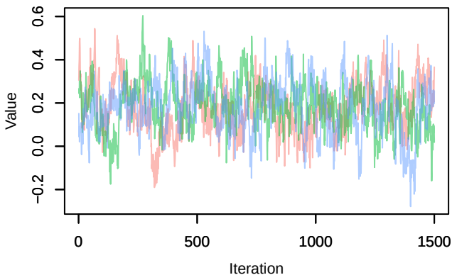
Trace – B[chelsea_hurs (C2), sp_15 (S15)]
