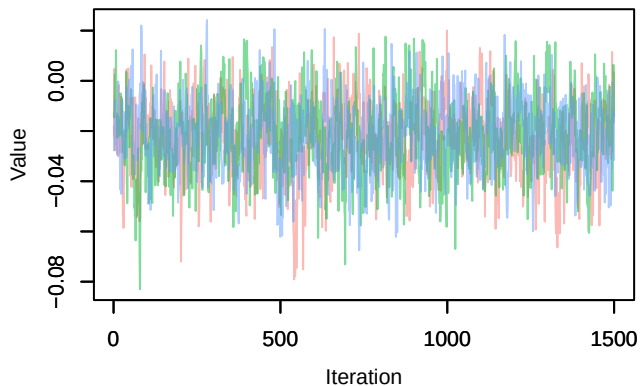
Trace – B[light_pollution (C6), sp_19 (S19)]
