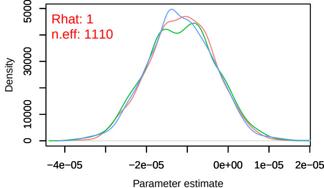
Density – B[distance.to.pastures (C10), sp_32 (S32)
