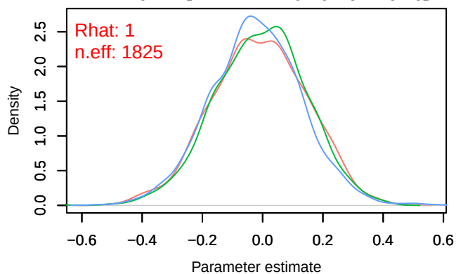
Density – B[ndvi (C5), sp_7 (S7)]
