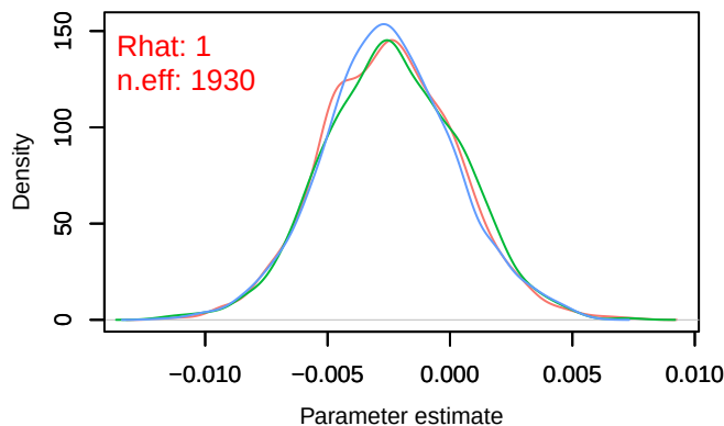
Density – B[chelsa_pr (C3), sp_7 (S7)]
