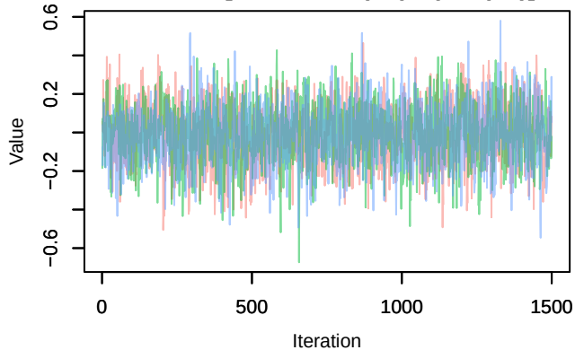
Trace – B[ndvi (C5), sp_7 (S7)]
