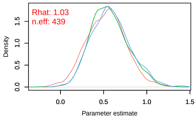
Density – B[chelsa_tas (C4), sp_1 (S1)]
