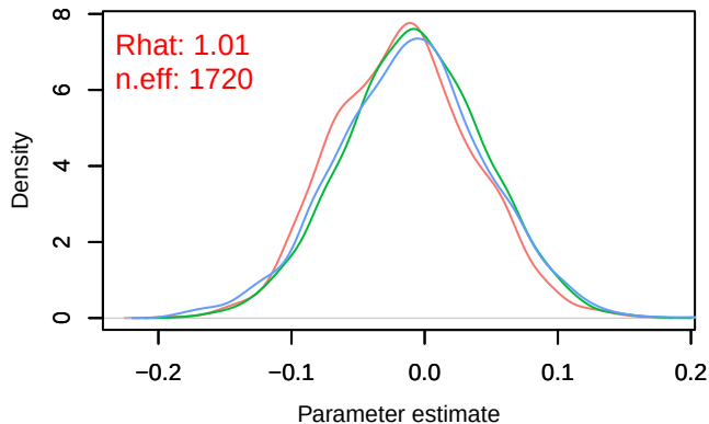
Density – B[chelsea_hurs (C2), sp_35 (S35)]
