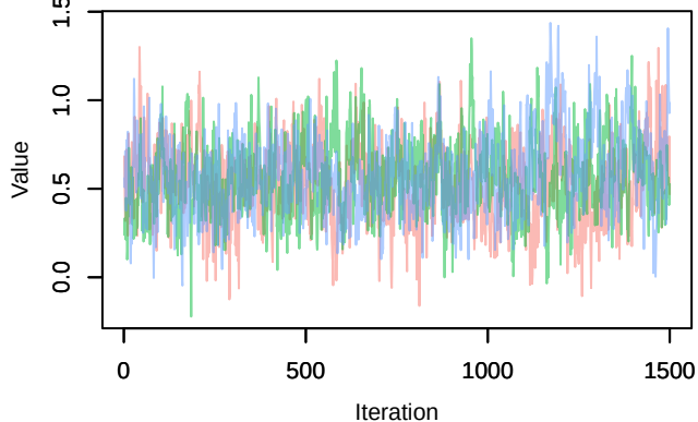
Trace – B[chelsa_tas (C4), sp_1 (S1)]
