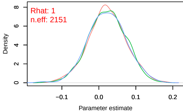
Density – B[chelsea_pr (C3), sp_14 (S14)]
