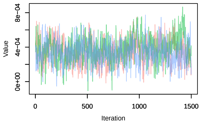
Trace – B[distance.to.water.bodies (C14), sp_3 (S3)]
