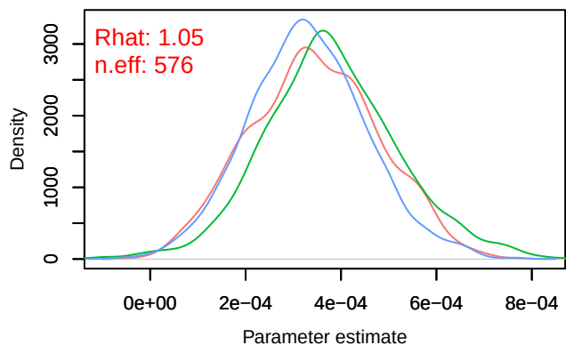
Density – B[distance.to.water.bodies (C14), sp_3 (S3)]
