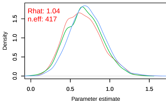
Density – B[chelsea_tas (C4), sp_6 (S6)]
