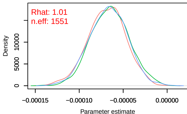
Density – B[distance.to.pastures (C10), sp_9 (S9)
