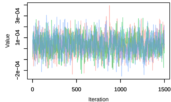
Trace – B[distance.to.arable.land (C8), sp_34 (S3 Density – B[distance.to.arable.land (C8), sp_34 (S3
