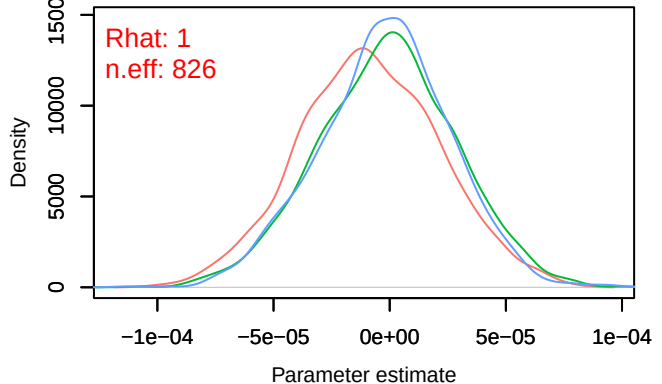
Density – B[distance.to.pastures (C10), sp_26 (S26)]
