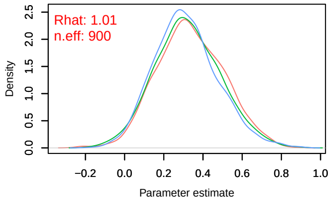
Density – B[ndvi (C5), sp_27 (S27)]
