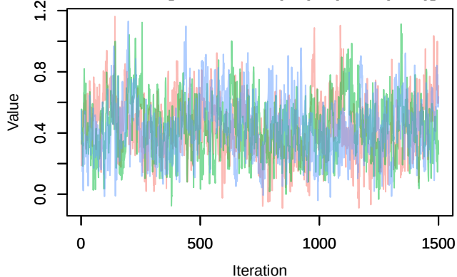
Trace – B[chelsea_tas (C4), sp_31 (S31)]
