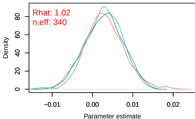
Density – B[chelsea_pr (C3), sp_33 (S33)]
