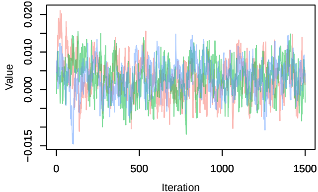
Trace – B[chelsea_pr (C3), sp_33 (S33)]
