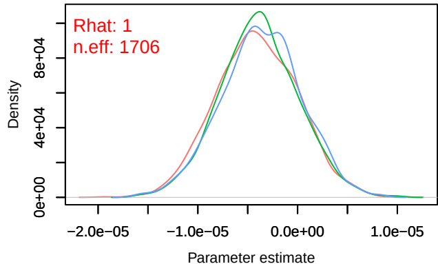
Density – B[distance.to.permanent.crops (C9), sp_7 (
