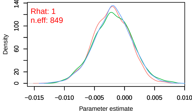
Density – B[chelsa_tas (C4), sp_8 (S8)]
