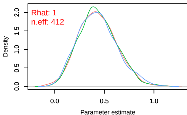
Density – B[chelsea_tas (C4), sp_31 (S31)]
