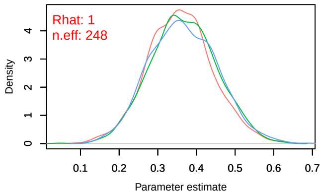
Density – B[chelsa_hurs (C2), sp_18 (S18)]
