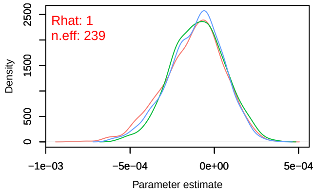
Density – B[distance.to.arable.land (C8), sp_33 (S3
