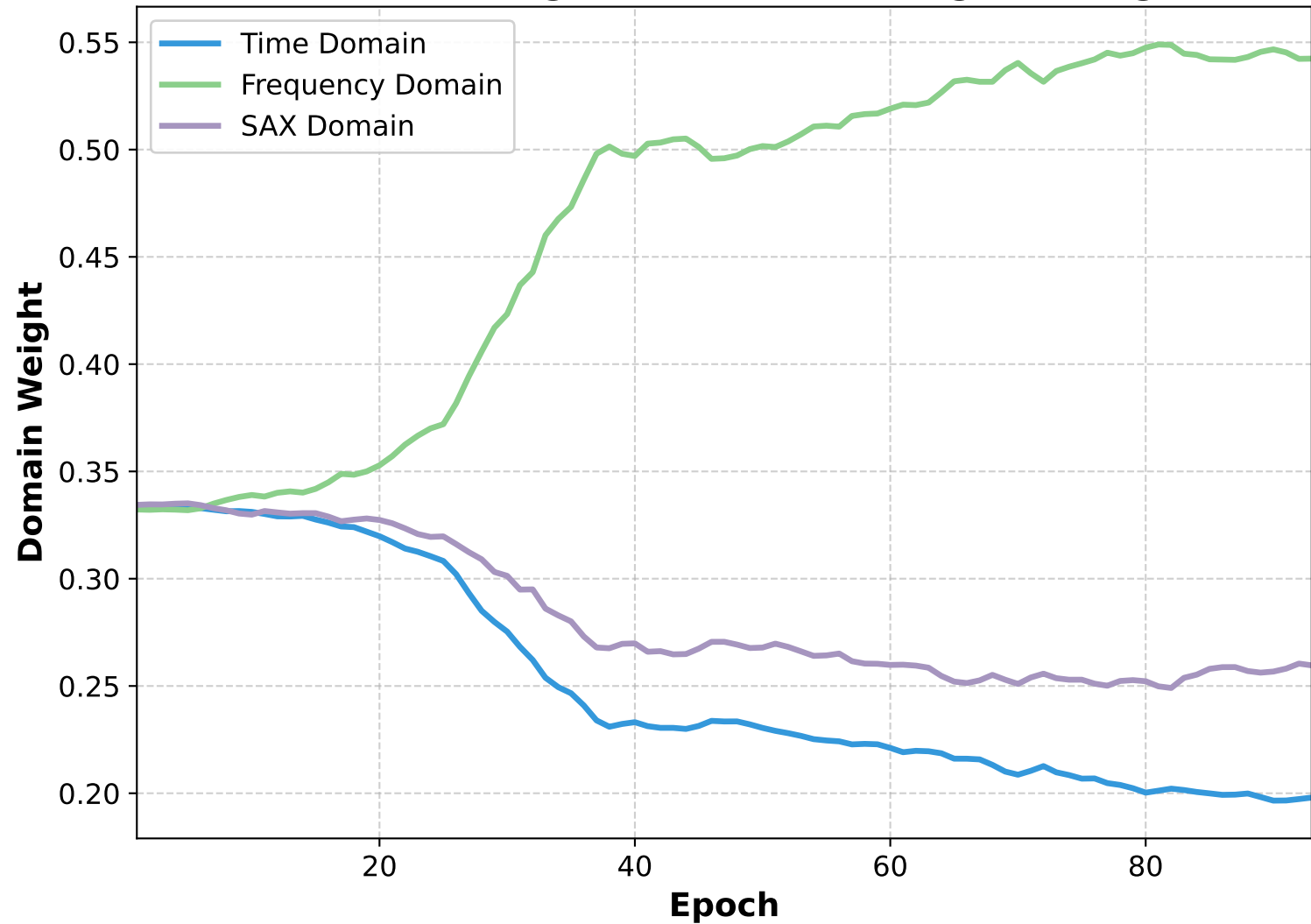
Domain Weight Evolution during Training
