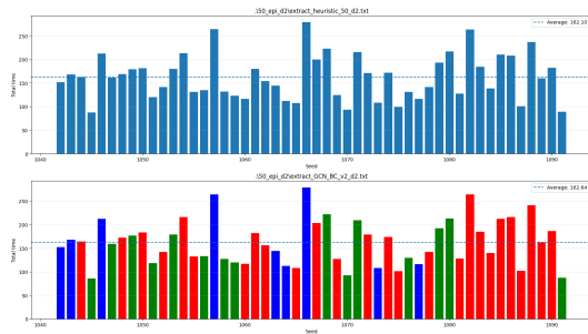
Fig. 7: Comparison between heuristic scheduling and the proposed GCN scheduler on denser D2 environments.
