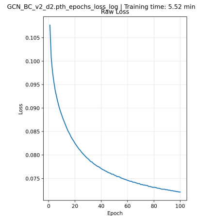
Fig. 2: Raw training loss evolution of the proposed GCN scheduler on the denser D2 environment.
