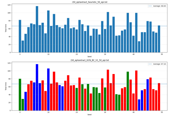
Fig. 4: Comparison between heuristic scheduling and the proposed GCN scheduler on known D1 environments.
