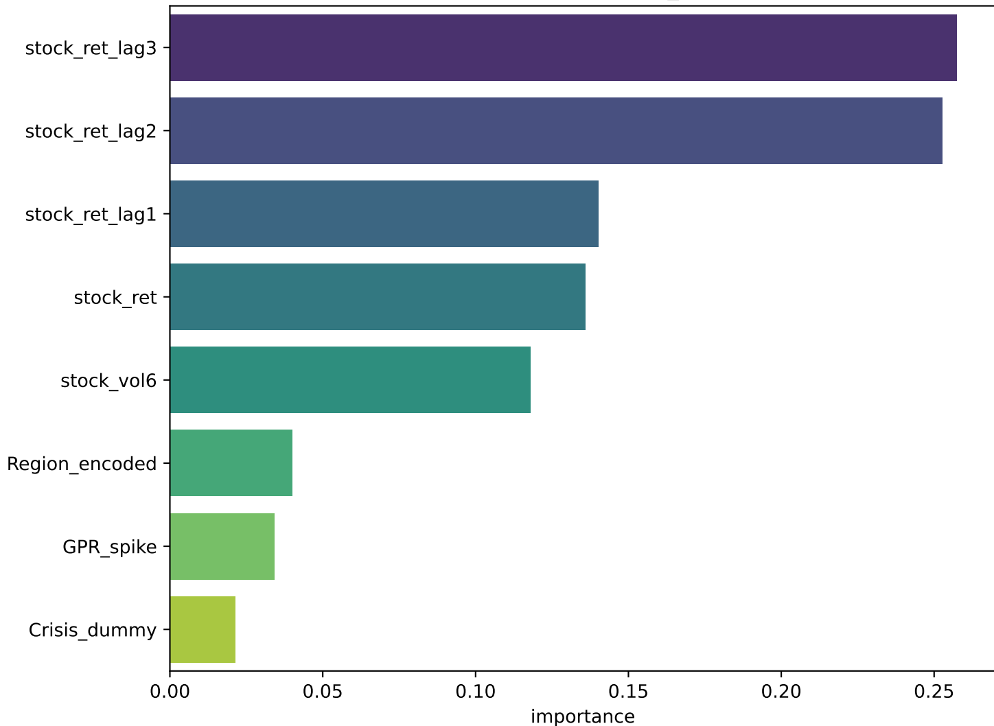
Feature Importances direction_B (full period)
