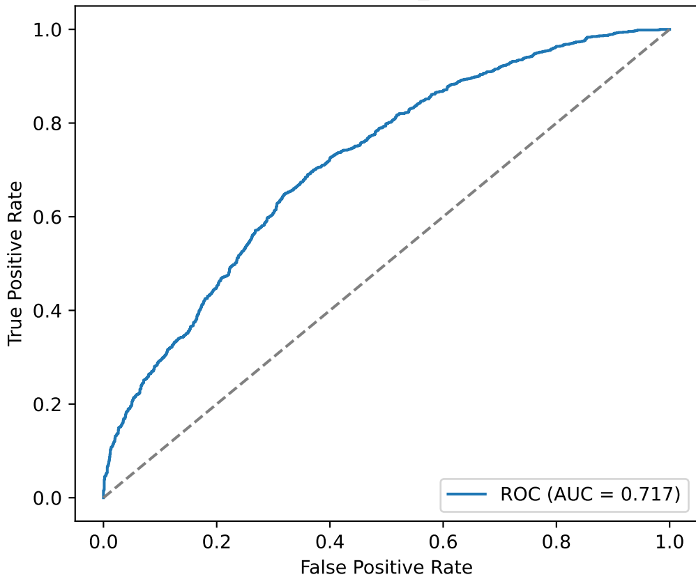
ROC Curve direction_B (full period)
