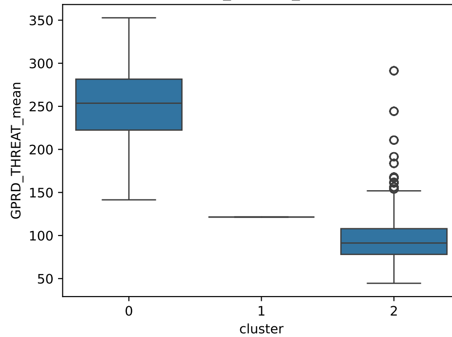
GPRD_THREAT_mean
