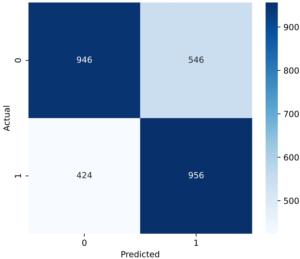
Confusion Matrix direction_B (full period)
